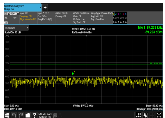
Band4-10MHz-QPSK-20000-1RB#49-0.009~0.15-PASS
