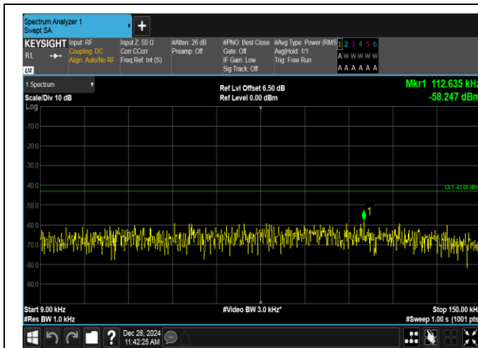
Band4-5MHz-QPSK-20375-1RB#0-0.009~0.15-PASS
