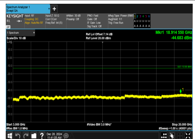
Band4-5MHz-QPSK-20175-25RB#0-3000~20000-PASS
