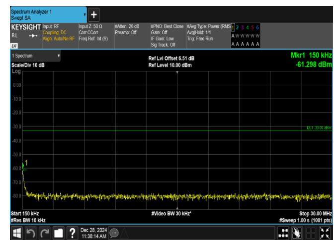
Band4-5MHz-QPSK-20175-1RB#24-0.15~30-PASS
