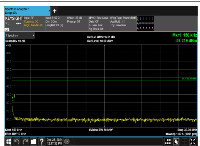
Band4-10MHz-QPSK-20000-1RB#0-0.15~30-PASS
