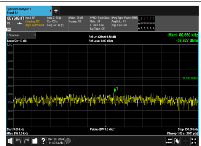
Band4-5MHz-QPSK-20175-25RB#0-0.009~0.15-PASS
