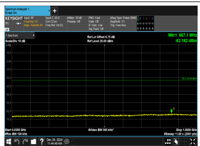
Band4-5MHz-QPSK-20375-1RB#24-30~1000-PASS
