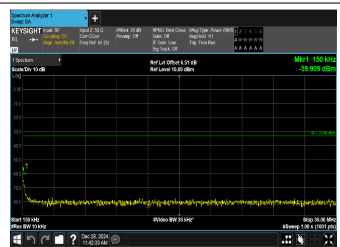
Band4-5MHz-QPSK-20375-1RB#0-0.15~30-PASS
