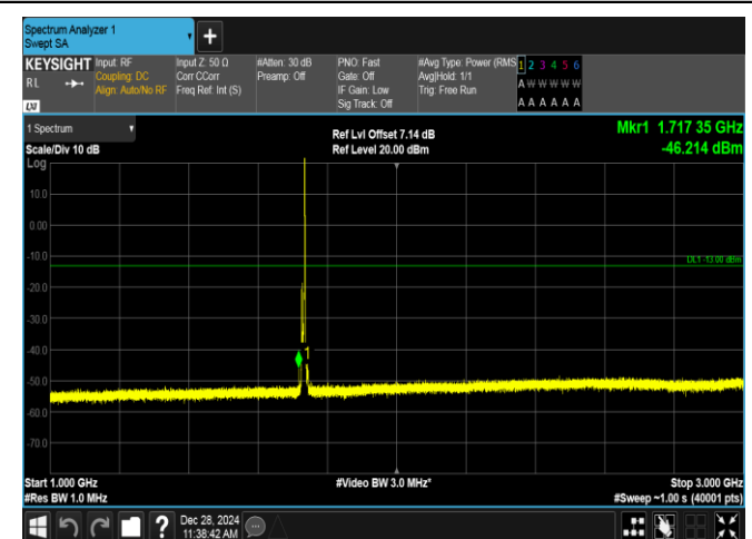
Band4-5MHz-QPSK-20175-1RB#24-1000~3000-PASS
