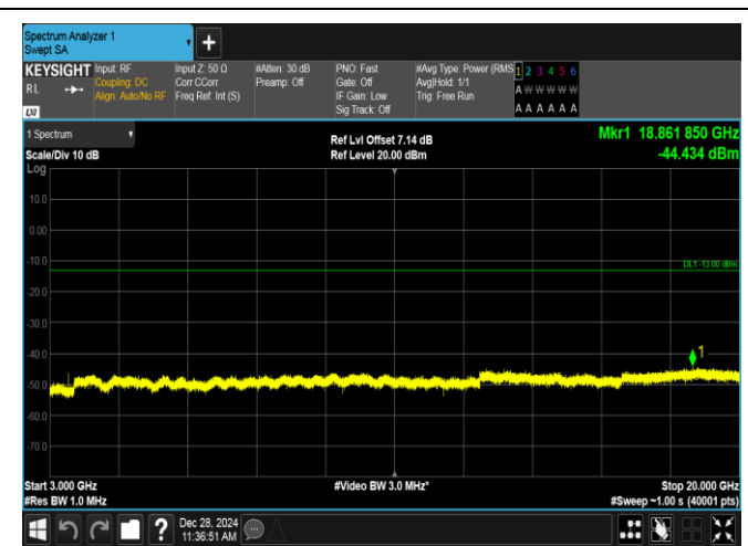
Band4-5MHz-QPSK-20175-1RB#0-3000~20000-PASS
