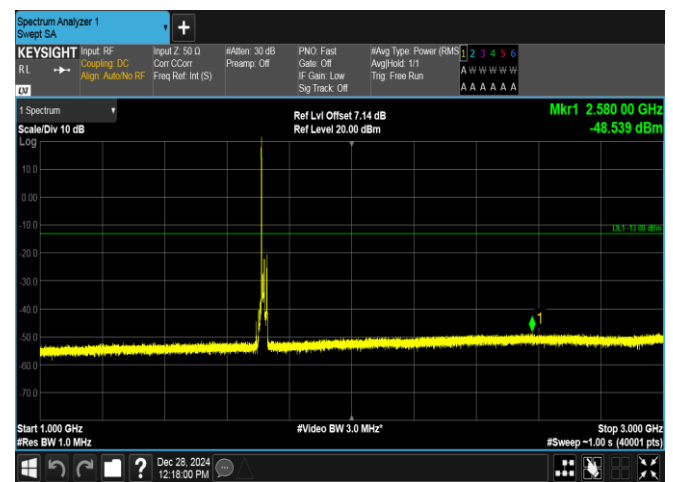
Band4-10MHz-QPSK-20000-1RB#0-1000~3000-PASS
