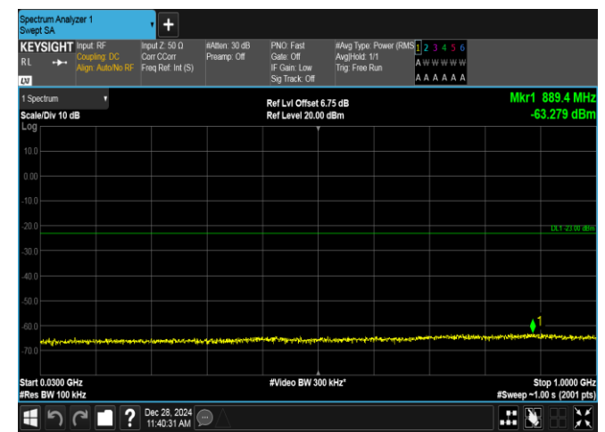
Band4-5MHz-QPSK-20175-25RB#0-30~1000-PASS
