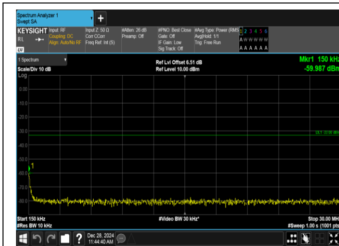
Band4-5MHz-QPSK-20375-1RB#24-0.15~30-PASS
