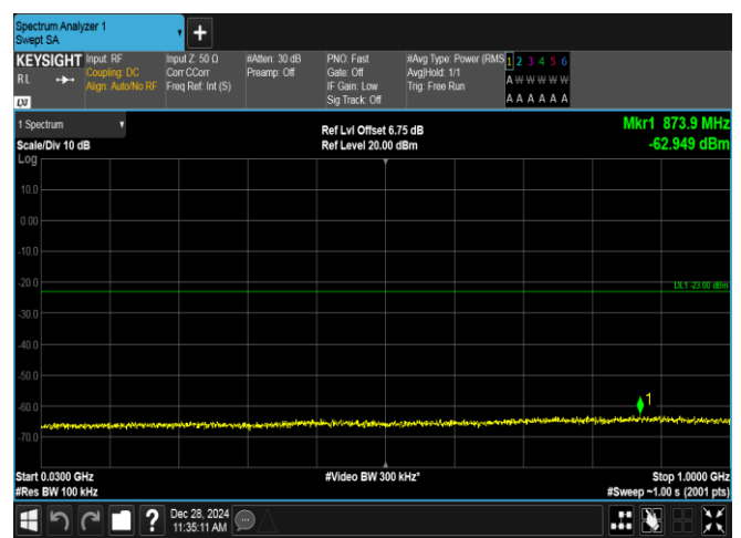
Band4-5MHz-16QAM-19975-25RB#0-30~1000-PASS
