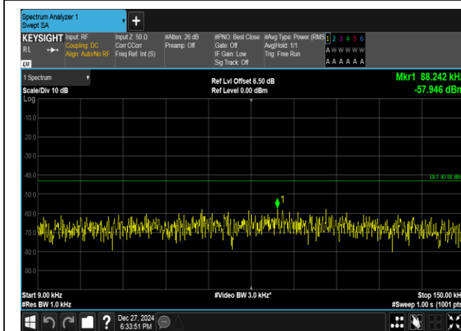
Band2-10MHz-16QAM-18900-50RB#0-0.009~0.15-PASS
