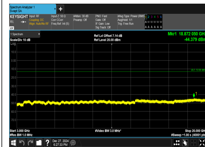
Band2-10MHz-QPSK-18650-50RB#0-3000~20000-PASS
