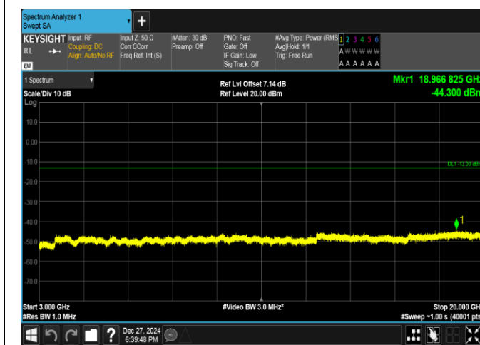
Band2-10MHz-QPSK-19150-50RB#0-3000~20000-PASS
