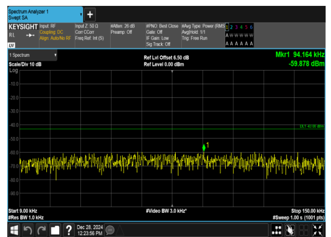
Band4-10MHz-QPSK-20175-1RB#0-0.009~0.15-PASS
