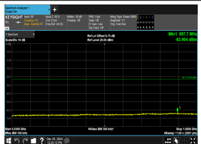
Band4-10MHz-QPSK-20175-1RB#0-30~1000-PASS
