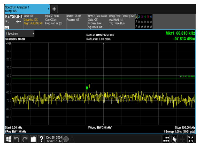
Band4-10MHz-QPSK-20350-1RB#49-0.009~0.15-PASS
