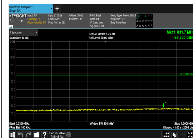
Band2-15MHz-QPSK-18900-1RB#74-30~1000-PASS
