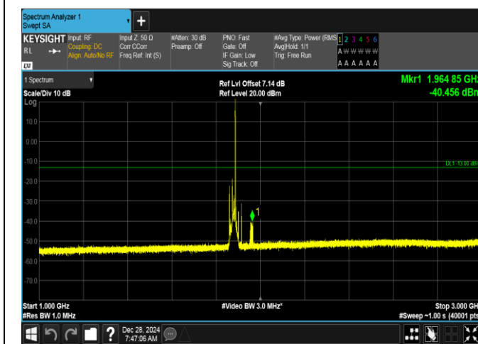
Band2-15MHz-16QAM-18900-1RB#74-1000~3000-PASS
