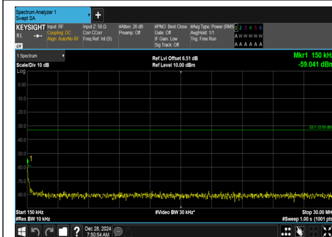
Band2-15MHz-16QAM-19125-1RB#0-0.15~30-PASS
