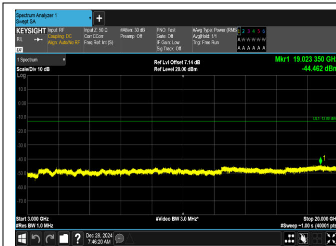
Band2-15MHz-QPSK-18900-1RB#74-3000~20000-PASS
