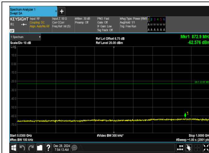
Band2-15MHz-QPSK-19125-75RB#0-30~1000-PASS
