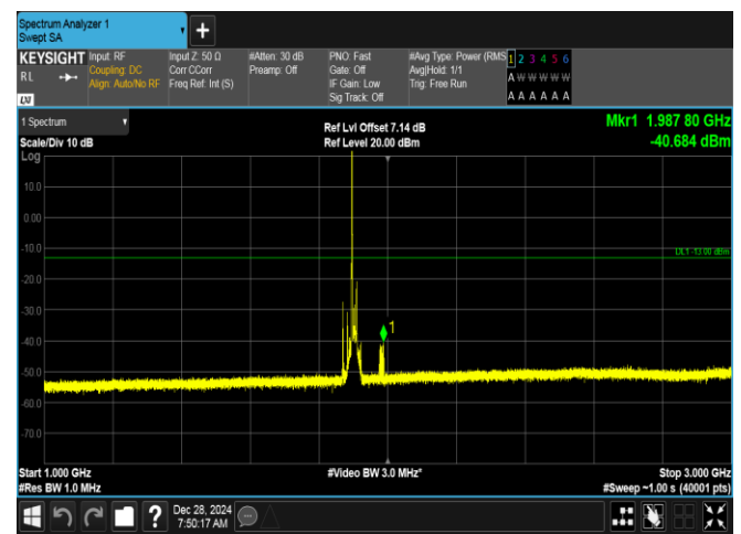
Band2-15MHz-QPSK-19125-1RB#0-1000~3000-PASS
