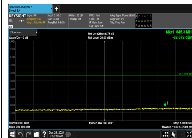
Band2-15MHz-16QAM-19125-1RB#74-30~1000-PASS
