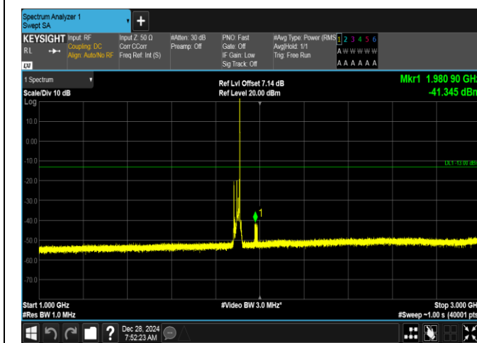
Band2-15MHz-QPSK-19125-1RB#74-1000~3000-PASS
