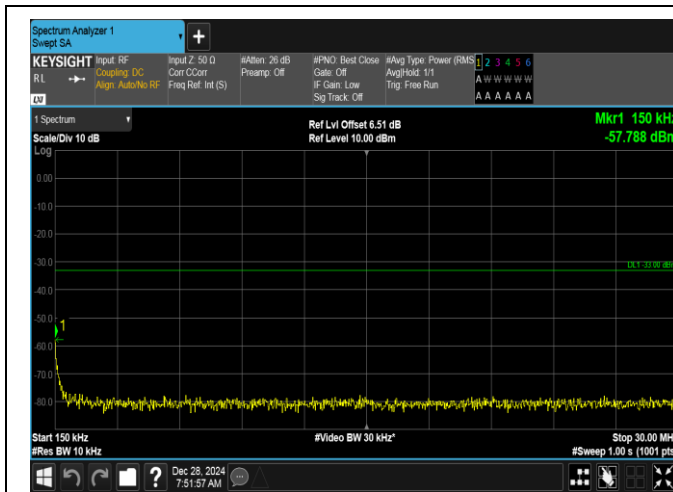
Band2-15MHz-QPSK-19125-1RB#74-0.15~30-PASS
