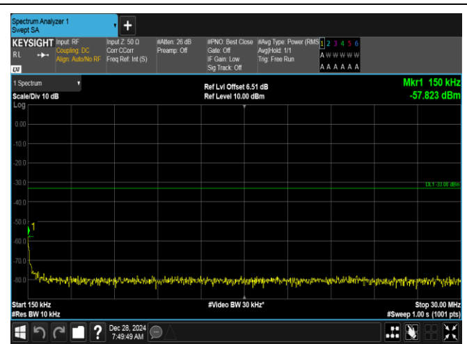
Band2-15MHz-QPSK-19125-1RB#0-0.15~30-PASS
