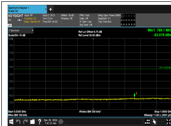
Band2-15MHz-QPSK-18675-75RB#0-30~1000-PASS
