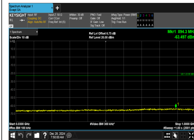
Band2-15MHz-QPSK-19125-1RB#0-30~1000-PASS
