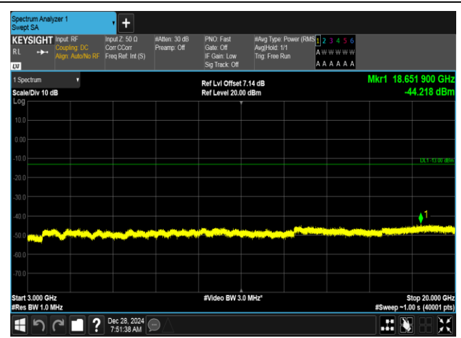
Band2-15MHz-16QAM-19125-1RB#0-3000~20000-PASS
