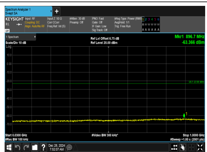
Band2-15MHz-QPSK-19125-1RB#74-30~1000-PASS
