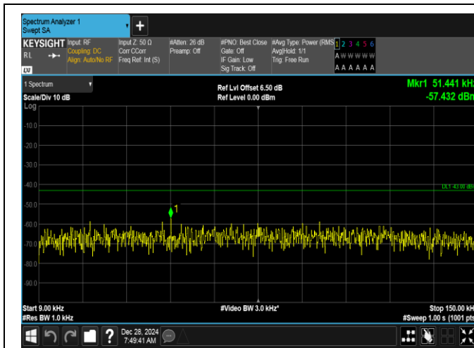
Band2-15MHz-QPSK-19125-1RB#0-0.009~0.15-PASS
