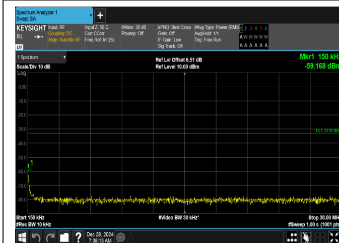
Band2-15MHz-16QAM-18675-1RB#0-0.15~30-PASS
