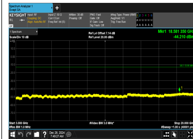
Band2-15MHz-16QAM-18900-75RB#0-3000~20000-PASS
