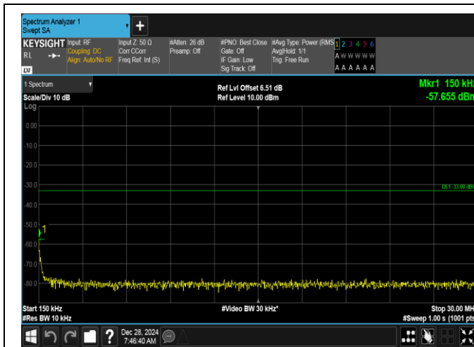
Band2-15MHz-16QAM-18900-1RB#74-0.15~30-PASS
