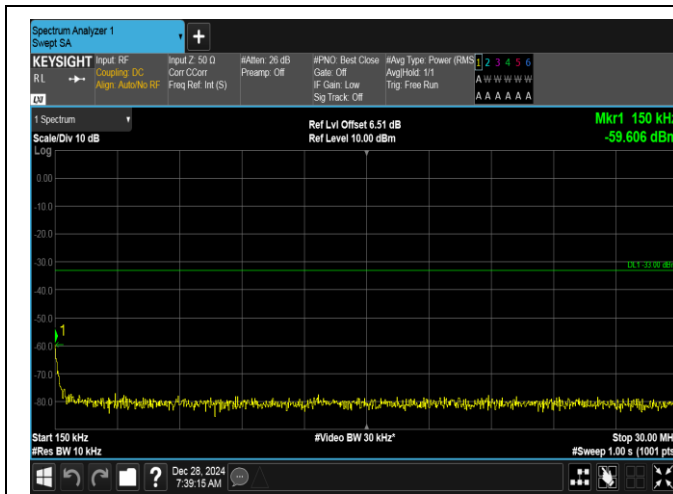
Band2-15MHz-QPSK-18675-1RB#74-0.15~30-PASS
