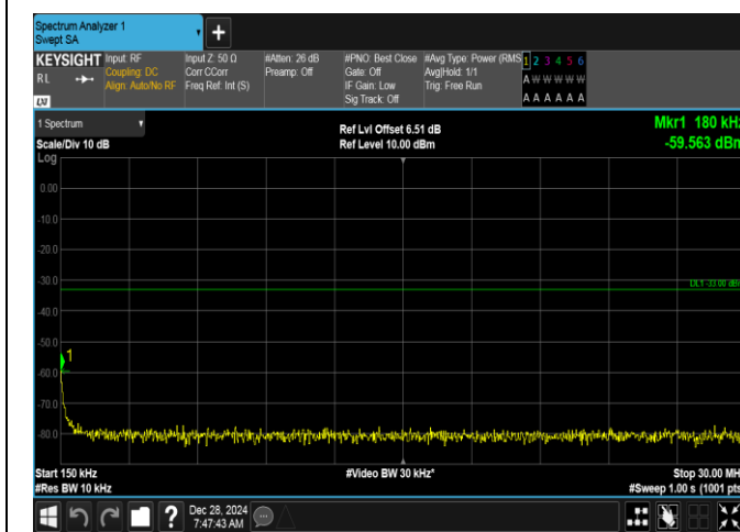
Band2-15MHz-QPSK-18900-75RB#0-0.15~30-PASS
