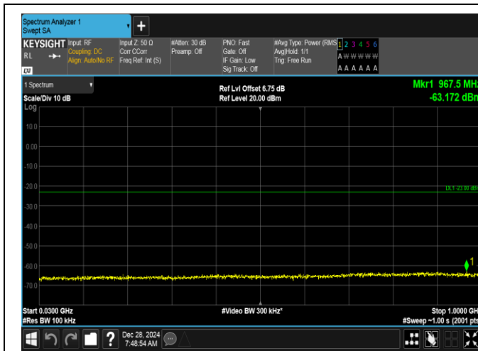
Band2-15MHz-16QAM-18900-75RB#0-30~1000-PASS
