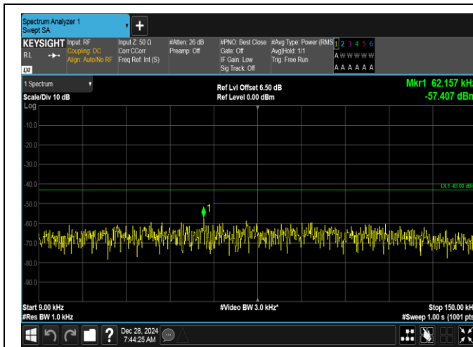
Band2-15MHz-16QAM-18900-1RB#0-0.009~0.15-PASS
