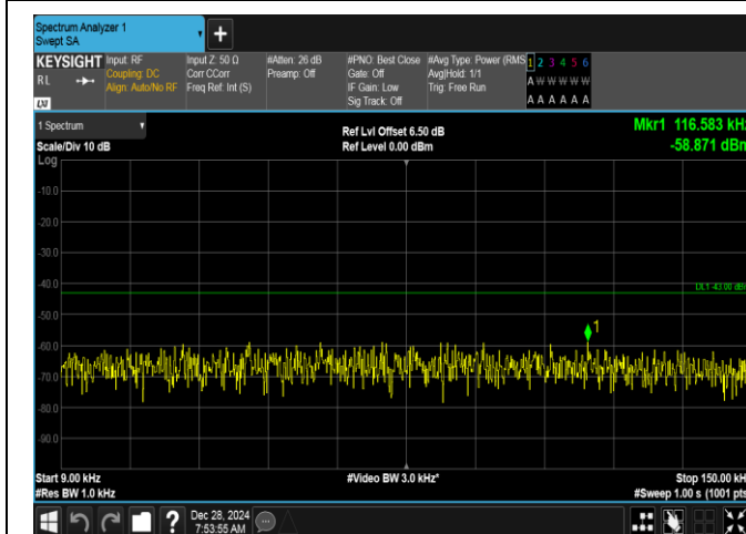
Band2-15MHz-QPSK-19125-75RB#0-0.009~0.15-PASS
