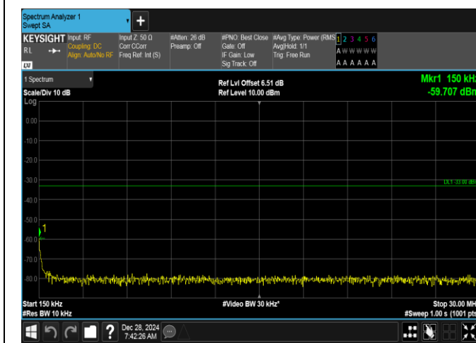
Band2-15MHz-16QAM-18675-75RB#0-0.15~30-PASS
