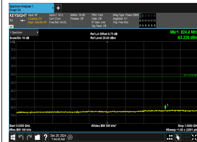
Band2-15MHz-16QAM-18900-1RB#0-30~1000-PASS
