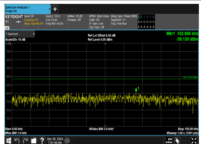
Band2-15MHz-QPSK-19125-1RB#74-0.009~0.15-PASS
