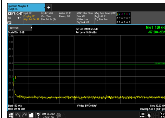
Band2-15MHz-QPSK-18900-1RB#0-0.15~30-PASS
