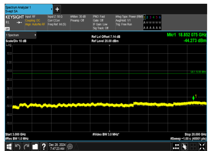
Band2-15MHz-16QAM-18900-1RB#74-3000~20000-PASS
