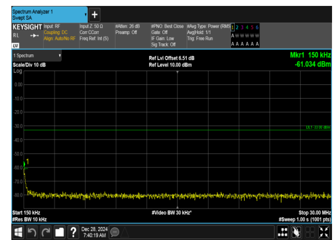
Band2-15MHz-16QAM-18675-1RB#74-0.15~30-PASS
