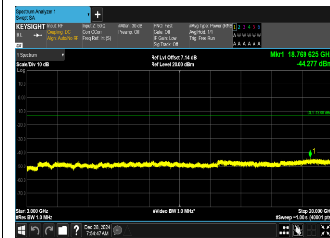
Band2-15MHz-QPSK-19125-75RB#0-3000~20000-PASS
