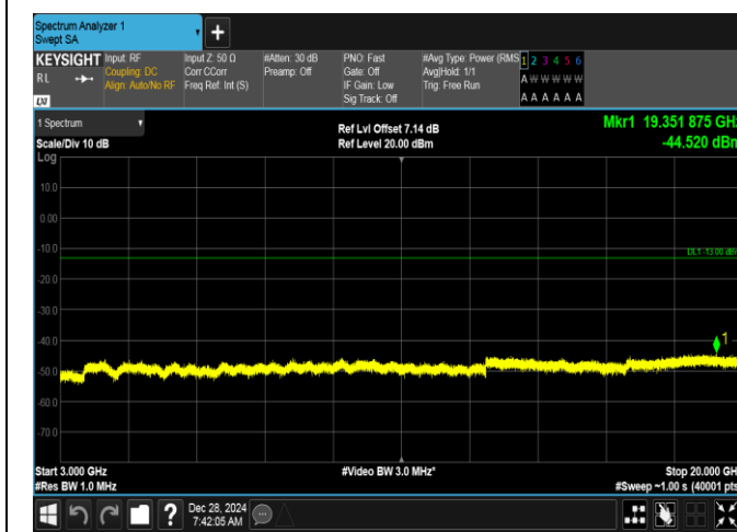
Band2-15MHz-QPSK-18675-75RB#0-3000~20000-PASS
