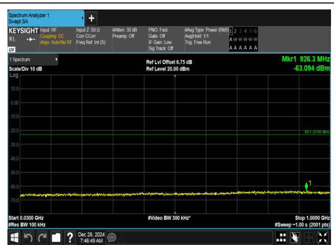
Band2-15MHz-16QAM-18900-1RB#74-30~1000-PASS
