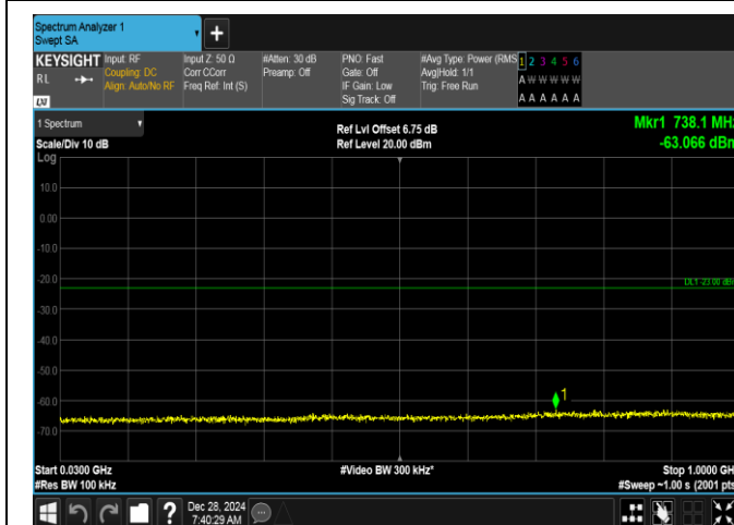
Band2-15MHz-16QAM-18675-1RB#74-30~1000-PASS
