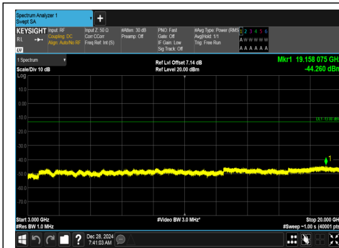
Band2-15MHz-16QAM-18675-1RB#74-3000~20000-PASS
