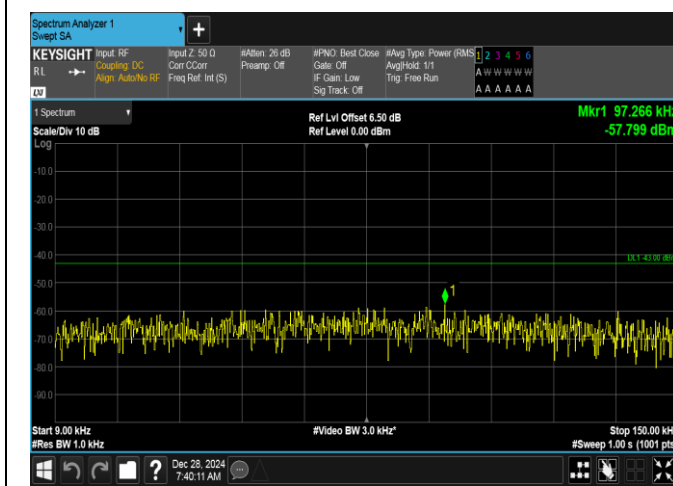
Band2-15MHz-16QAM-18675-1RB#74-0.009~0.15-PASS
