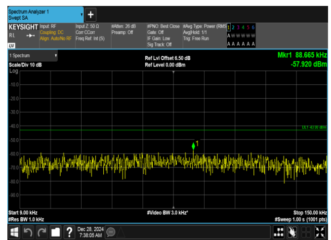
Band2-15MHz-16QAM-18675-1RB#0-0.009~0.15-PASS
