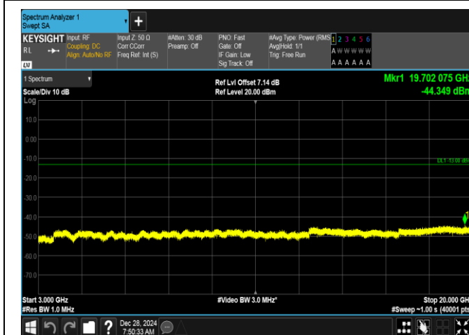
Band2-15MHz-QPSK-19125-1RB#0-3000~20000-PASS
