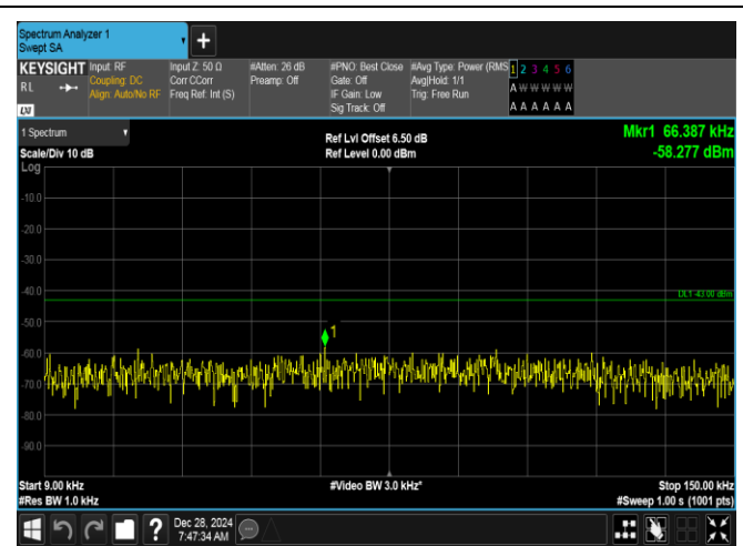
Band2-15MHz-QPSK-18900-75RB#0-0.009~0.15-PASS
