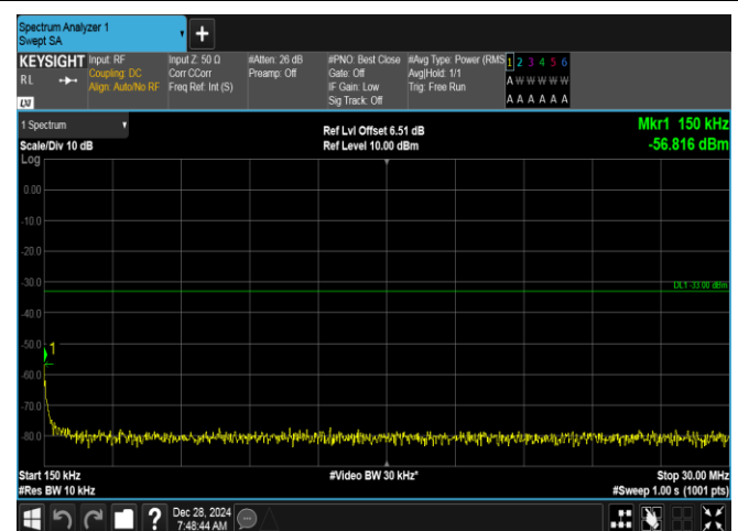
Band2-15MHz-16QAM-18900-75RB#0-0.15~30-PASS
