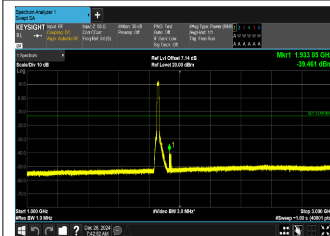
Band2-15MHz-16QAM-18675-75RB#0-1000~3000-PASS
