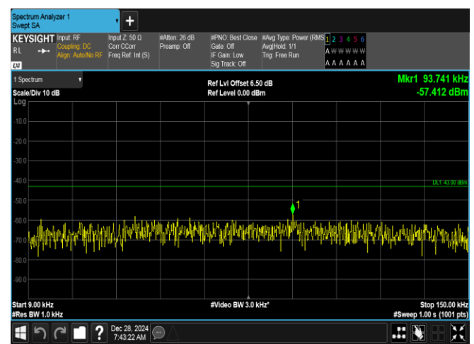
Band2-15MHz-QPSK-18900-1RB#0-0.009~0.15-PASS
