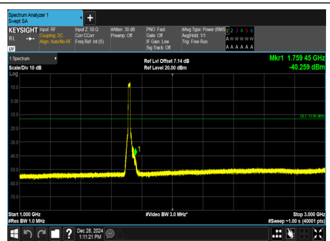
Band4-15MHz-QPSK-20025-75RB#0-1000~3000-PASS
