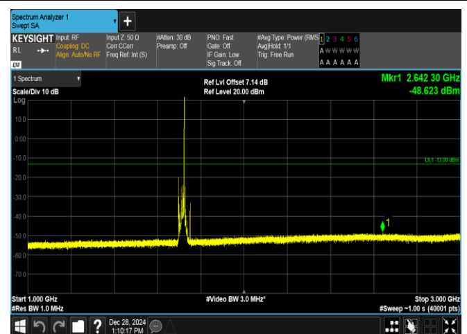
Band4-15MHz-16QAM-20025-1RB#74-1000~3000-PASS
