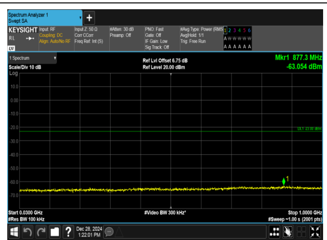
Band4-15MHz-QPSK-20325-1RB#74-30~1000-PASS
