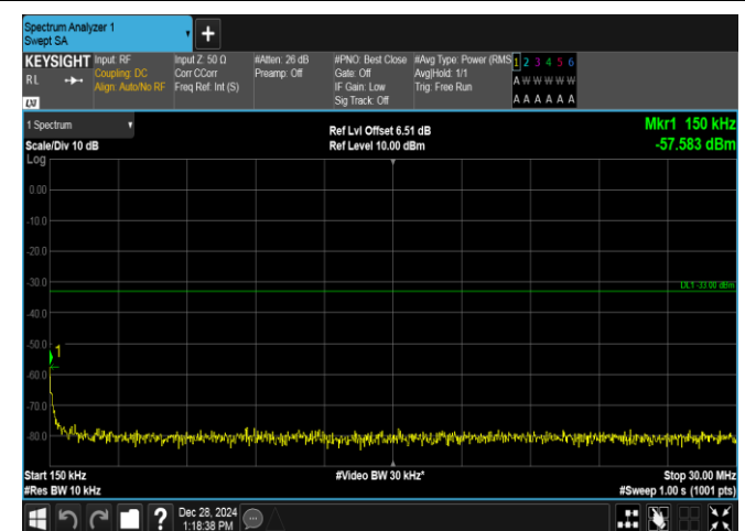
Band4-15MHz-16QAM-20175-75RB#0-0.15~30-PASS
