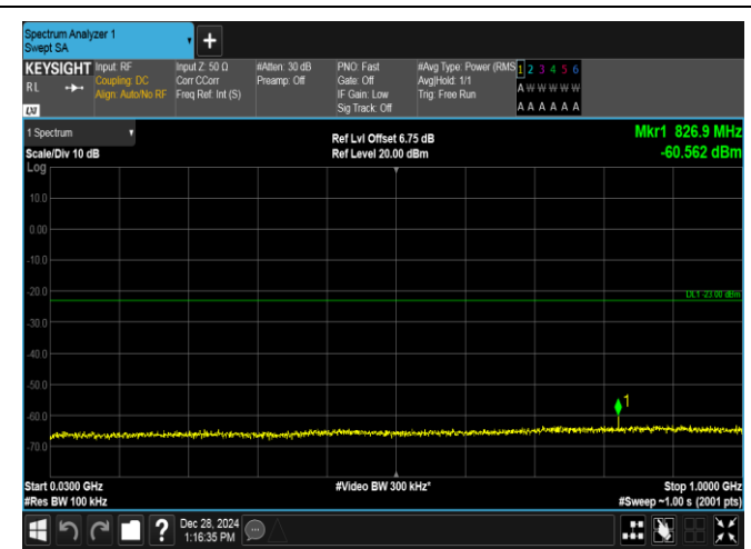
Band4-15MHz-16QAM-20175-1RB#74-30~1000-PASS
