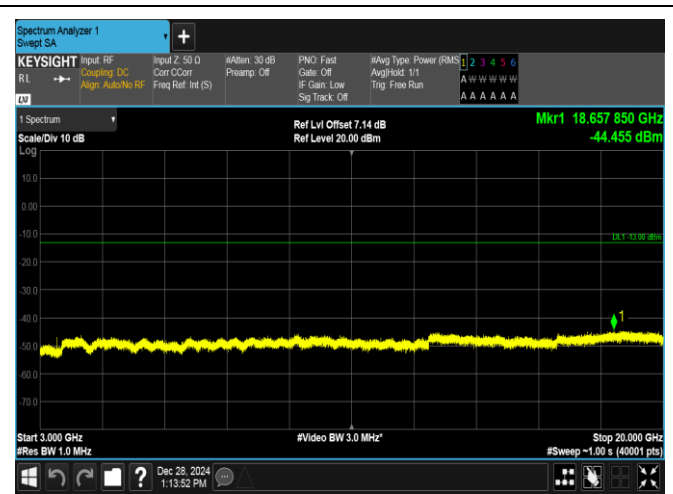
Band4-15MHz-QPSK-20175-1RB#0-3000~20000-PASS
