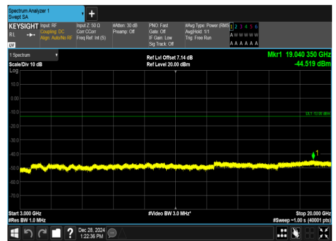
Band4-15MHz-QPSK-20325-1RB#74-3000~20000-PASS
