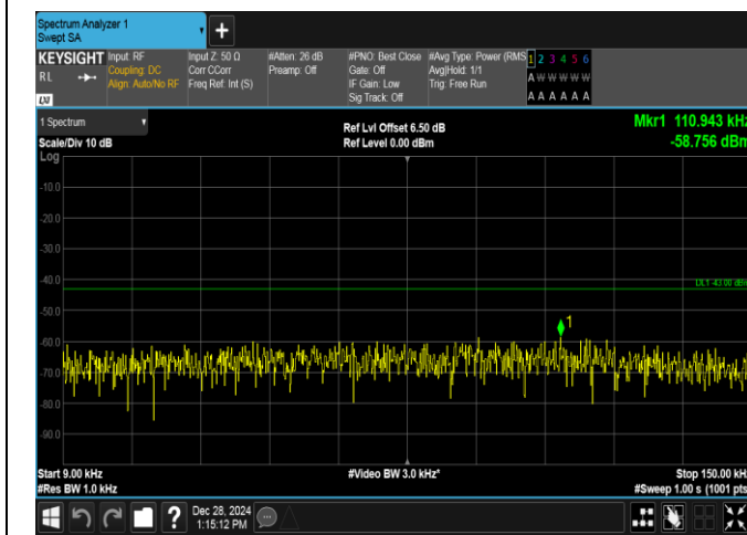
Band4-15MHz-QPSK-20175-1RB#74-0.009~0.15-PASS
