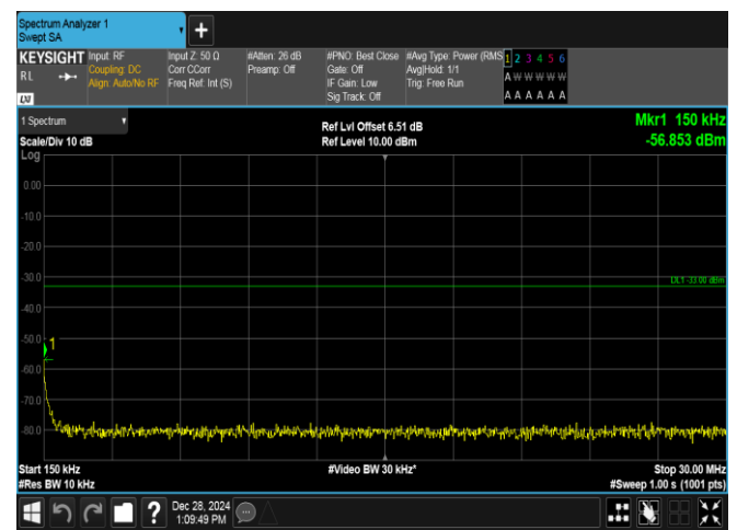
Band4-15MHz-16QAM-20025-1RB#74-0.15~30-PASS
