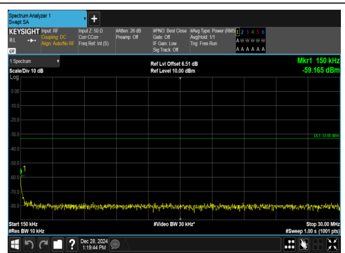
Band4-15MHz-QPSK-20325-1RB#0-0.15~30-PASS
