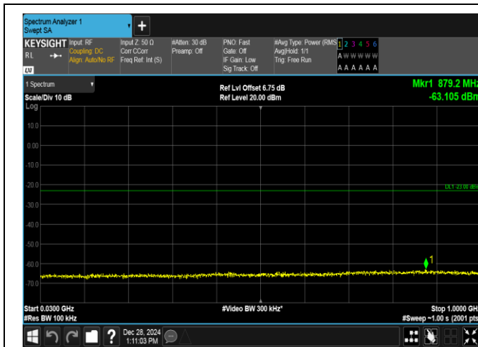
Band4-15MHz-QPSK-20025-75RB#0-30~1000-PASS
