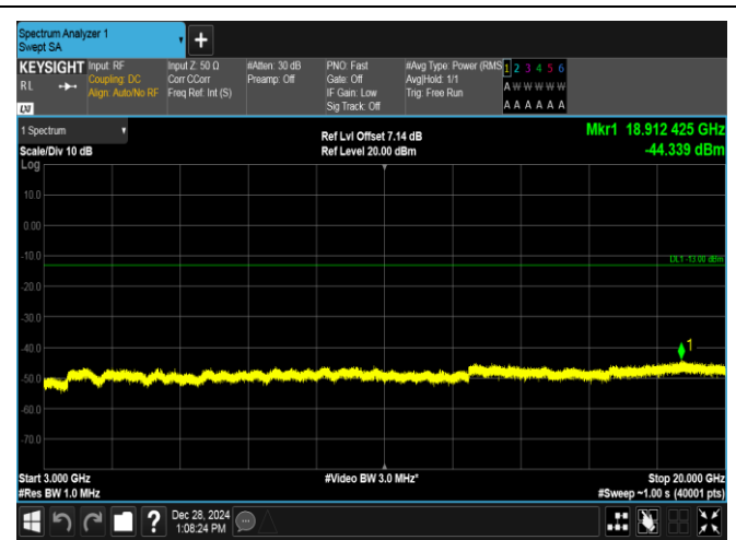
Band4-15MHz-16QAM-20025-1RB#0-3000~20000-PASS
