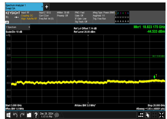
Band4-15MHz-16QAM-20175-1RB#74-3000~20000-PASS
