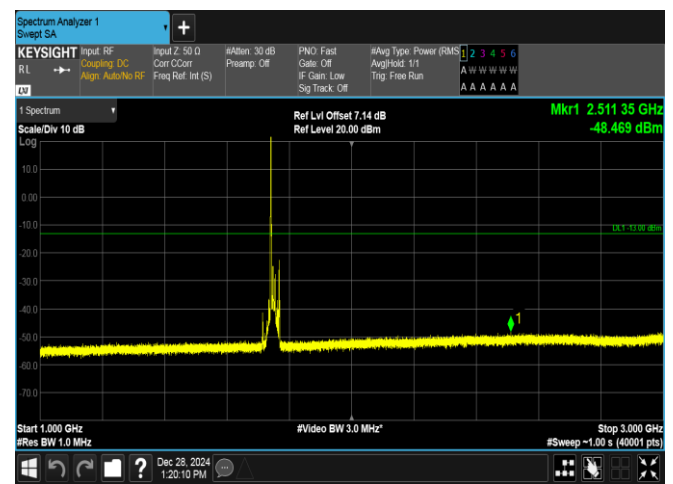
Band4-15MHz-QPSK-20325-1RB#0-1000~3000-PASS
