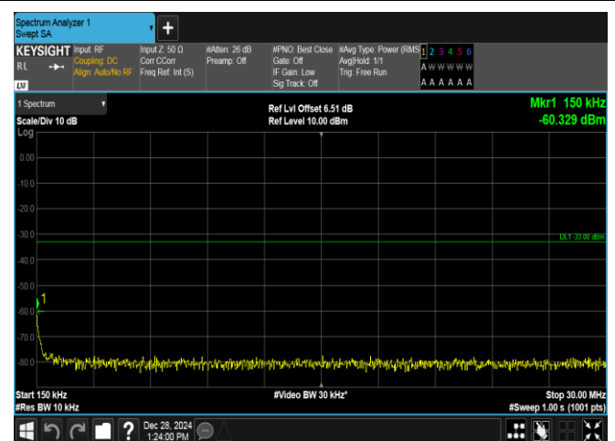
Band4-15MHz-QPSK-20325-75RB#0-0.15~30-PASS
