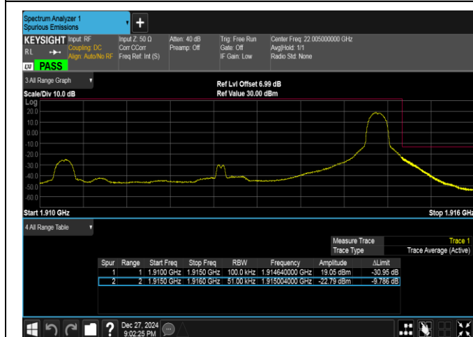
Band25-5MHz-QPSK-26665-1RB#24-PASS
