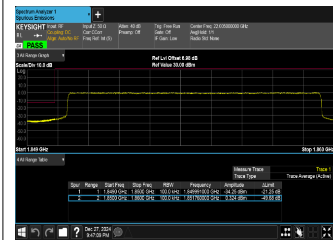
Band25-10MHz-QPSK-26090-50RB#0-PASS
