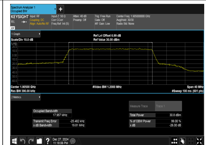
Band25-20MHz-16QAM-26590-100RB#0-PASS
