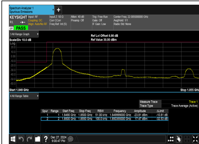
Band25-5MHz-16QAM-26065-1RB#0-PASS
