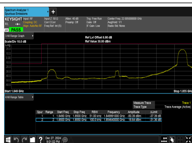
Band25-5MHz-QPSK-26065-1RB#24-PASS
