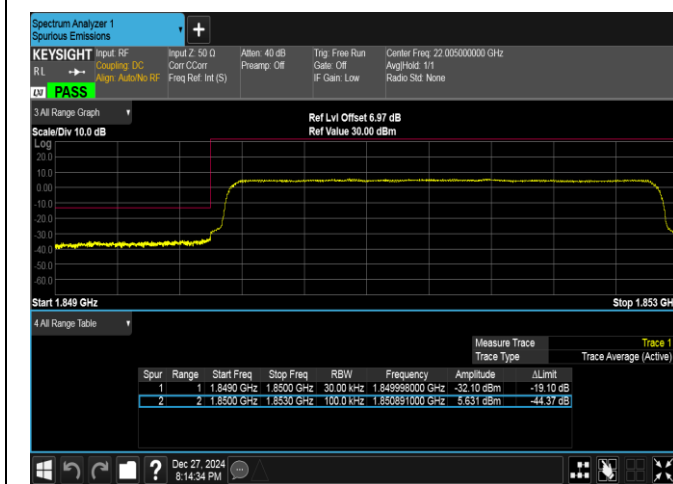
Band25-3MHz-QPSK-26055-15RB#0-PASS
