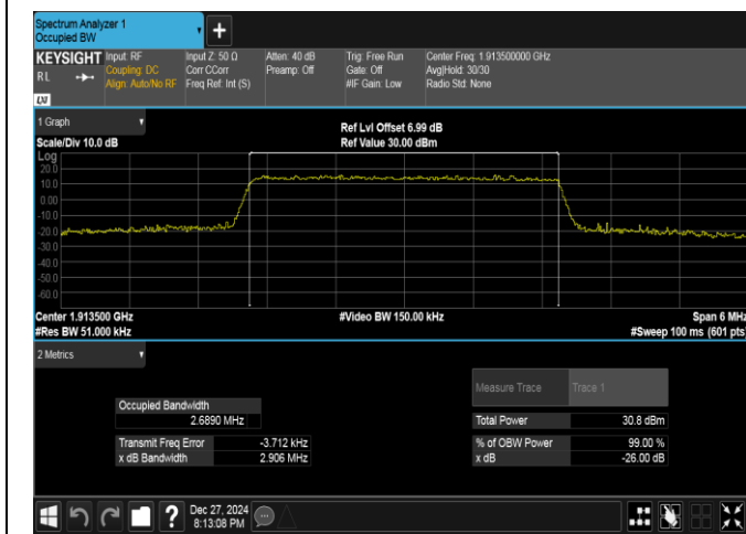
Band25-3MHz-QPSK-26675-15RB#0-PASS
