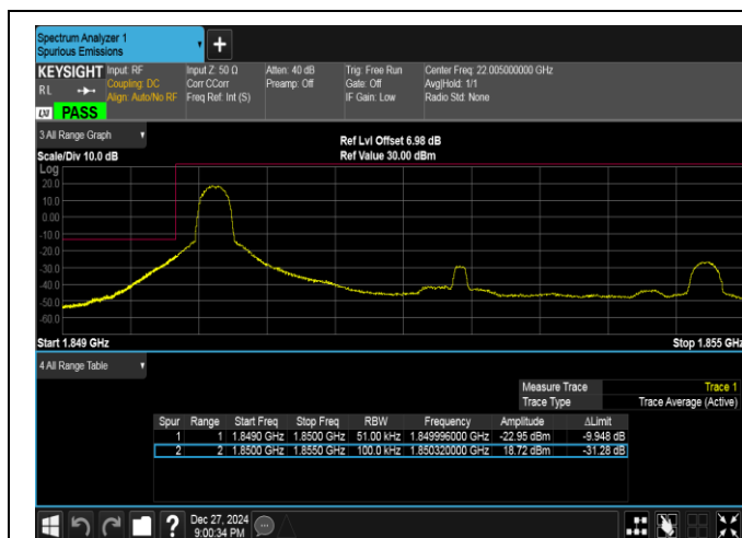
Band25-5MHz-QPSK-26065-1RB#0-PASS
