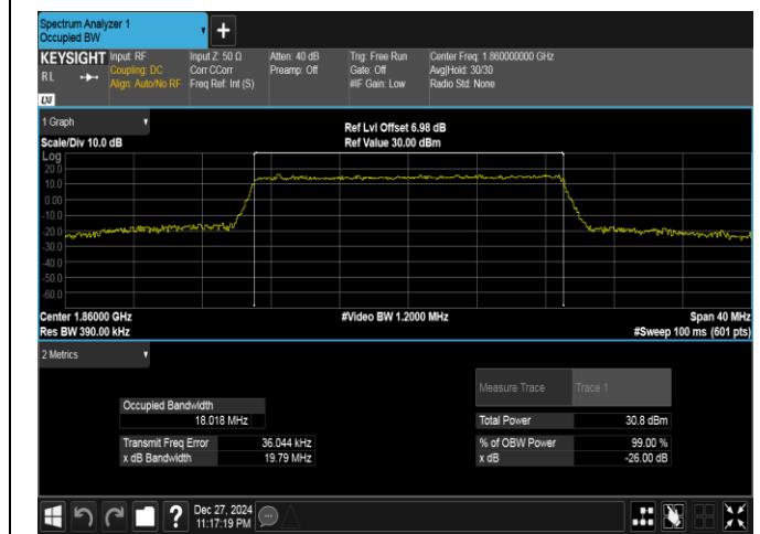
Band25-20MHz-16QAM-26140-100RB#0-PASS
