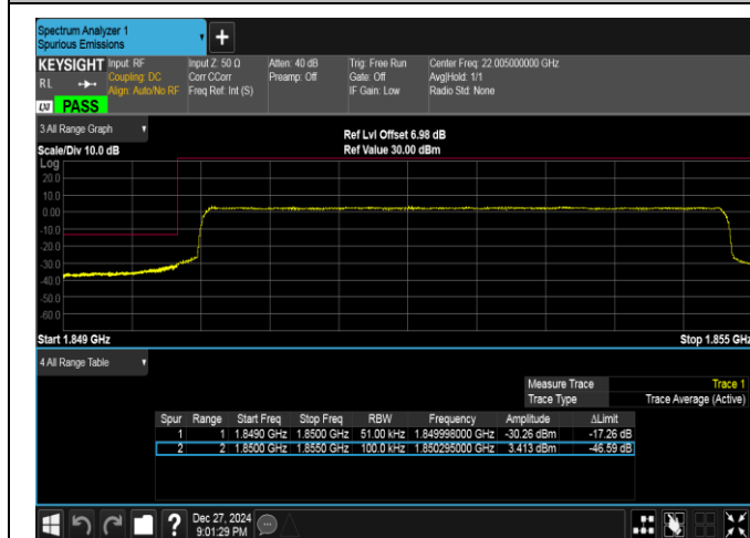
Band25-5MHz-QPSK-26065-25RB#0-PASS
