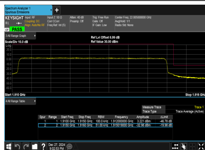
Band25-5MHz-QPSK-26665-25RB#0-PASS
