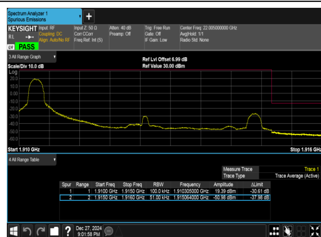
Band25-5MHz-QPSK-26665-1RB#0-PASS
