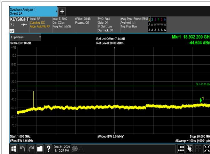
Band38-10MHz-QPSK-37800-1RB#49-1000~20000-PASS
