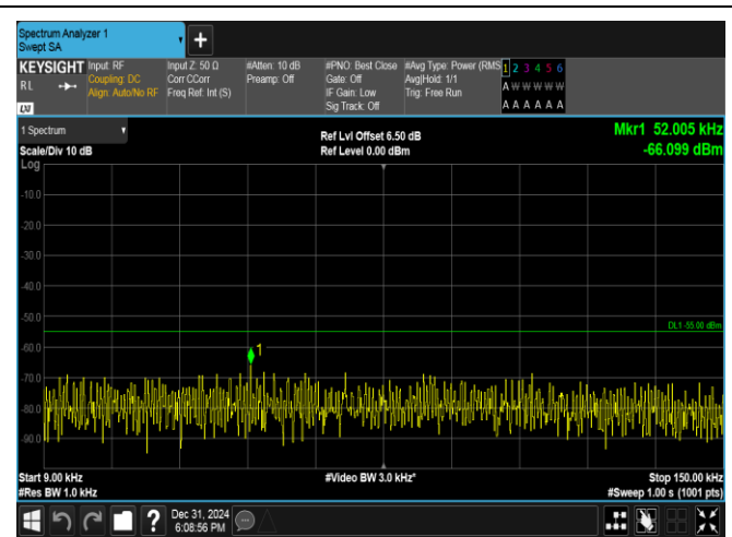
Band38-10MHz-16QAM-37800-1RB#0-0.009~0.15-PASS
