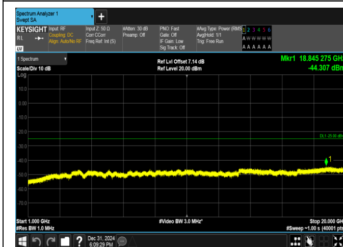
Band38-10MHz-16QAM-37800-1RB#0-1000~20000-PASS
