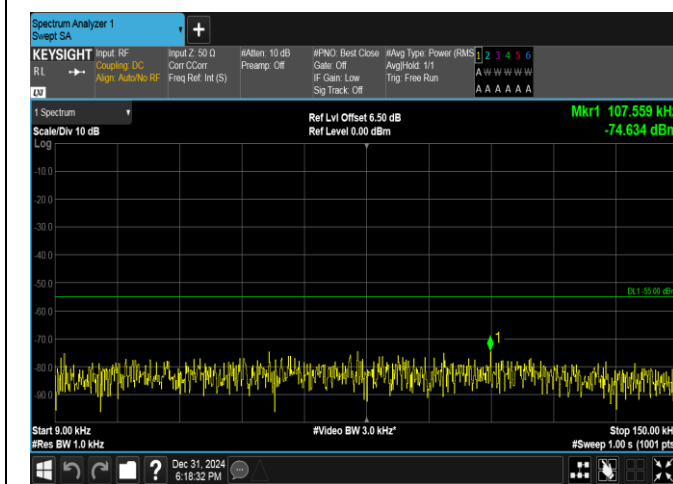
Band38-10MHz-16QAM-38000-50RB#0-0.009~0.15-PASS
