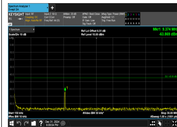
Band38-10MHz-16QAM-37800-1RB#0-0.15~30-PASS
