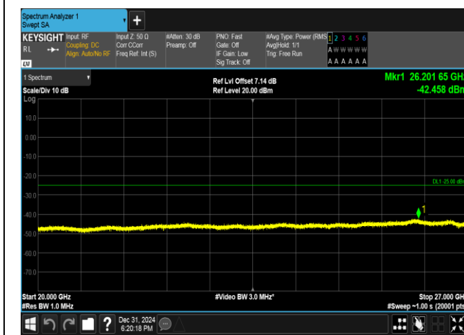
Band38-10MHz-QPSK-38200-1RB#0-20000~27000-PASS
