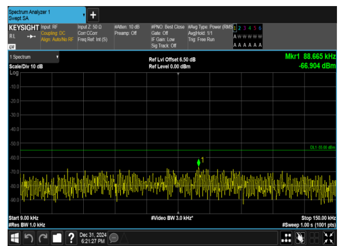
Band38-10MHz-QPSK-38200-1RB#49-0.009~0.15-PASS
