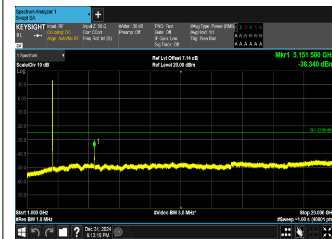
Band38-10MHz-16QAM-37800-50RB#0-1000~20000-PASS
