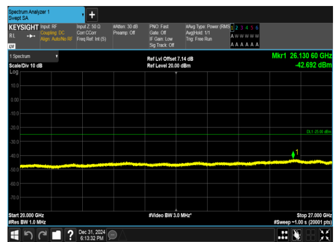
Band38-10MHz-16QAM-37800-50RB#0-20000~27000-PASS
