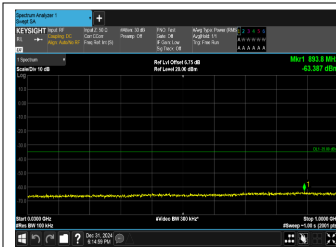
Band38-10MHz-16QAM-38000-1RB#0-30~1000-PASS
