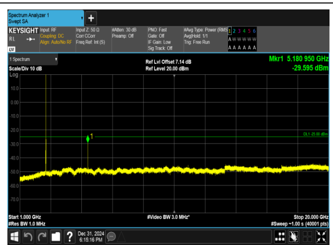
Band38-10MHz-16QAM-38000-1RB#0-1000~20000-PASS
