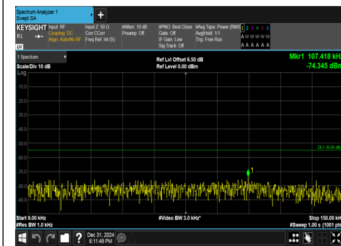
Band38-10MHz-QPSK-37800-50RB#0-0.009~0.15-PASS
