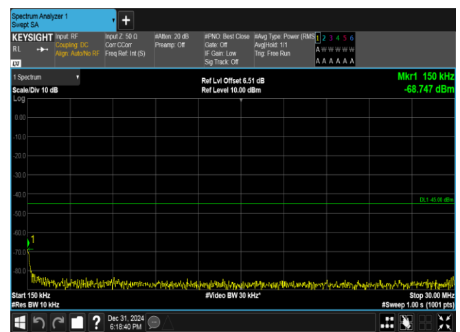
Band38-10MHz-16QAM-38000-50RB#0-0.15~30-PASS
