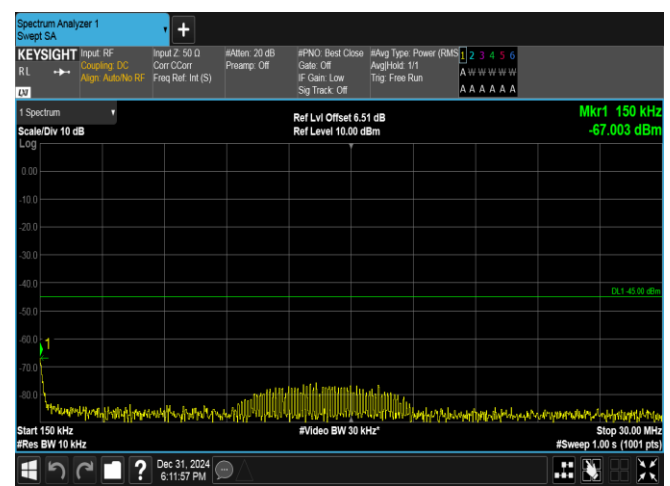
Band38-10MHz-QPSK-37800-50RB#0-0.15~30-PASS
