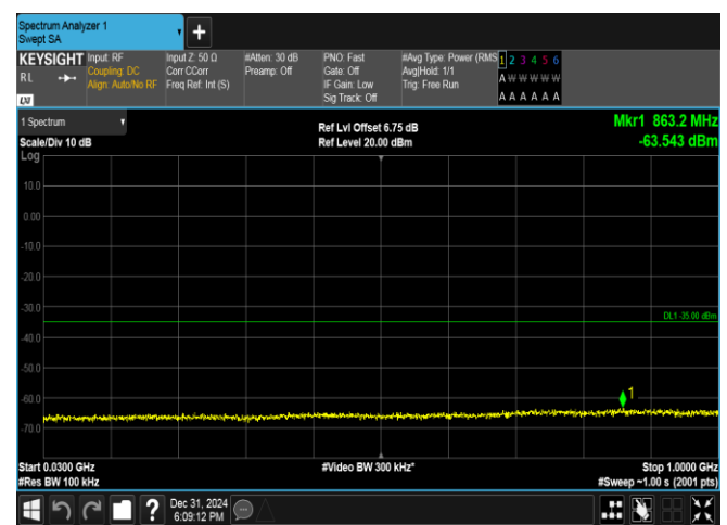
Band38-10MHz-16QAM-37800-1RB#0-30~1000-PASS
