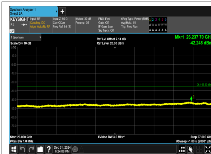
Band38-10MHz-QPSK-38200-50RB#0-20000~27000-PASS
