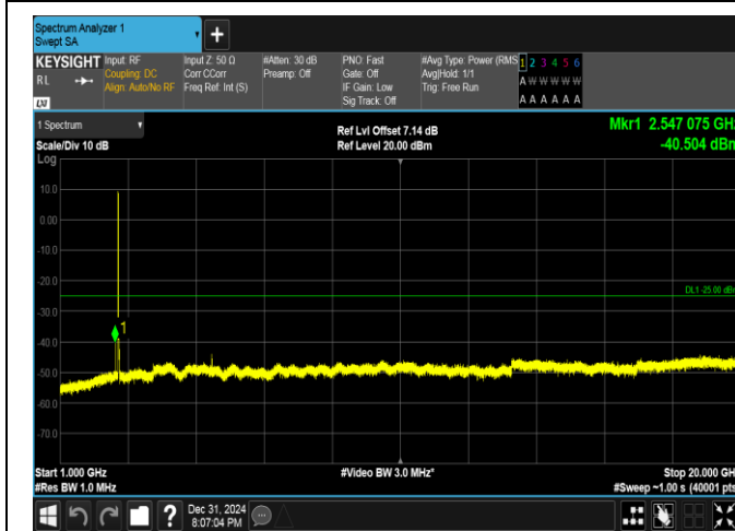
Band38-20MHz-16QAM-38150-100RB#0-1000~20000-PASS
