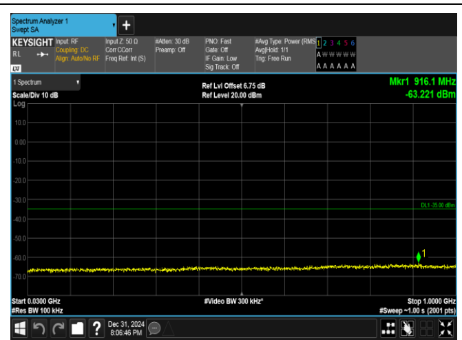
Band38-20MHz-16QAM-38150-100RB#0-30~1000-PASS
