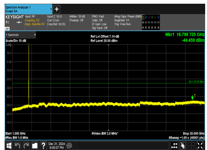
Band38-20MHz-16QAM-38150-1RB#99-1000~20000-PASS
