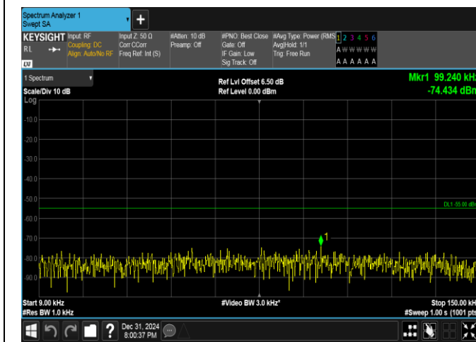
Band38-20MHz-16QAM-38000-100RB#0-0.009~0.15-PASS
