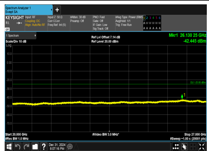
Band38-20MHz-16QAM-38150-100RB#0-20000~27000-PASS
