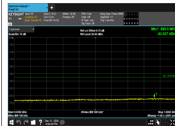
Band38-20MHz-16QAM-38150-1RB#99-30~1000-PASS
