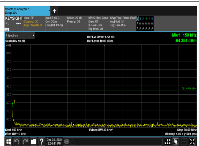
Band38-20MHz-16QAM-38150-1RB#99-0.15~30-PASS
