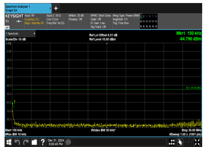
Band38-20MHz-16QAM-38000-100RB#0-0.15~30-PASS
