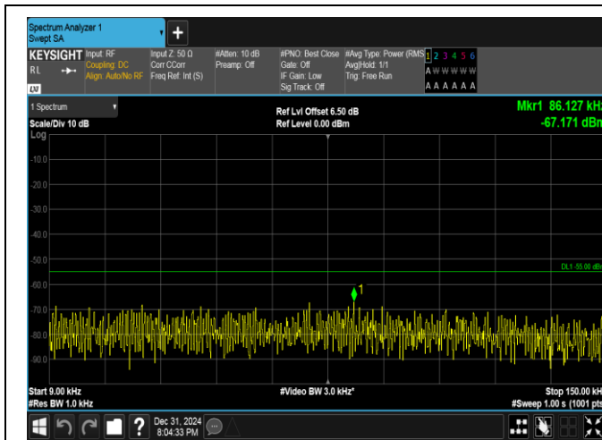
Band38-20MHz-16QAM-38150-1RB#99-0.009~0.15-PASS
