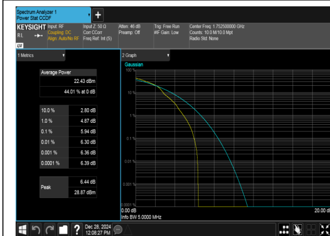
Band4-5MHz-16QAM-20375-1RB#0-PASS
