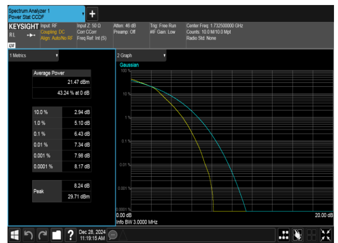
Band4-3MHz-16QAM-20175-15RB#0-PASS
