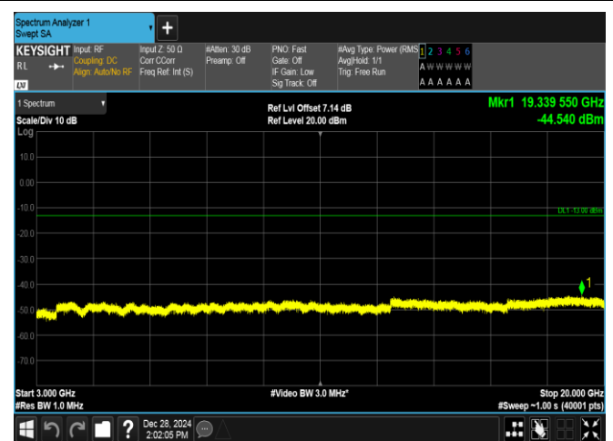
Band4-20MHz-16QAM-20050-100RB#0-3000~20000-PAS
