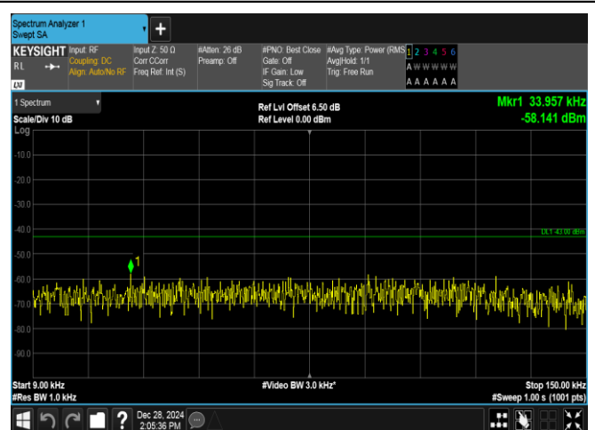
Band4-20MHz-16QAM-20175-1RB#99-0.009~0.15-PASS
