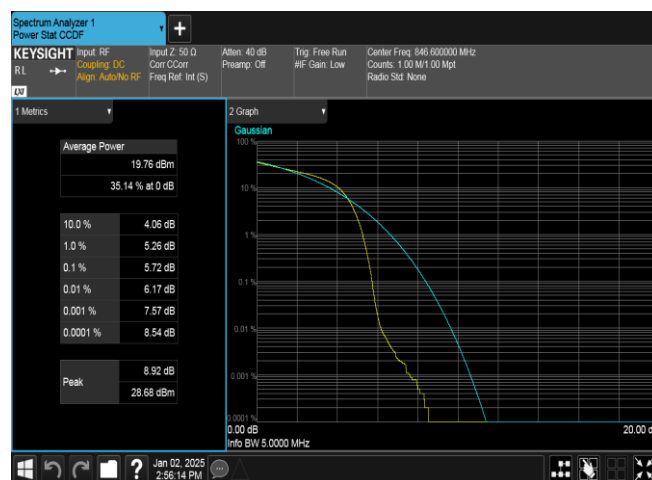
Band5-4233-2-PASS
