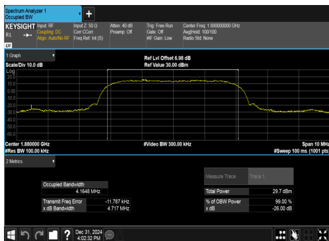
Band2-9400-4-PASS
