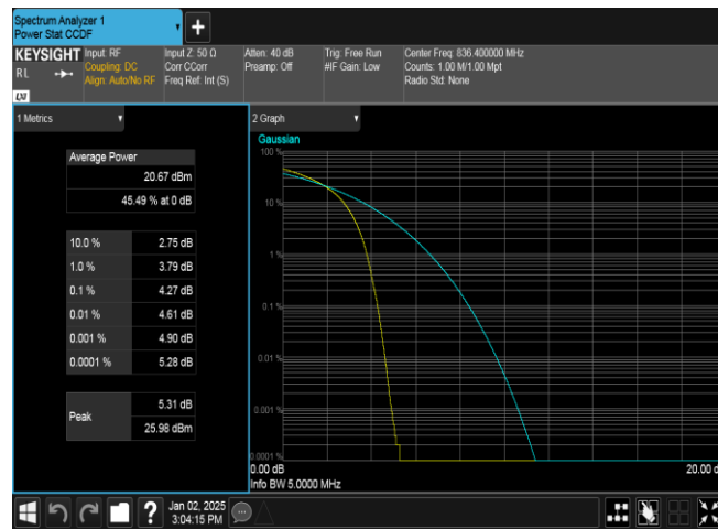
Band5-4182-5-PASS
