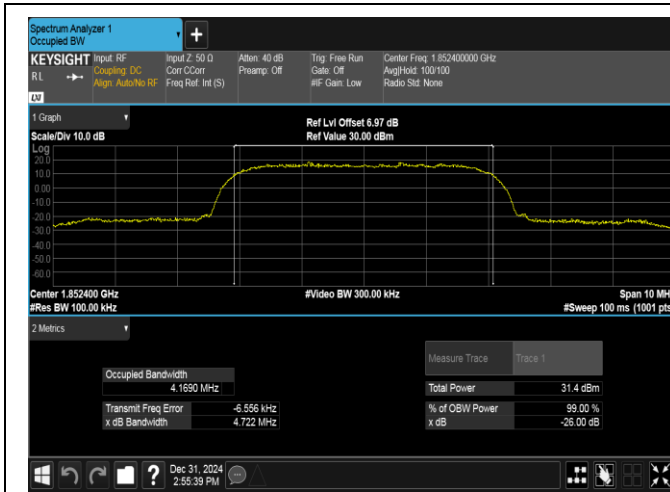
Band2-9262-PASS
