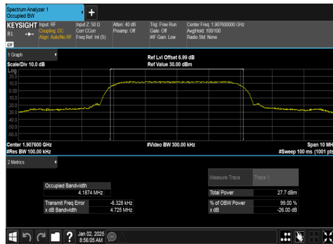
Band2-9538-4-PASS
