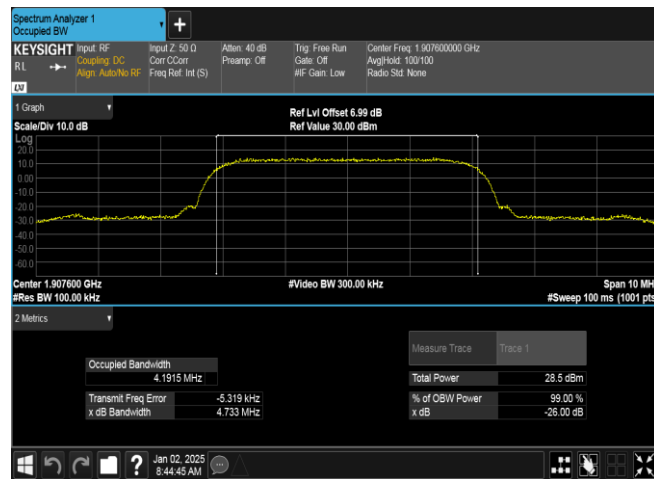
Band2-9538-1-PASS
