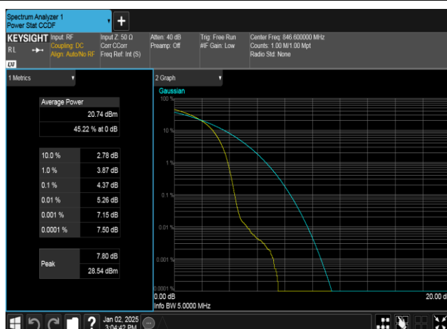
Band5-4233-5-PASS
