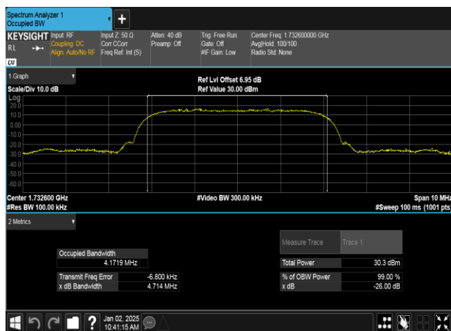
Band4-1413-1-PASS
