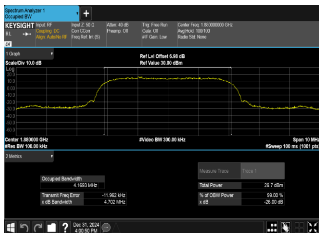
Band2-9400-3-PASS
