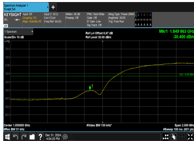
Band2-9262-2-PASS
