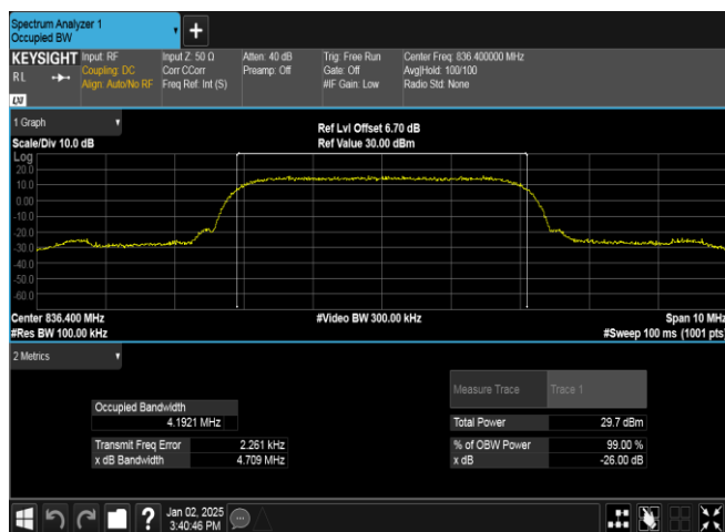
Band5-4182-3-PASS
