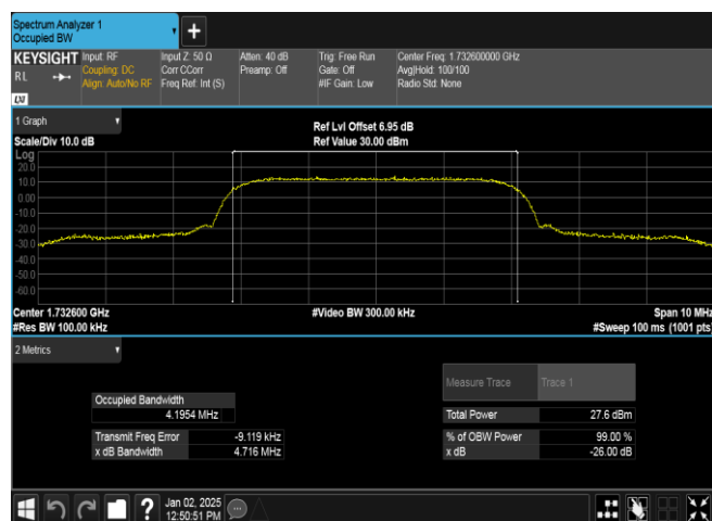
Band4-1413-4-PASS
