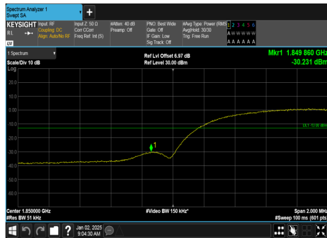
Band2-9262-4-PASS
