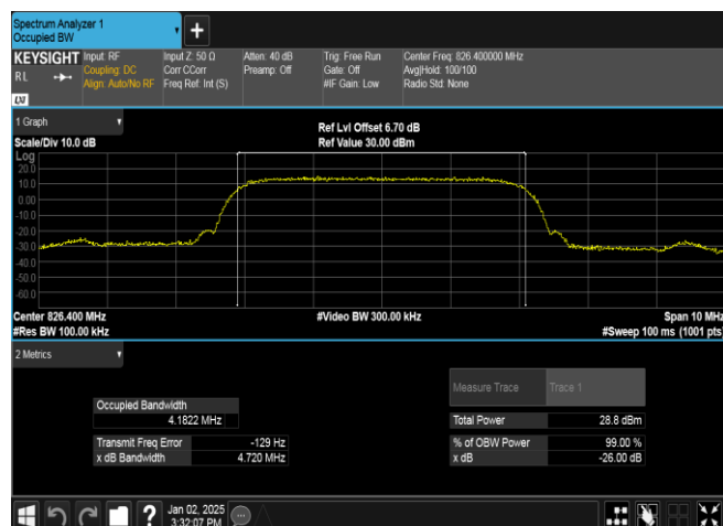
Band5-4132-1-PASS
