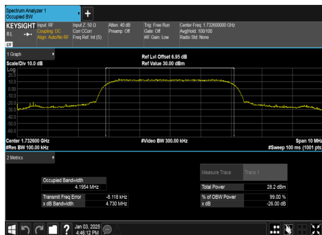
Band4-1413-2-PASS
