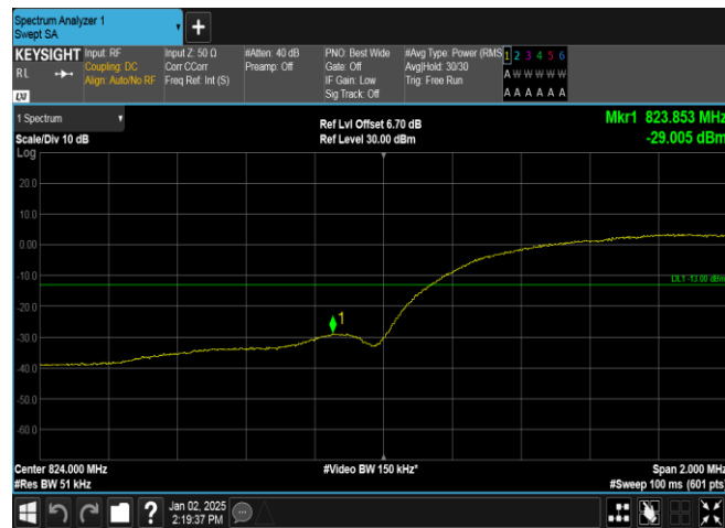
Band5-4132-4-PASS
