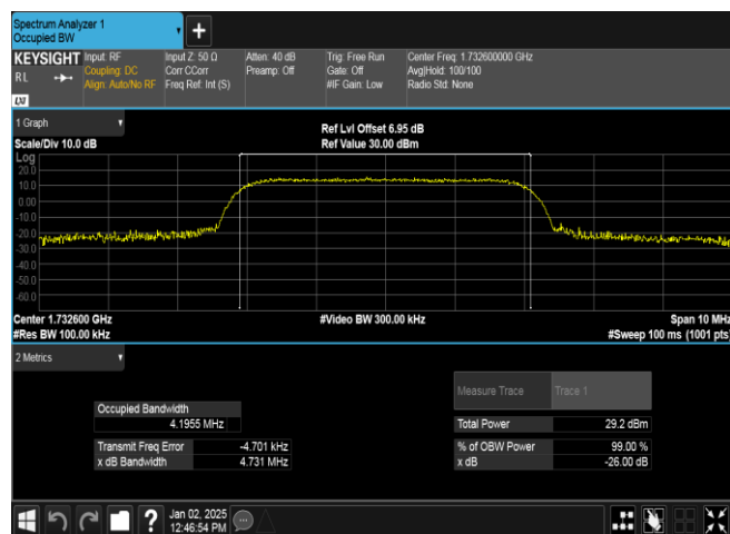
Band4-1413-3-PASS
