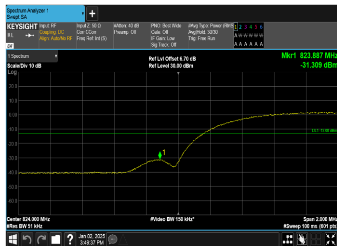
Band5-4132-1-PASS
