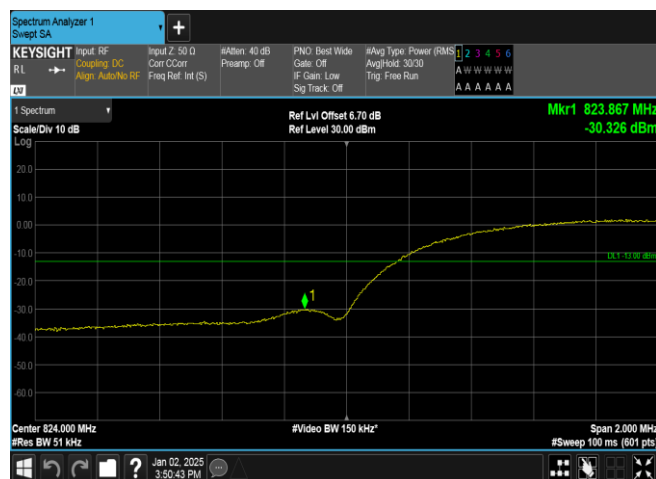
Band5-4132-2-PASS
