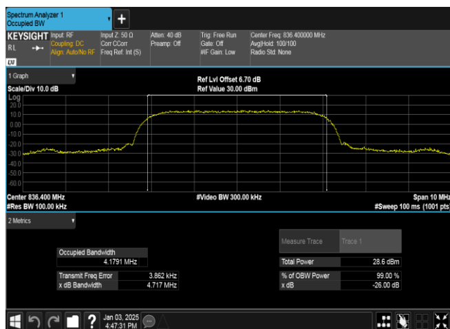
Band5-4182-2-PASS
