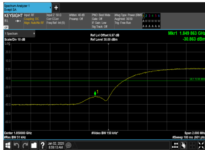
Band2-9262-1-PASS
