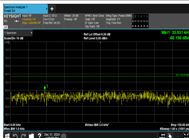
Band2-9538-1-0.009~0.15MHz-PASS
