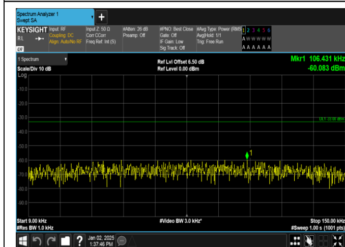
Band5-4182-0.009~0.15MHz-PASS
