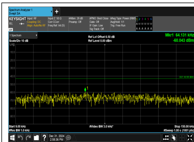
Band2-9538-0.009~0.15MHz-PASS
