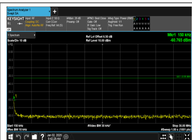
Band4-1513-0.15~30MHz-PASS
