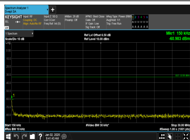
Band4-1413-0.15~30MHz-PASS
