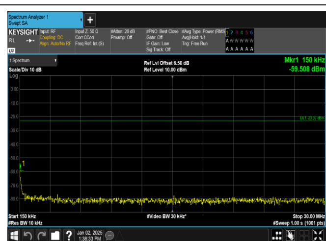
Band5-4233-0.15~30MHz-PASS
