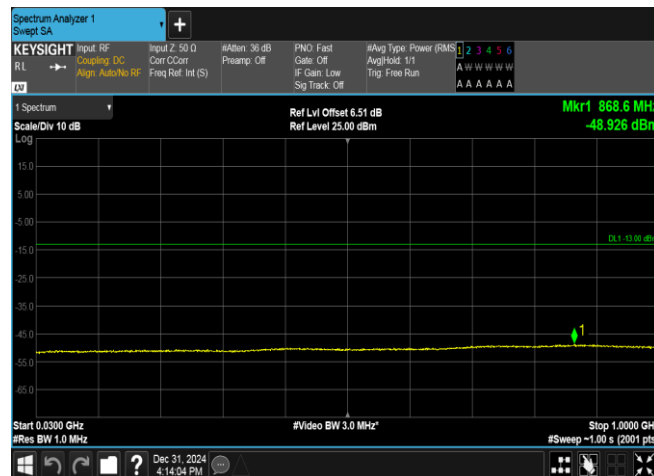
Band2-9400-4-30~1000MHz-PASS
