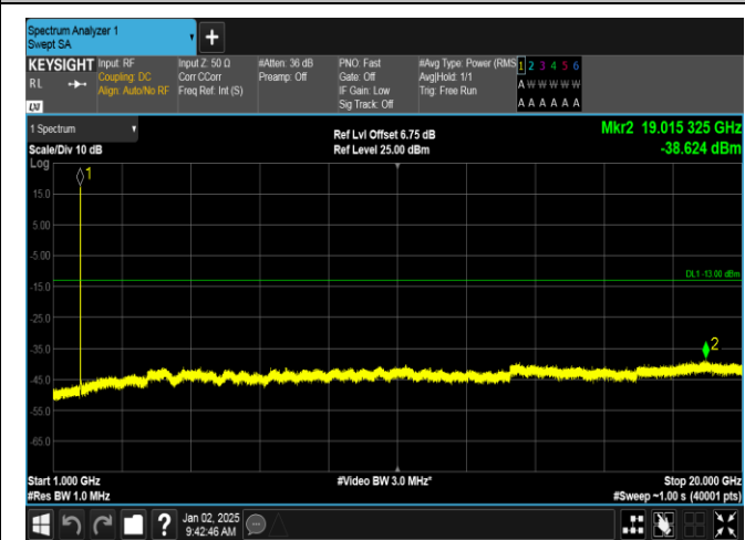
Band4-1513-1000~20000MHz-PASS
