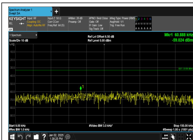
Band5-4233-0.009~0.15MHz-PASS
