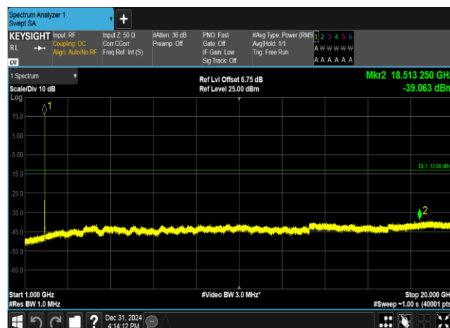
Band2-9400-4-1000~20000MHz-PASS
