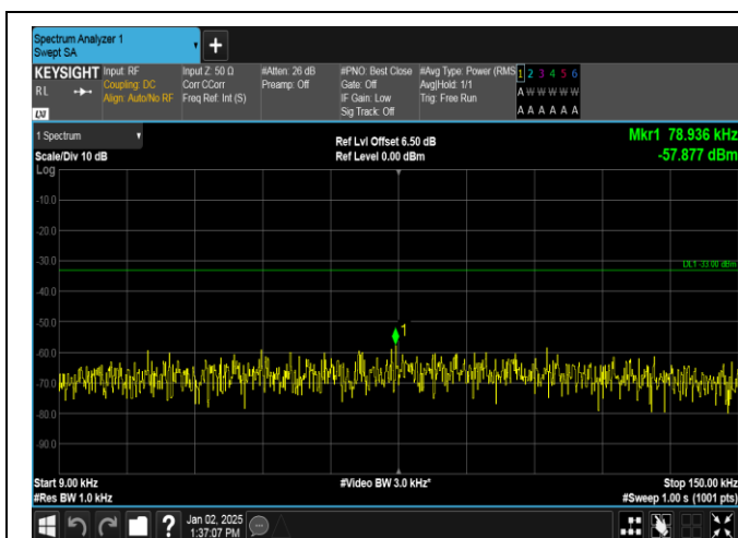
Band5-4132-0.009~0.15MHz-PASS
