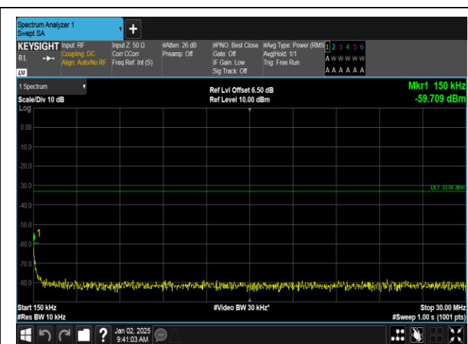
Band4-1312-0.15~30MHz-PASS
