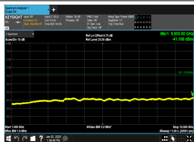
Band5-4233-1000~10000MHz-PASS
