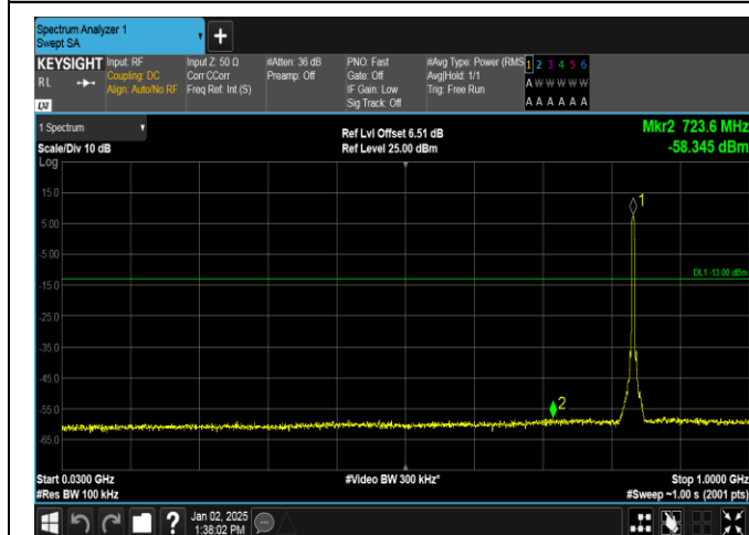
Band5-4182-30~1000MHz-PASS
