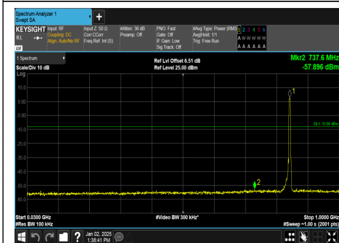
Band5-4233-30~1000MHz-PASS
