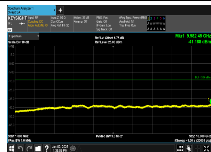
Band5-4182-1000~10000MHz-PASS
