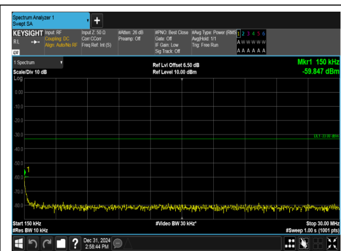
Band2-9538-0.15~30MHz-PASS
