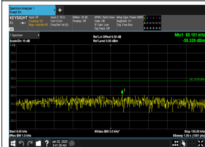
Band4-1413-0.009~0.15MHz-PASS
