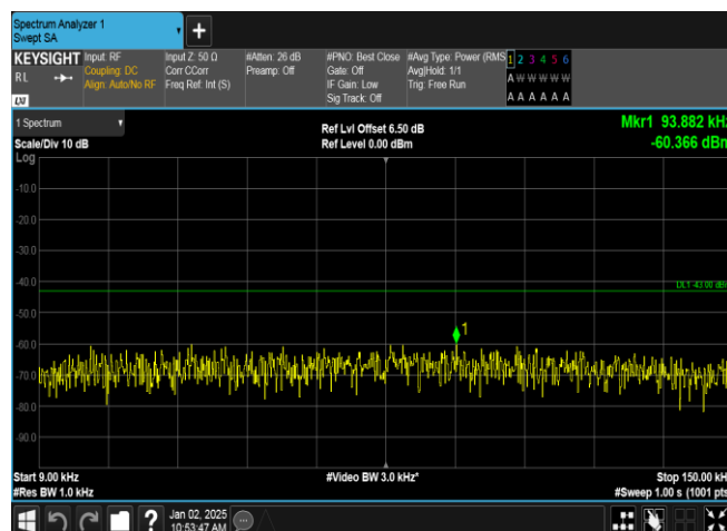
Band4-1513-2-0.009~0.15MHz-PASS
