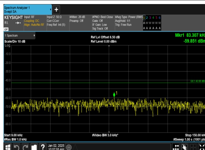
Band4-1513-4-0.009~0.15MHz-PASS
