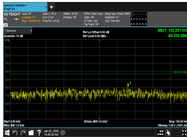
Band4-1312-1-0.009~0.15MHz-PASS
