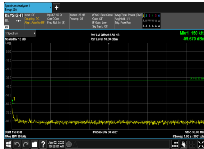
Band4-1513-4-0.15~30MHz-PASS
