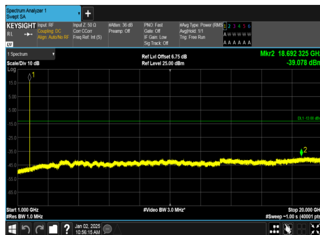
Band4-1513-3-1000~20000MHz-PASS
