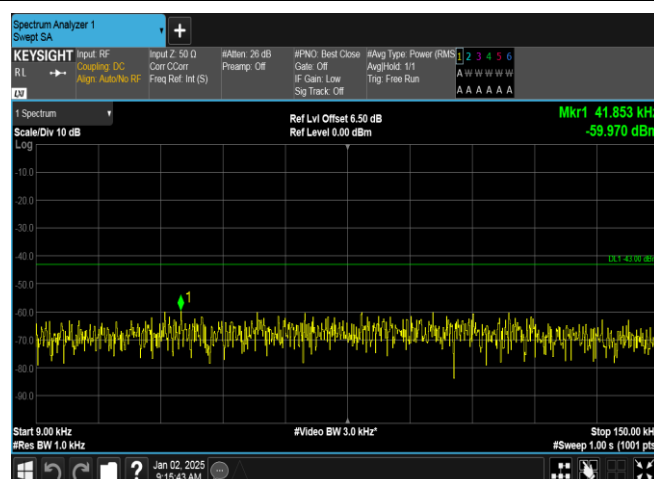
Band2-9538-2-0.009~0.15MHz-PASS
