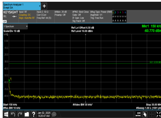
Band2-9538-5-0.15~30MHz-PASS
