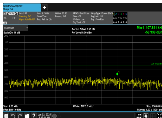
Band2-9538-5-0.009~0.15MHz-PASS
