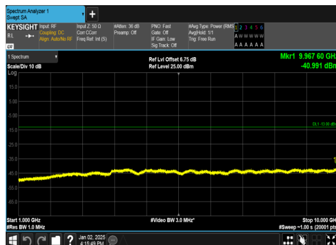
Band5-4132-5-1000~10000MHz-PASS
