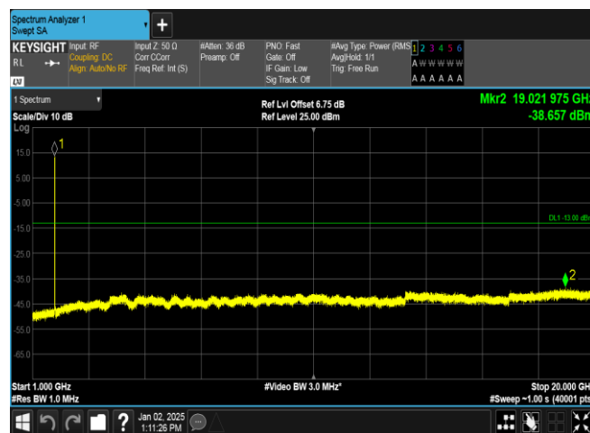
Band4-1513-1-1000~20000MHz-PASS
