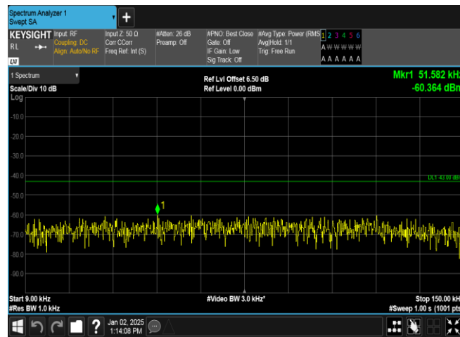
Band4-1413-2-0.009~0.15MHz-PASS
