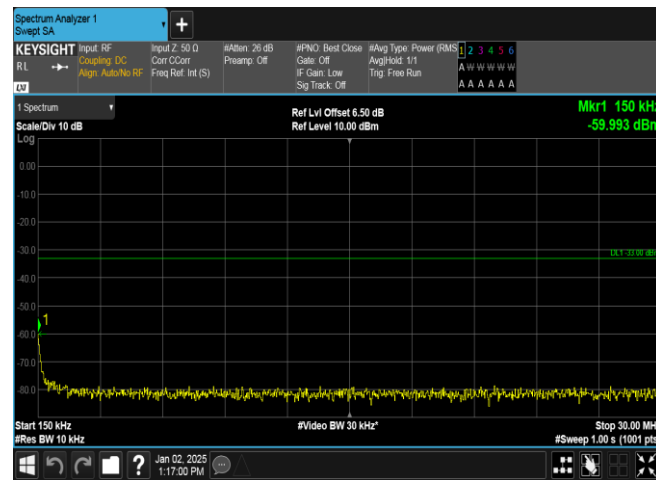
Band4-1312-3-0.15~30MHz-PASS
