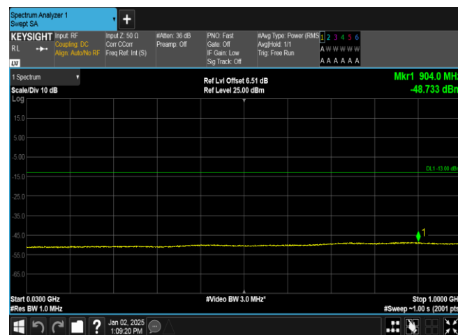
Band4-1413-1-30~1000MHz-PASS
