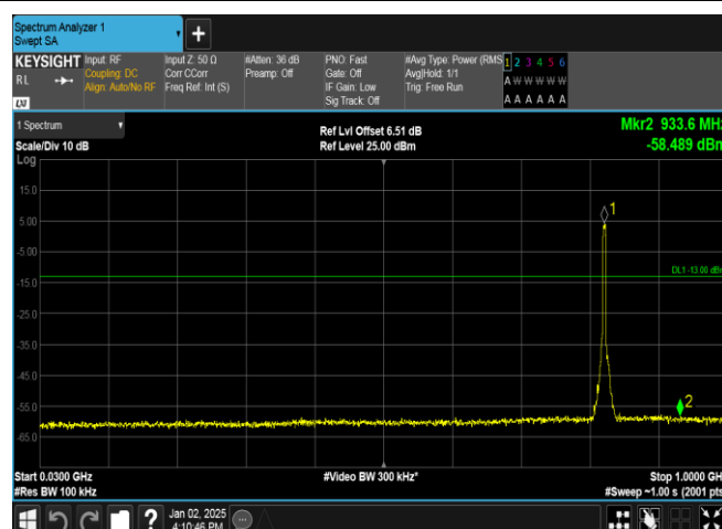
Band5-4132-4-30~1000MHz-PASS
