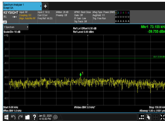
Band5-4132-4-0.009~0.15MHz-PASS
