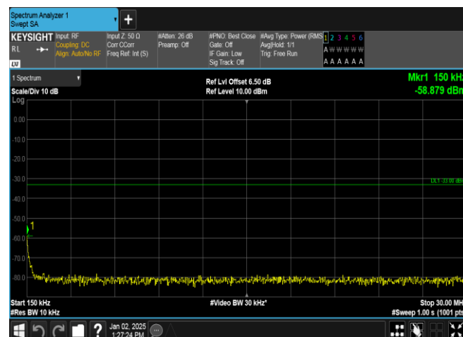
Band4-1413-5-0.15~30MHz-PASS
