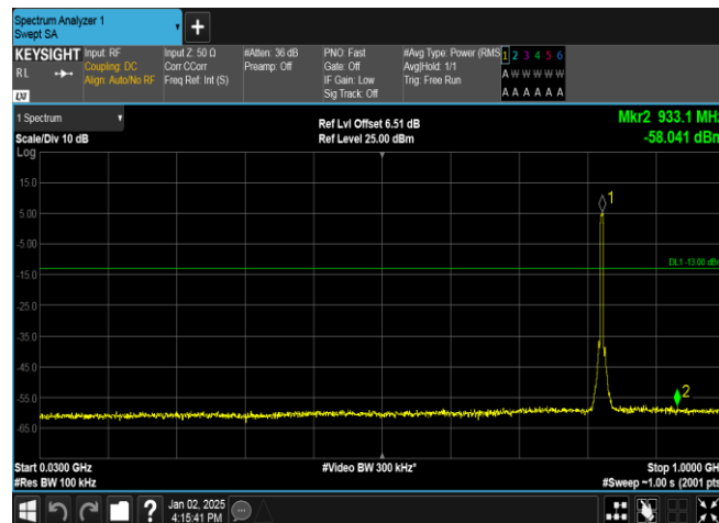
Band5-4132-5-30~1000MHz-PASS
