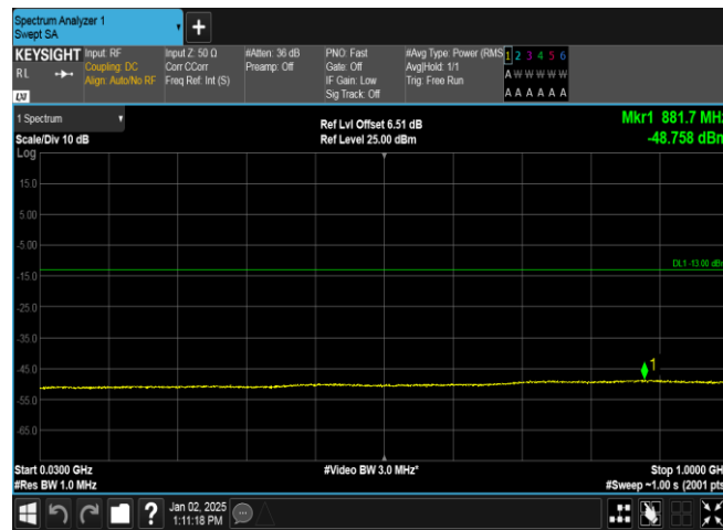
Band4-1513-1-30~1000MHz-PASS
