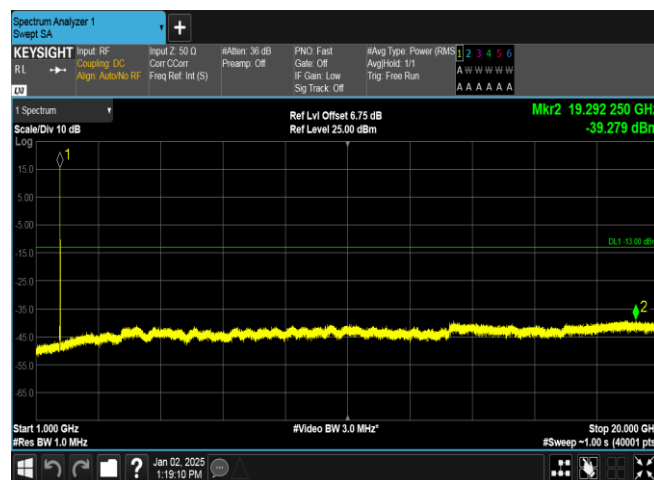
Band4-1413-3-1000~20000MHz-PASS
