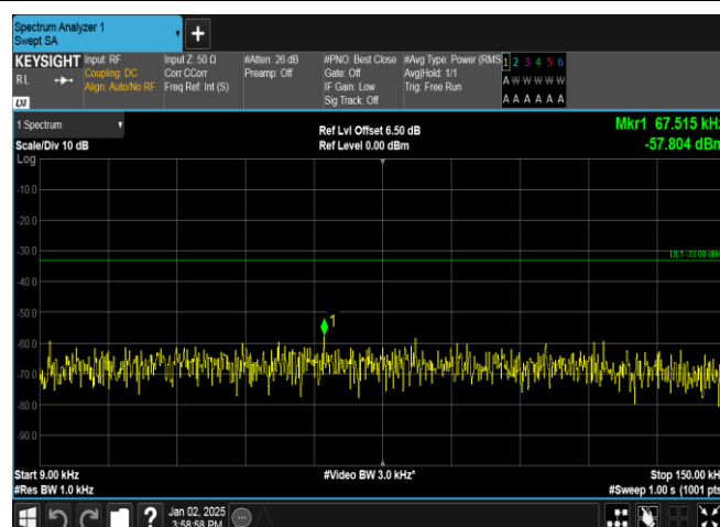
Band5-4182-1-0.009~0.15MHz-PASS
