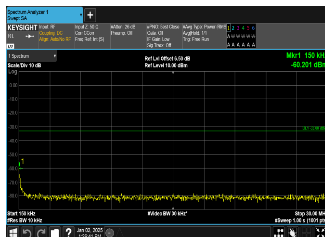
Band4-1312-5-0.15~30MHz-PASS
