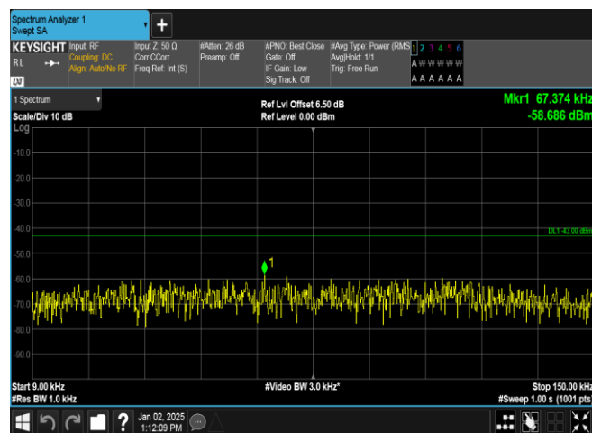
Band4-1312-2-0.009~0.15MHz-PASS
