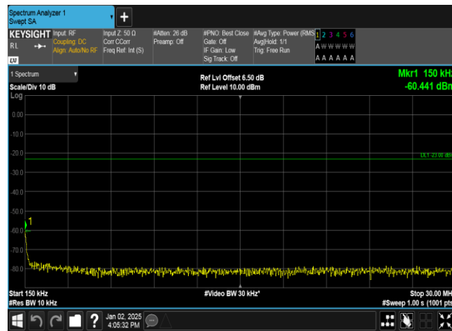
Band5-4132-3-0.15~30MHz-PASS
