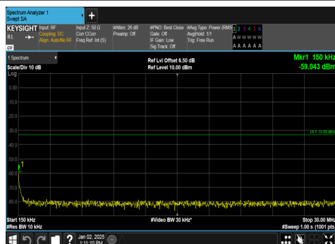
Band4-1513-1-0.15~30MHz-PASS
