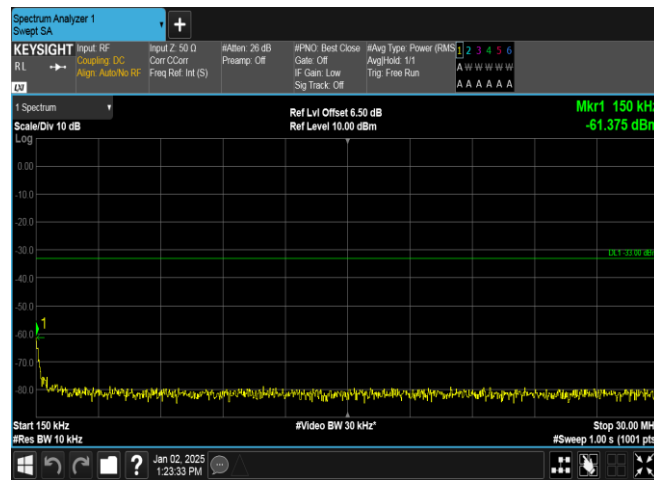
Band4-1413-4-0.15~30MHz-PASS
