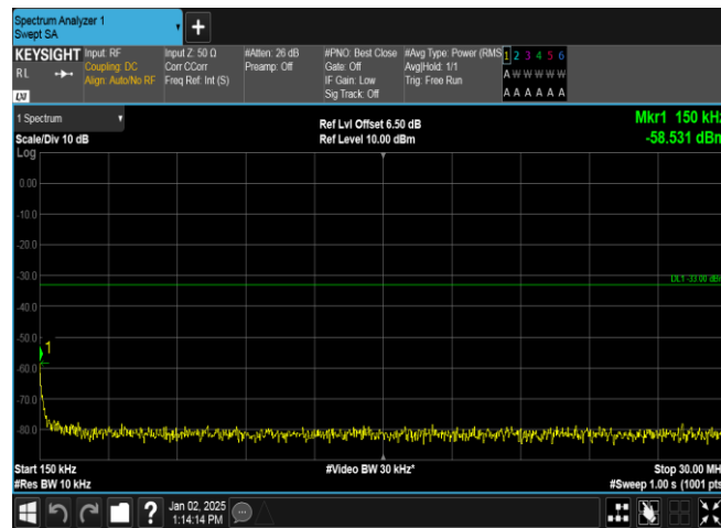
Band4-1413-2-0.15~30MHz-PASS
