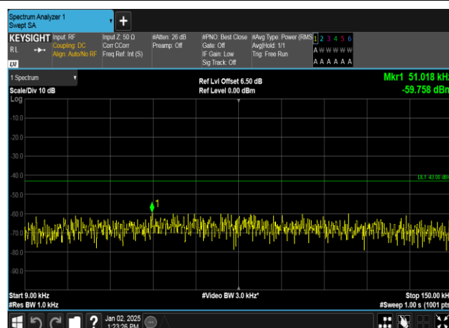
Band4-1413-4-0.009~0.15MHz-PASS
