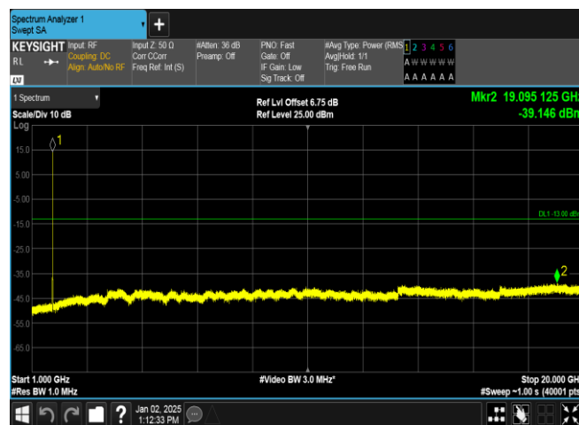
Band4-1312-2-1000~20000MHz-PASS
