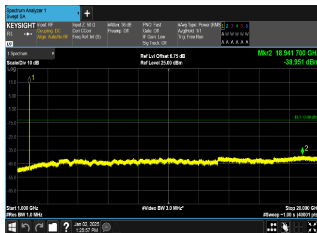
Band4-1513-4-1000~20000MHz-PASS
