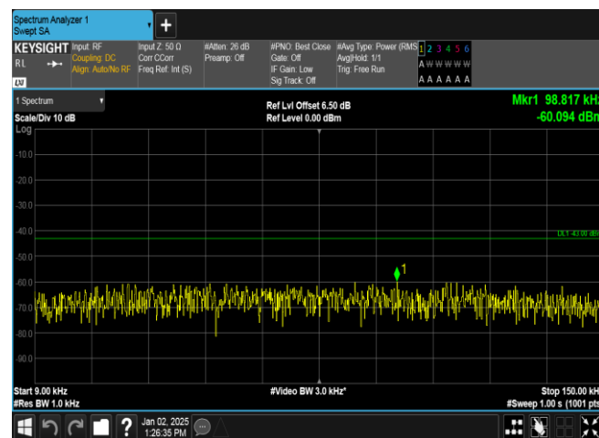
Band4-1312-5-0.009~0.15MHz-PASS
