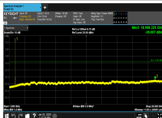
Band4-1312-3-1000~20000MHz-PASS
