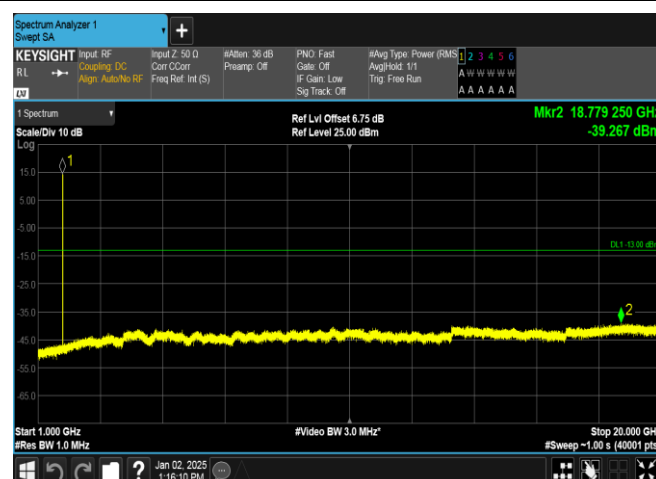
Band4-1513-2-1000~20000MHz-PASS
