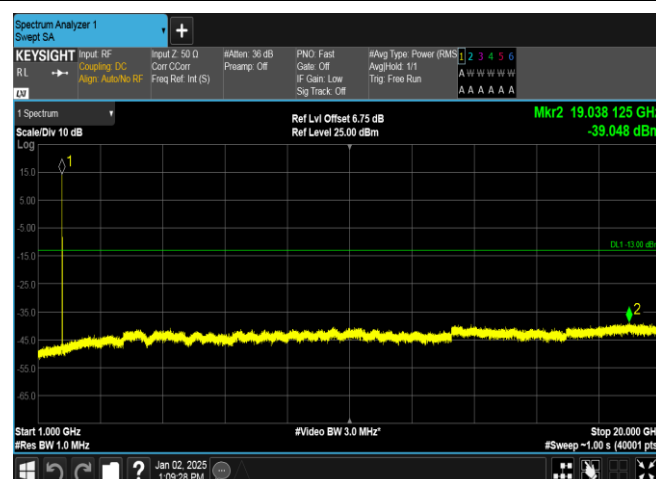
Band4-1413-1-1000~20000MHz-PASS
