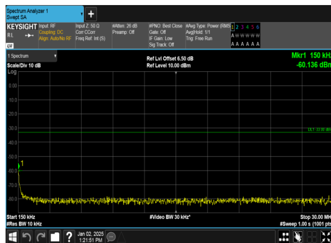
Band4-1312-4-0.15~30MHz-PASS
