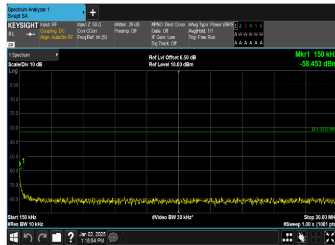
Band4-1513-2-0.15~30MHz-PASS
