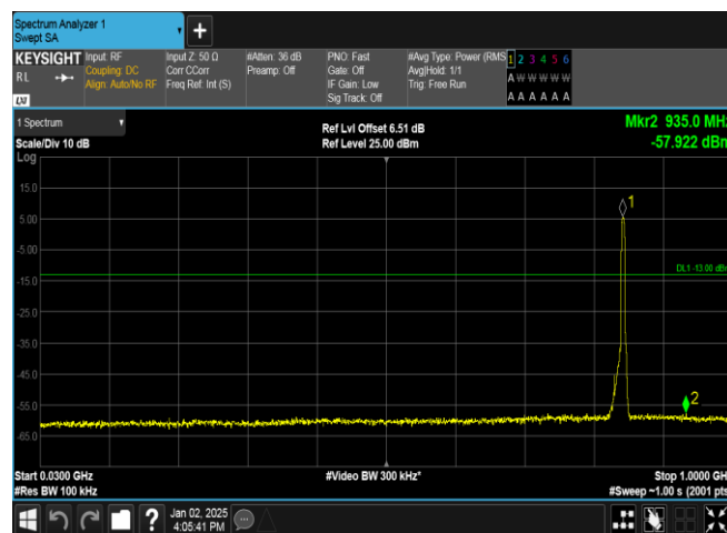
Band5-4132-3-30~1000MHz-PASS
