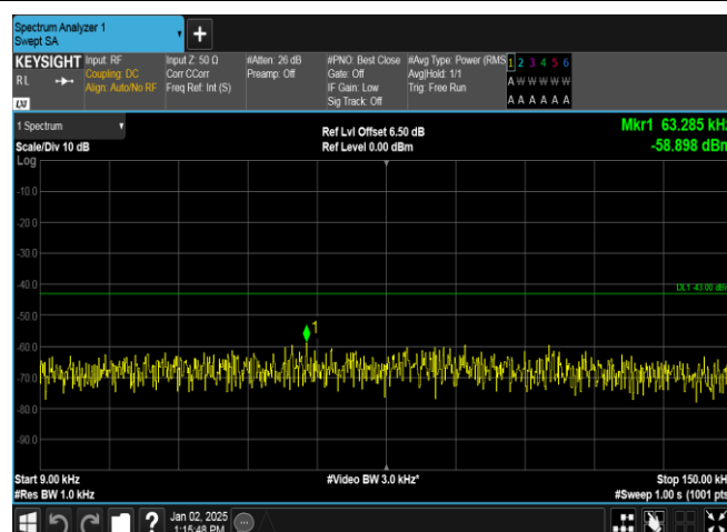
Band4-1513-2-0.009~0.15MHz-PASS
