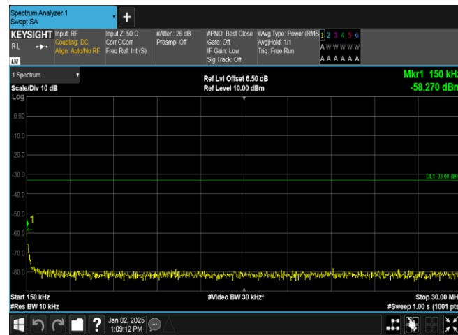
Band4-1413-1-0.15~30MHz-PASS
