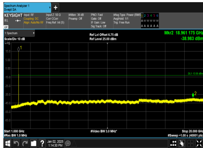
Band4-1413-2-1000~20000MHz-PASS
