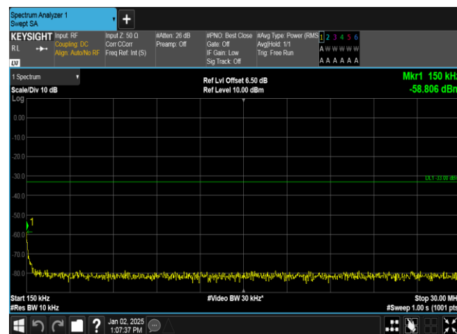
Band4-1312-1-0.15~30MHz-PASS
