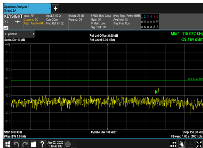
Band4-1413-3-0.009~0.15MHz-PASS
