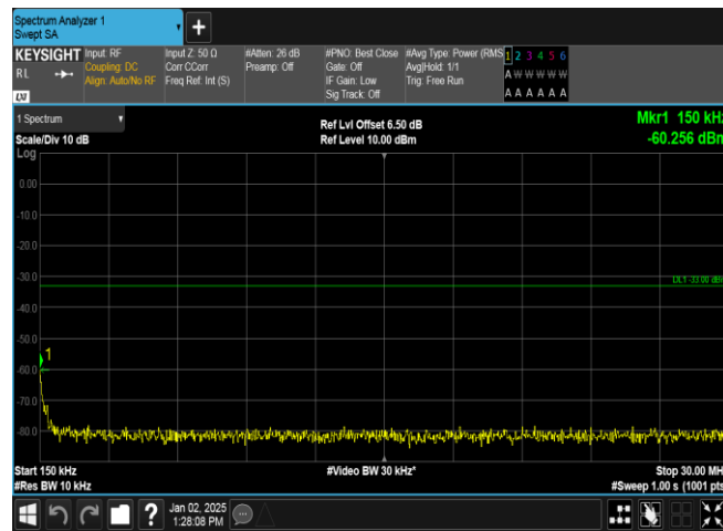
Band4-1513-5-0.15~30MHz-PASS
