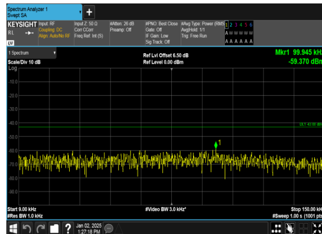
Band4-1413-5-0.009~0.15MHz-PASS
