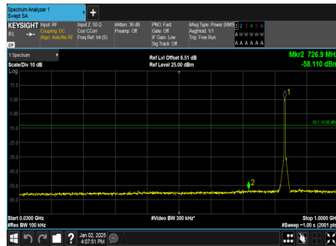
Band5-4182-3-30~1000MHz-PASS
