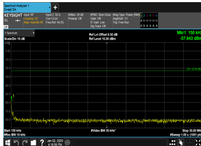
Band5-4233-5-0.15~30MHz-PASS
