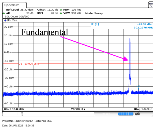
30 MHz – 1GHz WCDMA (HSDPA) Mode, High channel
