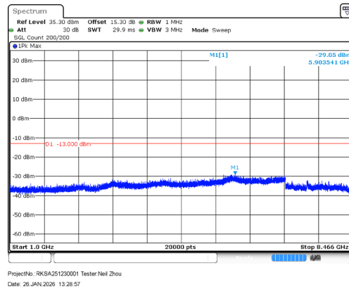
1 GHz – 8.466 GHz WCDMA (HSDPA) Mode, High channel
