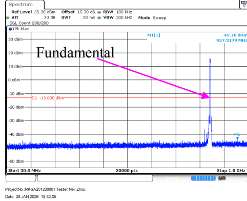
30 MHz – 1GHz WCDMA (Rel 99) Mode, High channel
