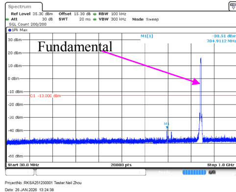
30 MHz – 1GHz WCDMA (HSUPA) Mode, High channel
