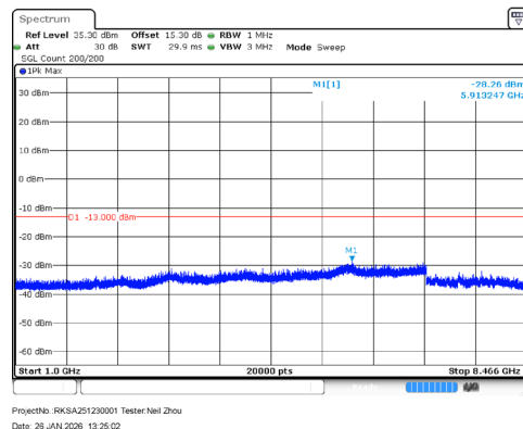
1 GHz – 8.466 GHz WCDMA (HSUPA) Mode, High channel
