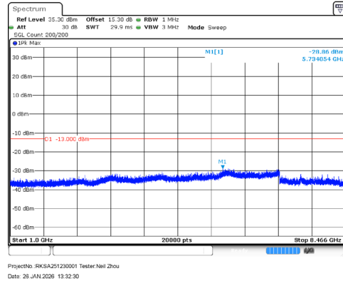
1 GHz – 8.466 GHz WCDMA (Rel 99) Mode, High channel
