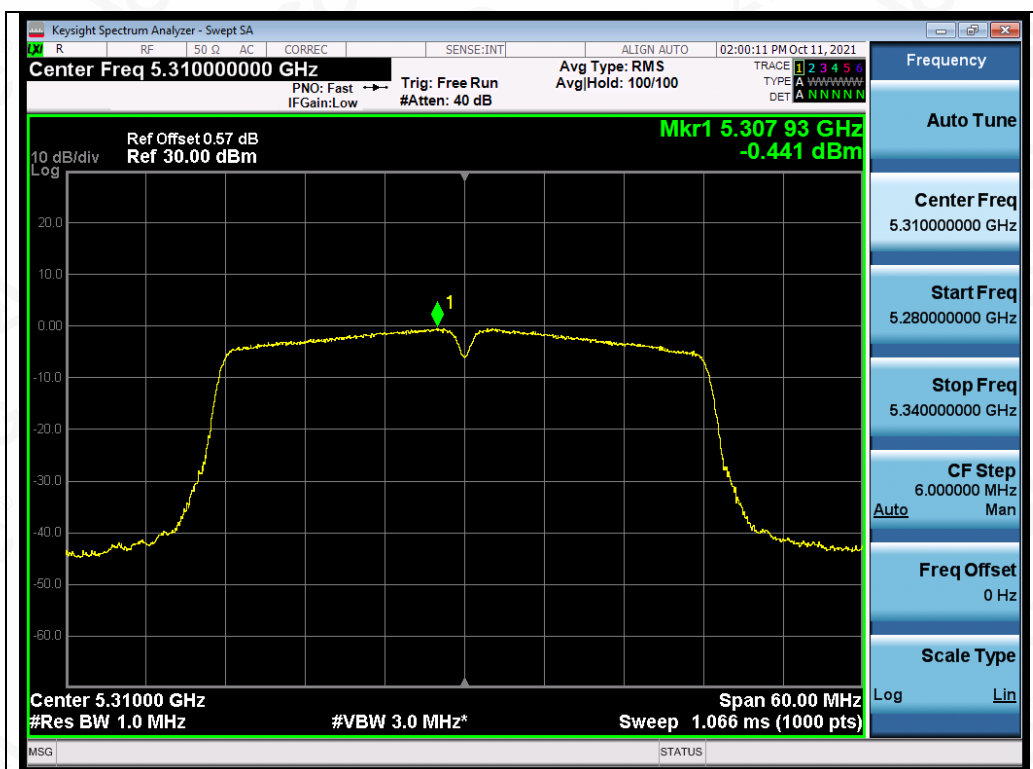
Test_Graph_802.11ac40_ANT1_5310_MCS9_PSD
