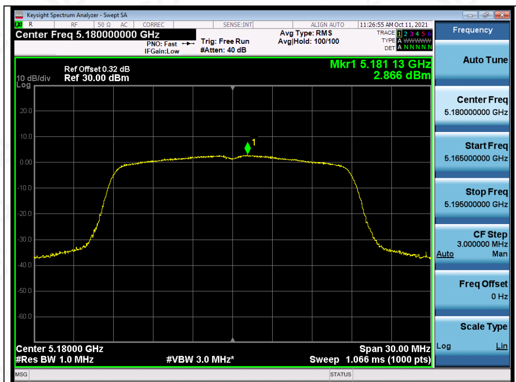
Test_Graph_802.11ac20_ANT1_5180_MCS0_PSD
