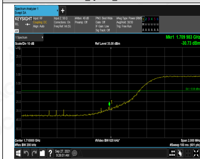
LCH_QPSK_50RB#0
