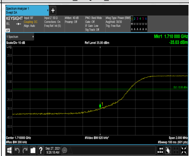
LCH_16QAM_50RB#0
