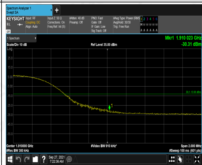
HCH_16QAM_75RB#0
