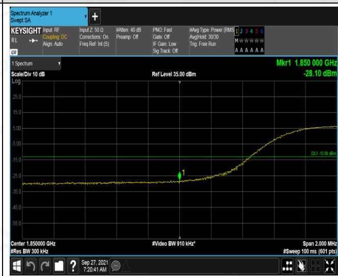
LCH_16QAM_75RB#0
