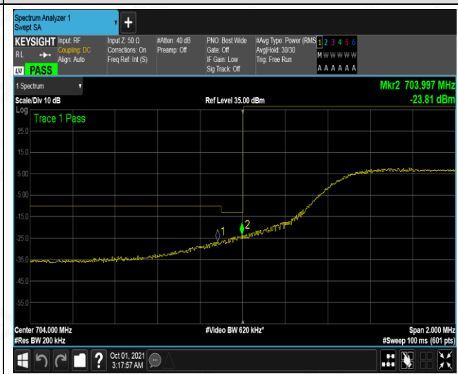
LCH_16QAM_50RB#0
