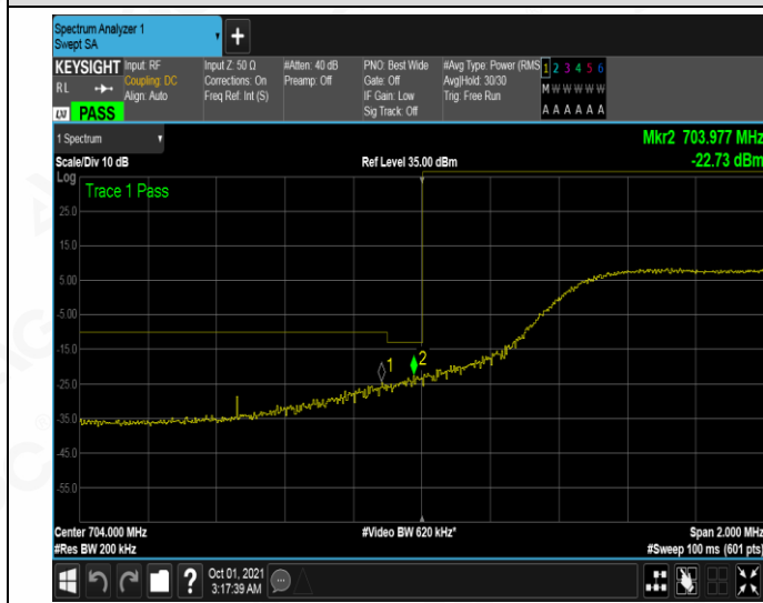
LCH_QPSK_50RB#0
