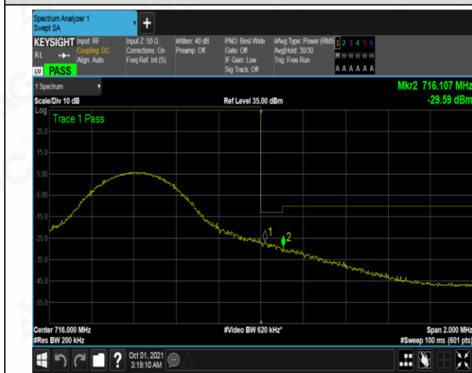
HCH_QPSK_50RB#0
