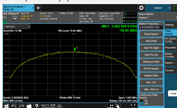
GFSK (BLE 1Mbps) LOW CHANNEL
