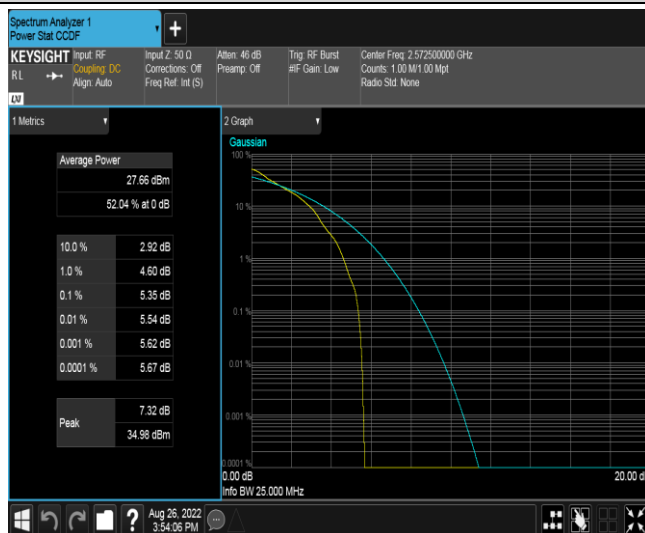
Band38-5MHz-QPSK-37775-25RB#0
