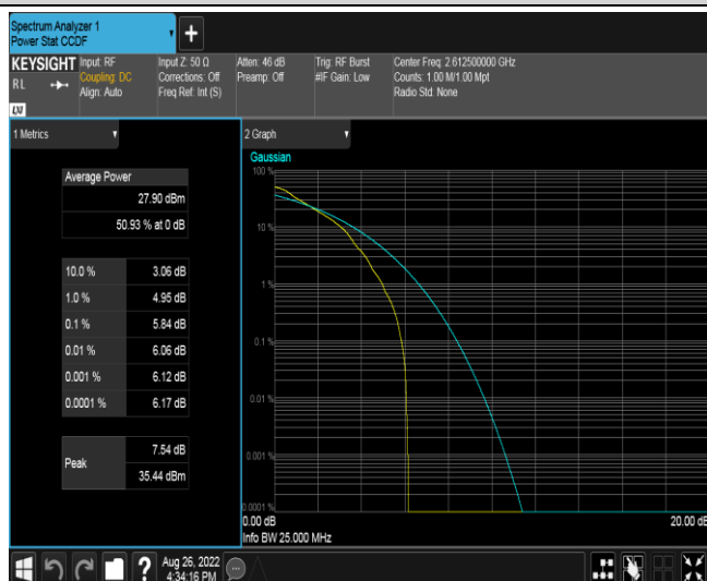
Band38-15MHz-QPSK-38175-75RB#0
