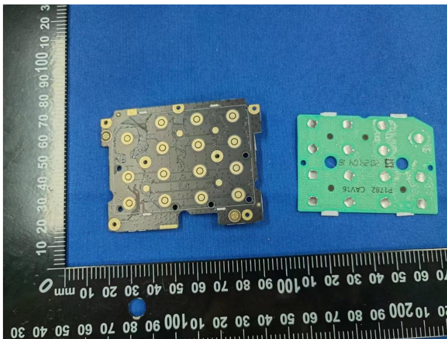
MAIN BOARD 2 TOP VIEW (WITHOUT SHIELDING)
