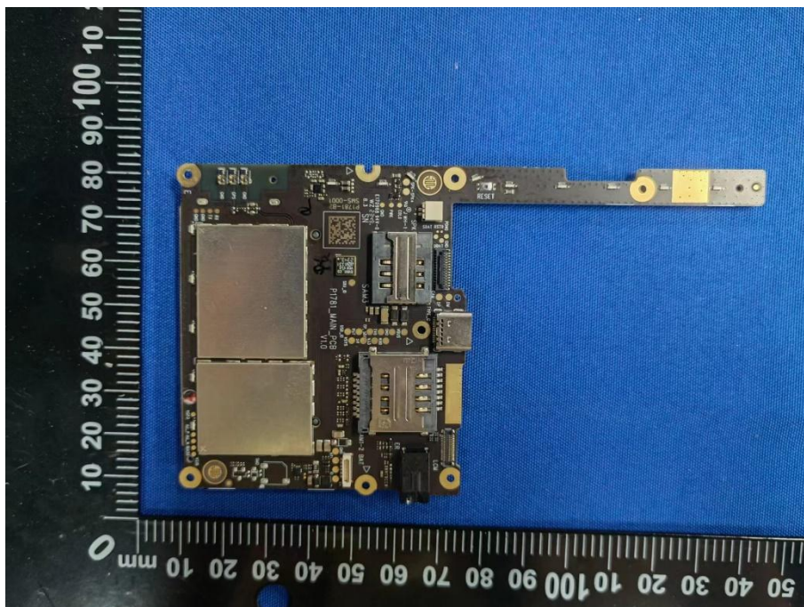
MAIN BOARD 1 TOP VIEW (WITH SHIELDING)
