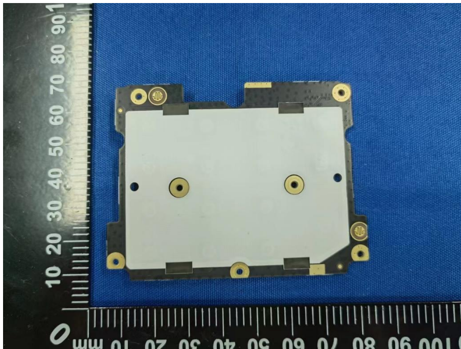
MAIN BOARD 2 TOP VIEW (WITH SHIELDING)
