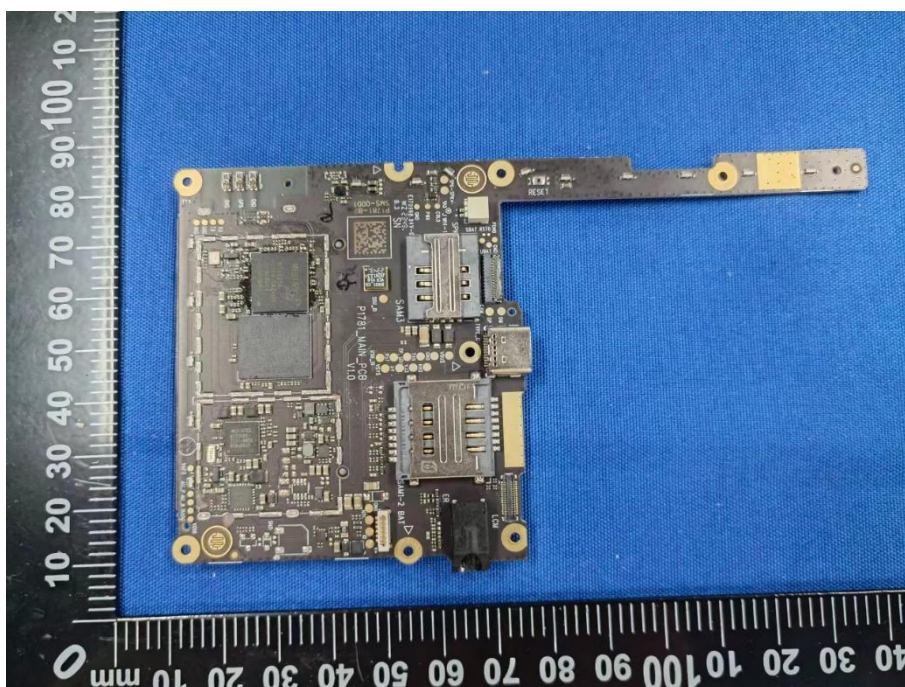
MAIN BOARD 1 TOP VIEW (WITHOUT SHIELDING)
