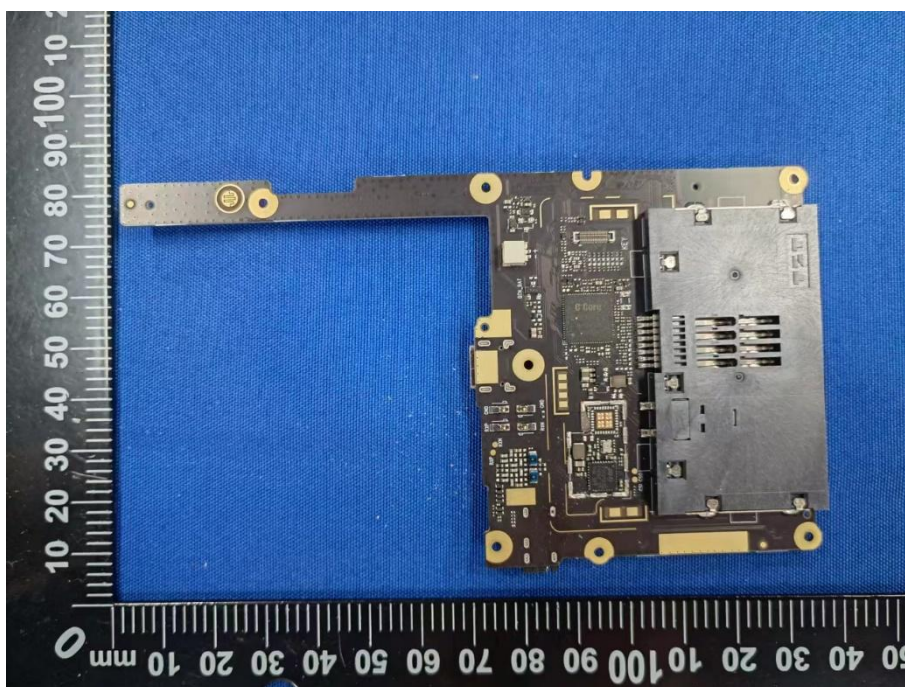
MAIN BOARD 1 REAR VIEW (WITHOUT SHIELDING)
