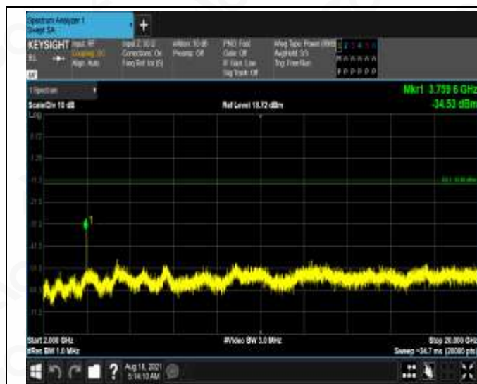
1.4MHz_HCH_QPSK_1RB#0
