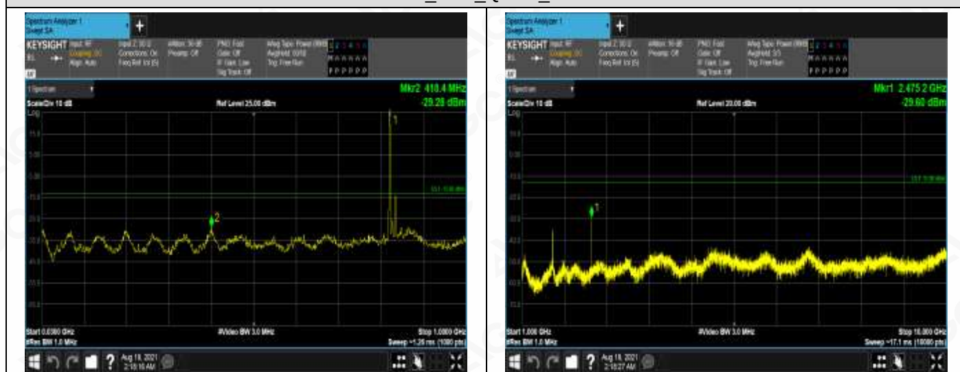
15MHz_MCH_QPSK_1RB#0
