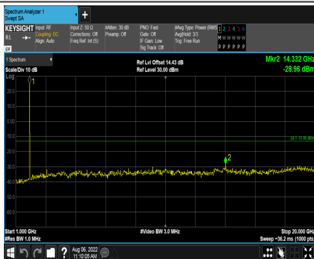
Band25-1.4MHz-16QAM-26365-1RB#0-Range2:1000~20000MHz
