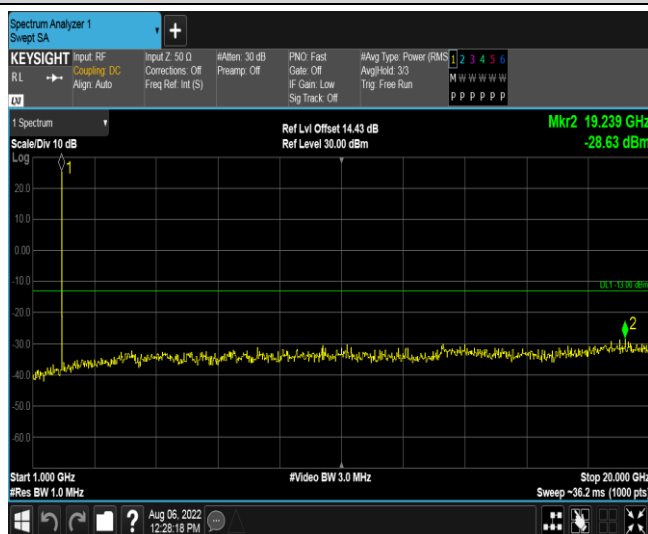
Band25-15MHz-16QAM-26615-1RB#0-Range2:1000~20000MHz
