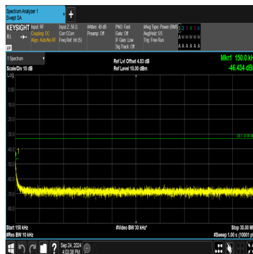
EGPRS1900-512-2-0.15~30MHz-PASS
