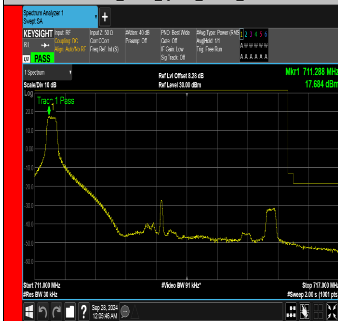
Band17_5MHz_QPSK_23825_1RB#0
