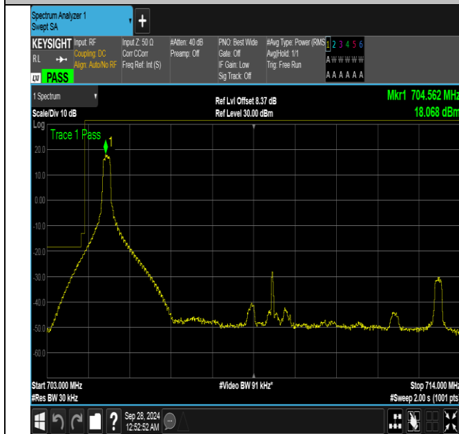
Band17_10MHz_QPSK_23780_1RB#0
