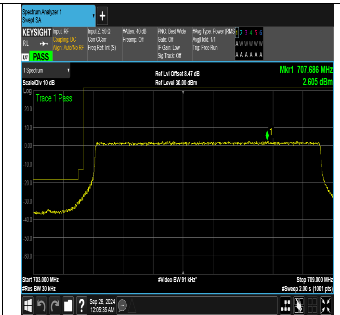
Band17_5MHz_16QAM_23755_25RB#0
