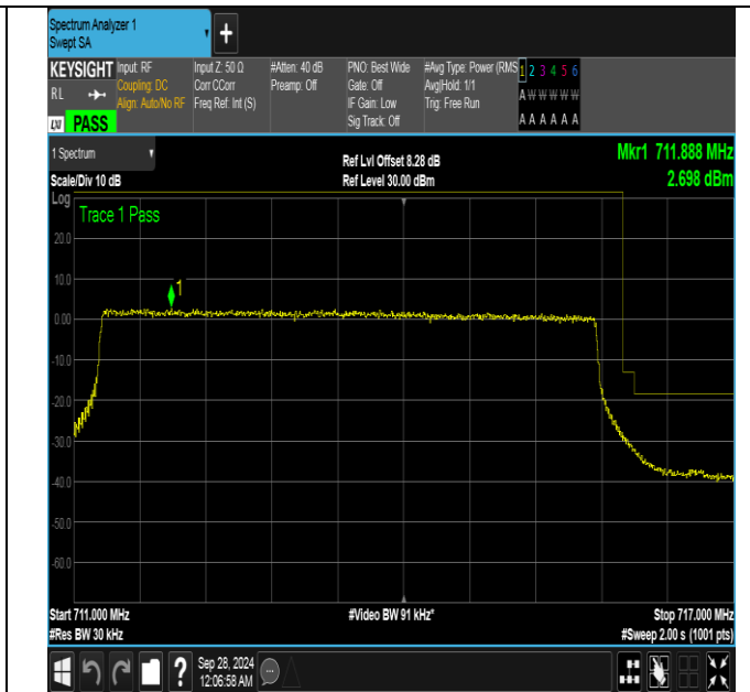
Band17_5MHz_16QAM_23825_25RB#0
