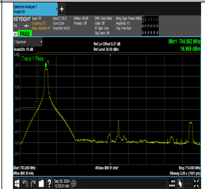
Band17_10MHz_16QAM_23780_1RB#0
