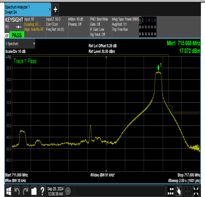
Band17_5MHz_16QAM_23825_1RB#24
