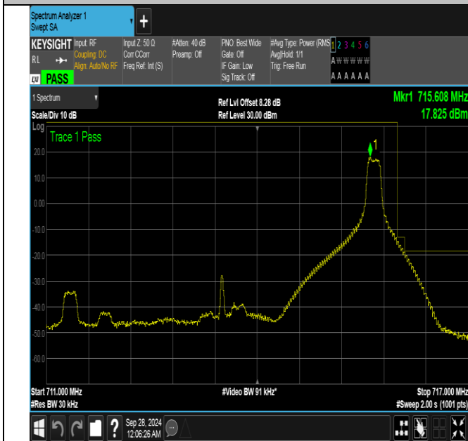
Band17_5MHz_QPSK_23825_1RB#24
