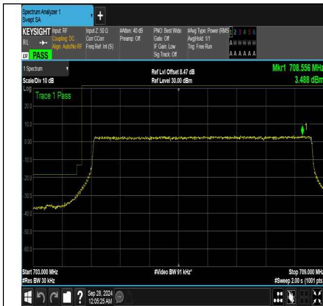
Band17_5MHz_QPSK_23755_25RB#0
