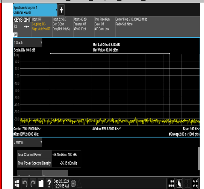
Band17_5MHz_QPSK_23825_1RB#0_Final1
