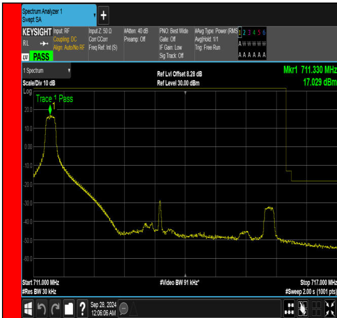
Band17_5MHz_16QAM_23825_1RB#0
