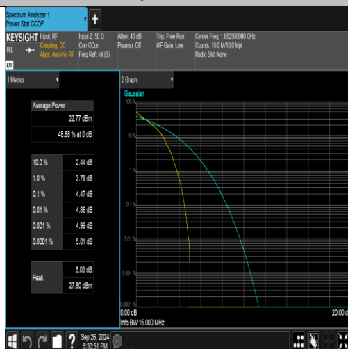
Band25-15MHz-QPSK-26365-1RB#0-PASS
