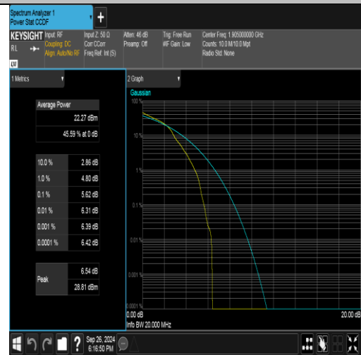
Band25-20MHz-16QAM-26590-1RB#0-PASS
