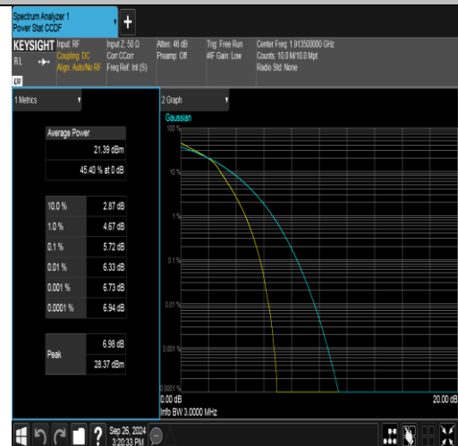
Band25-3MHz-16QAM-26675-15RB#0-PASS
