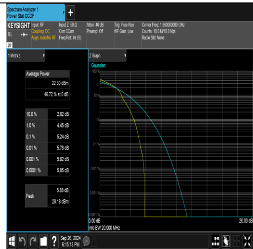
Band25-20MHz-16QAM-26140-1RB#0-PASS
