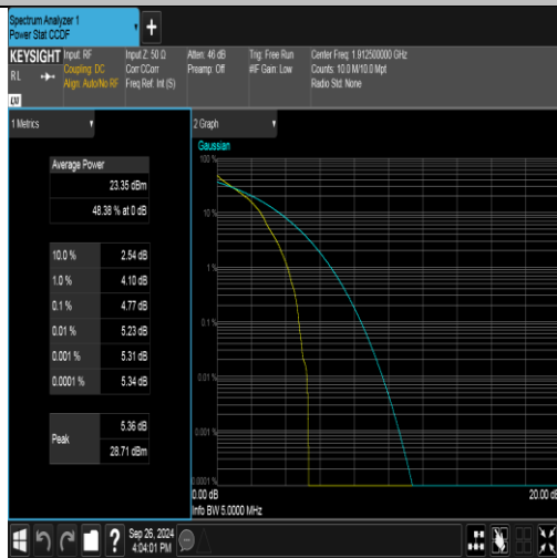
Band25-5MHz-QPSK-26665-1RB#0-PASS
