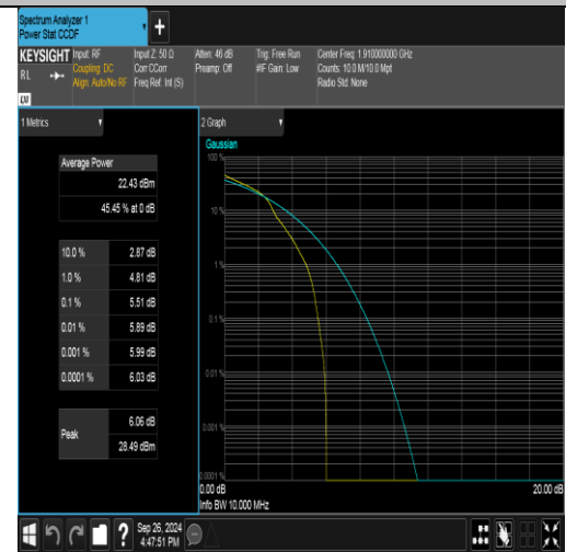
Band25-10MHz-16QAM-26640-1RB#0-PASS
