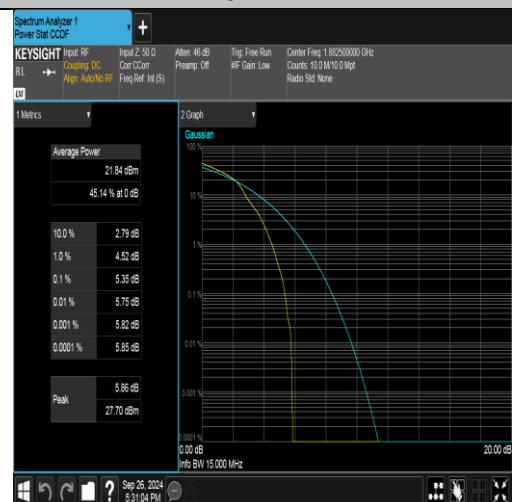
Band25-15MHz-16QAM-26365-1RB#0-PASS
