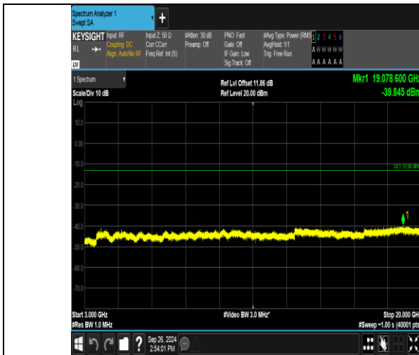
Band25_3MHz_QPSK_26675_1RB#0_3000~20000_3000~20000
