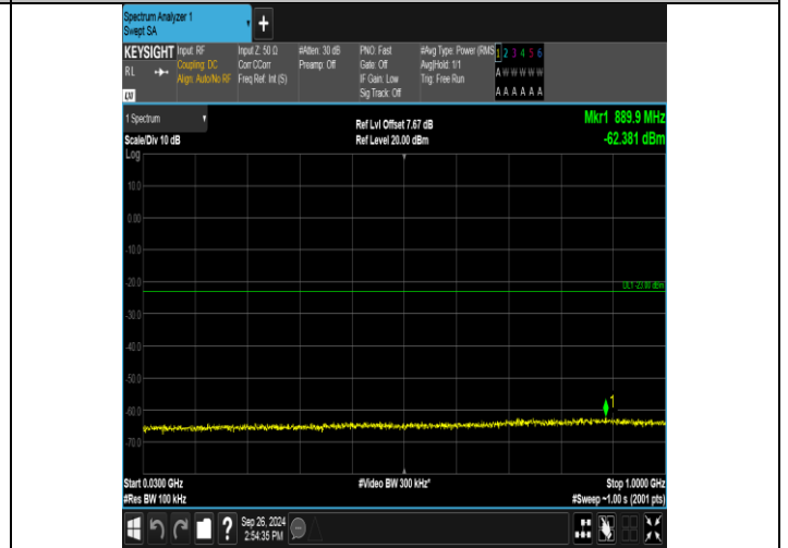
Band25_3MHz_16QAM_26675_1RB#0_30~1000_30~1000
