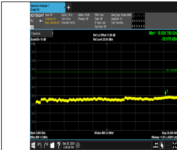
Band25_3MHz_QPSK_26365_1RB#0_3000~20000_3000~20000
