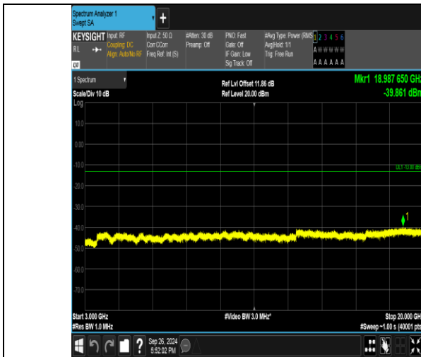
Band25_20MHz_QPSK_26590_1RB#0_3000~20000_3000~20000
