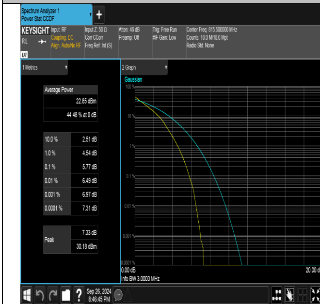
Band26(814-824)-3MHz-QPSK-26705-15RB#0-PASS
