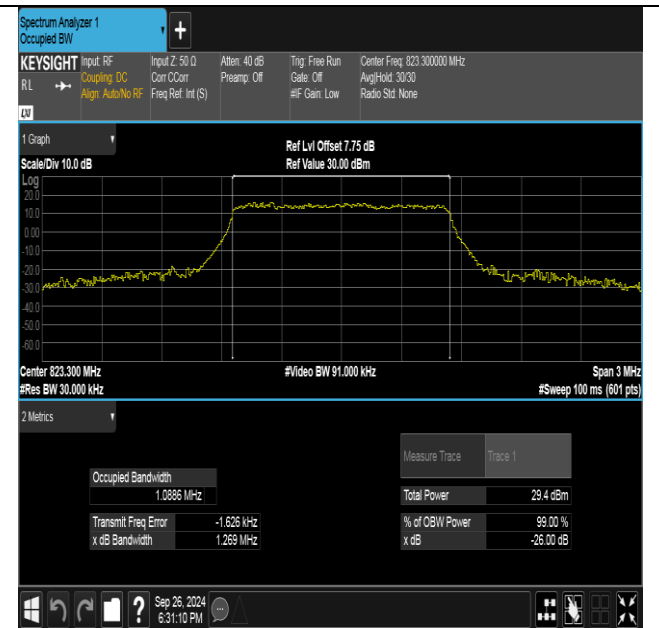
Band26(814-824)-1.4MHz-16QAM-26783-6RB#0-PASS
