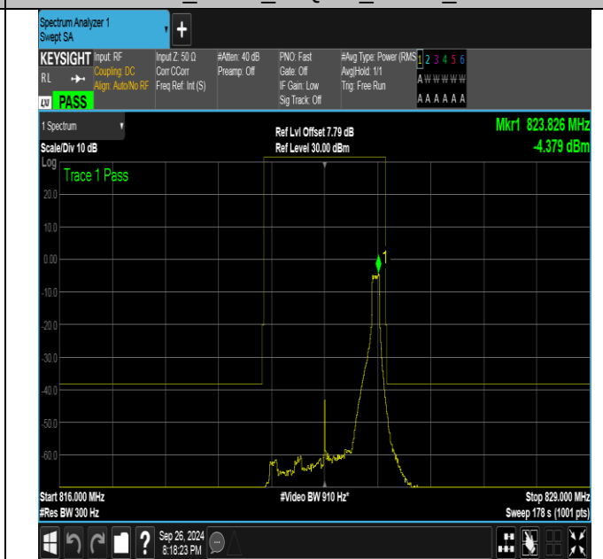
Band26_3MHz_16QAM_26775_1RB#14
