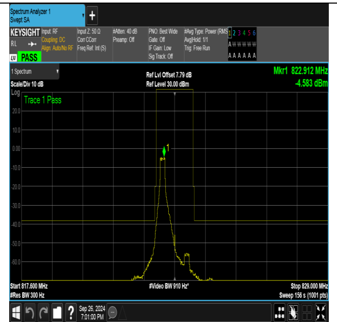
Band26_1.4MHz_16QAM_26783_1RB#0
