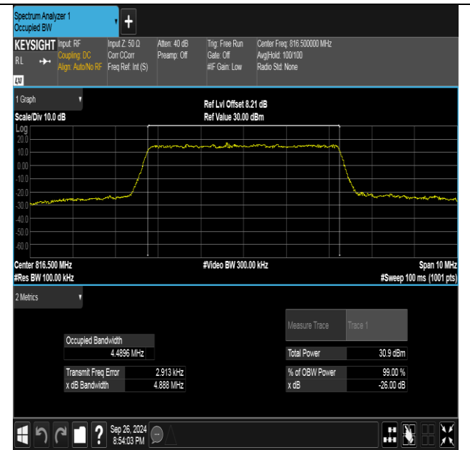
Band26(814-824)-5MHz-16QAM-26715-25RB#0-PASS
