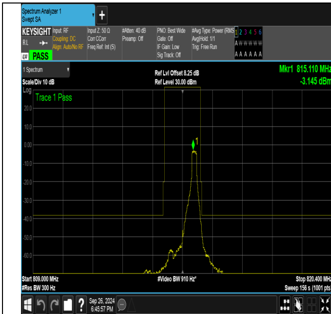
Band26_1.4MHz_QPSK_26697_1RB#5
