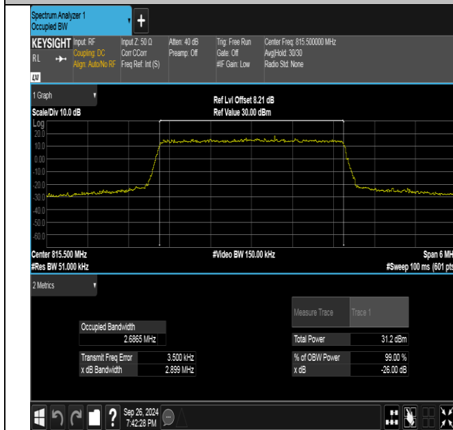
Band26(814-824)-3MHz-QPSK-26705-15RB#0-PASS
