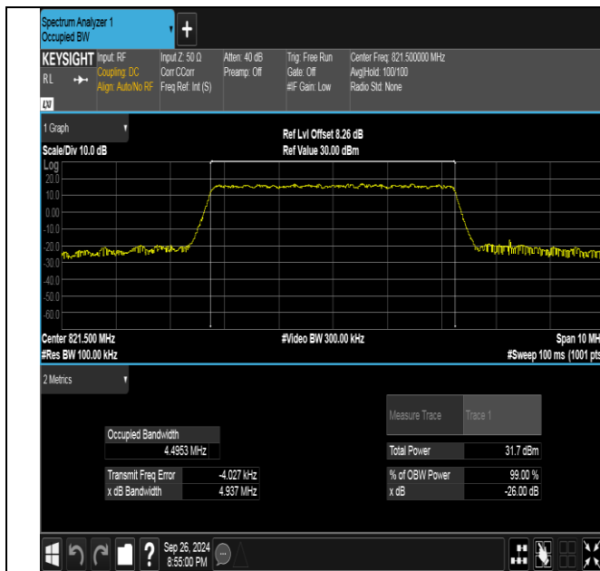
Band26(814-824)-5MHz-QPSK-26765-25RB#0-PASS
