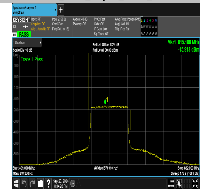
Band26_3MHz_16QAM_26705_15RB#0
