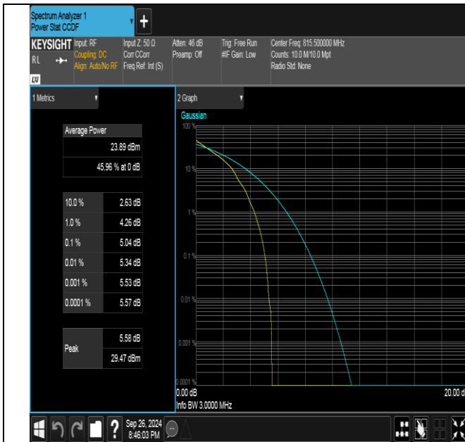
Band26(814-824)-3MHz-QPSK-26705-1RB#0-PASS
