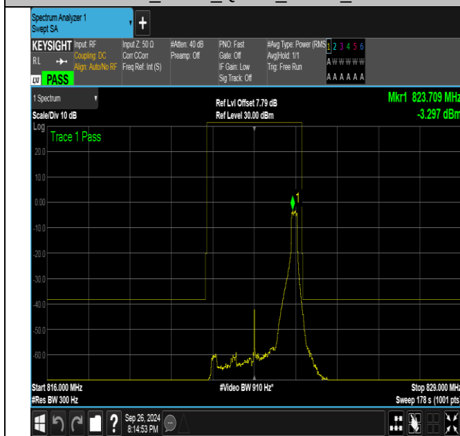
Band26_3MHz_QPSK_26775_1RB#14
