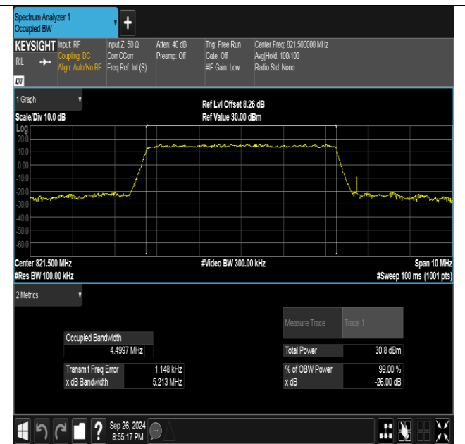
Band26(814-824)-5MHz-16QAM-26765-25RB#0-PASS
