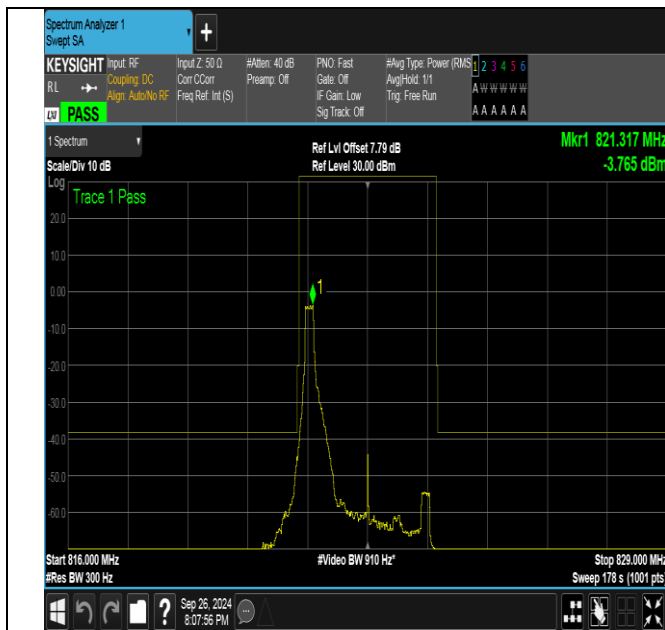
Band26_3MHz_QPSK_26775_1RB#0
