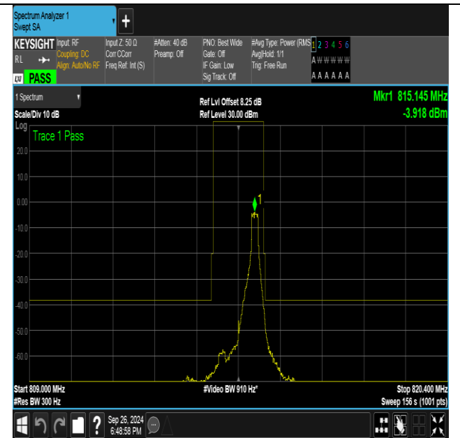
Band26_1.4MHz_16QAM_26697_1RB#5
