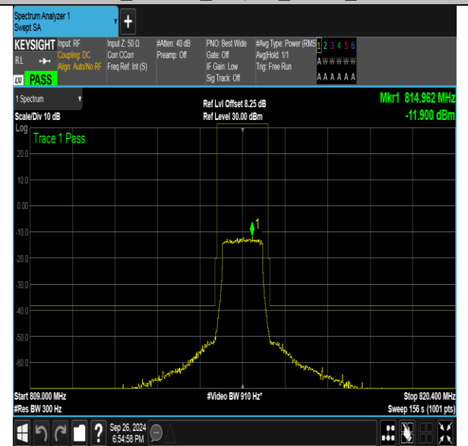
Band26_1.4MHz_16QAM_26697_6RB#0
