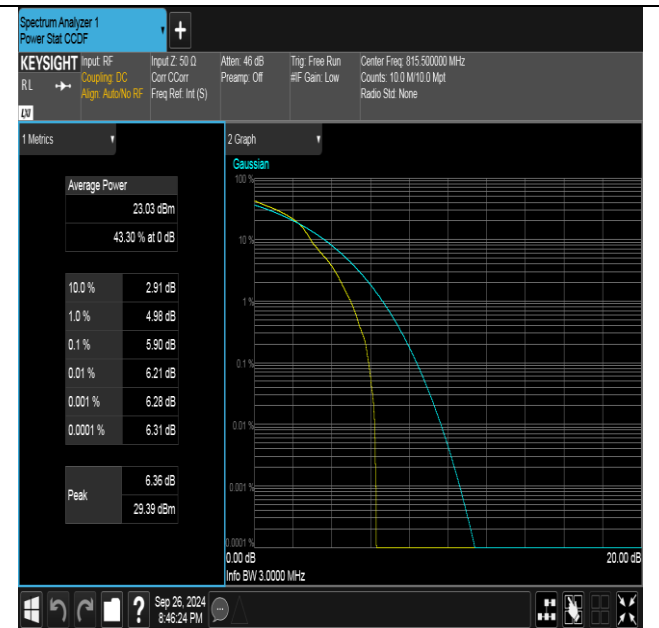
Band26(814-824)-3MHz-16QAM-26705-1RB#0-PASS
