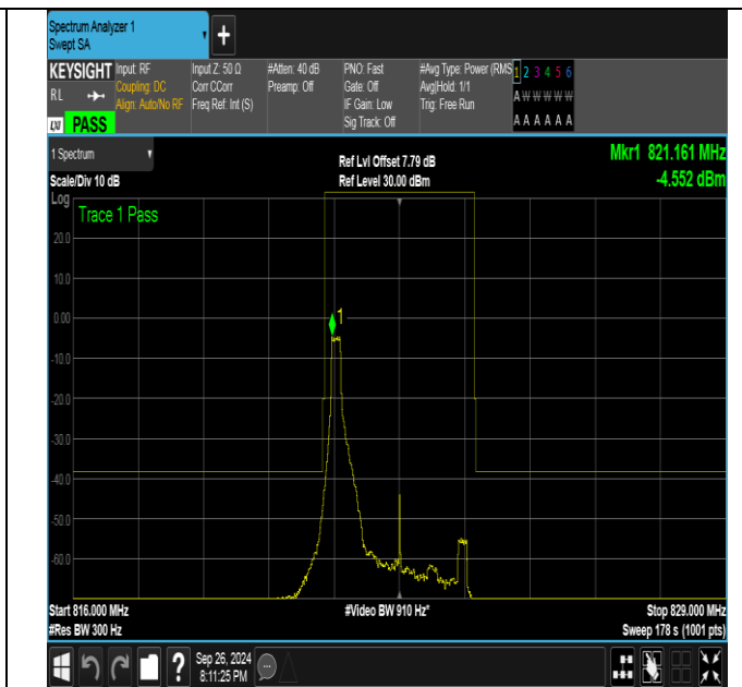
Band26_3MHz_16QAM_26775_1RB#0
