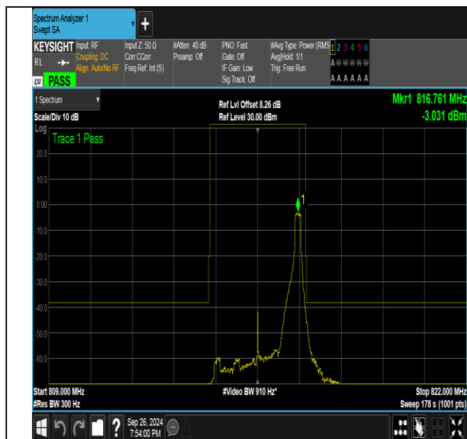
Band26_3MHz_QPSK_26705_1RB#14
