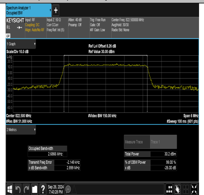
Band26(814-824)-3MHz-16QAM-26775-15RB#0-PASS
