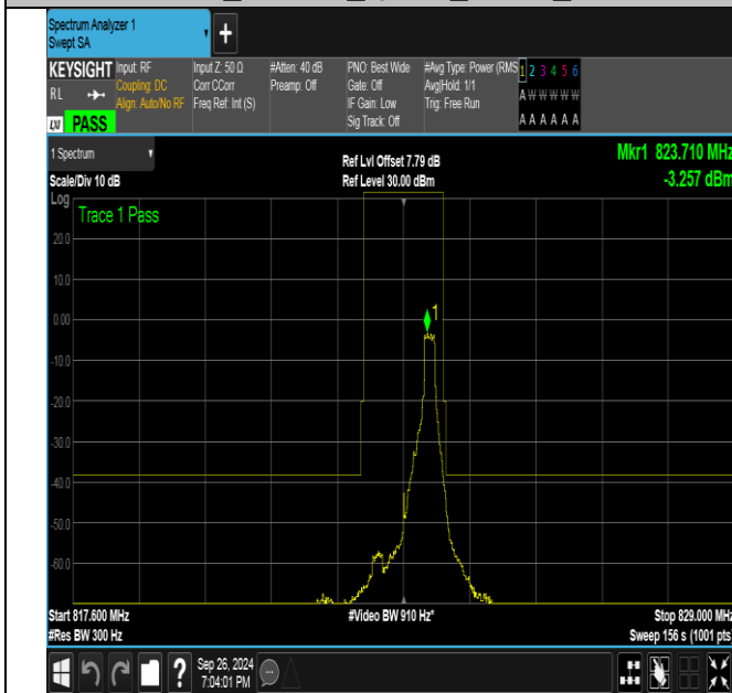
Band26_1.4MHz_QPSK_26783_1RB#5
