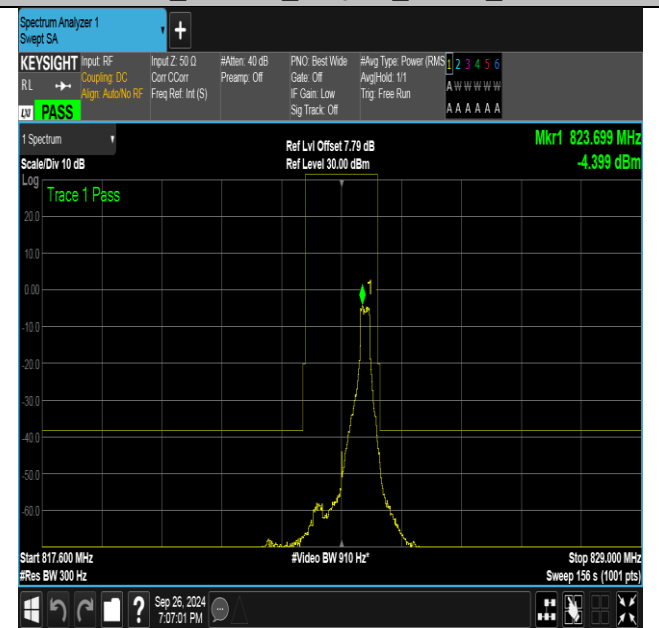
Band26_1.4MHz_16QAM_26783_1RB#5
