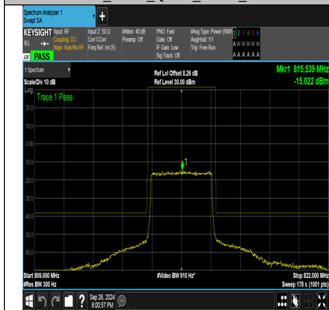
Band26_3MHz_QPSK_26705_15RB#0
