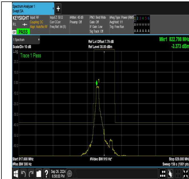
Band26_1.4MHz_QPSK_26783_1RB#0
