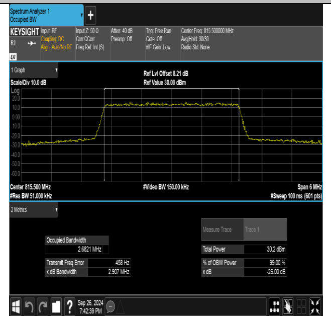
Band26(814-824)-3MHz-16QAM-26705-15RB#0-PASS
