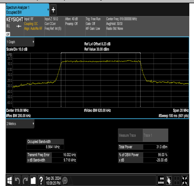
Band26(814-824)-10MHz-16QAM-26740-50RB#0-PASS
