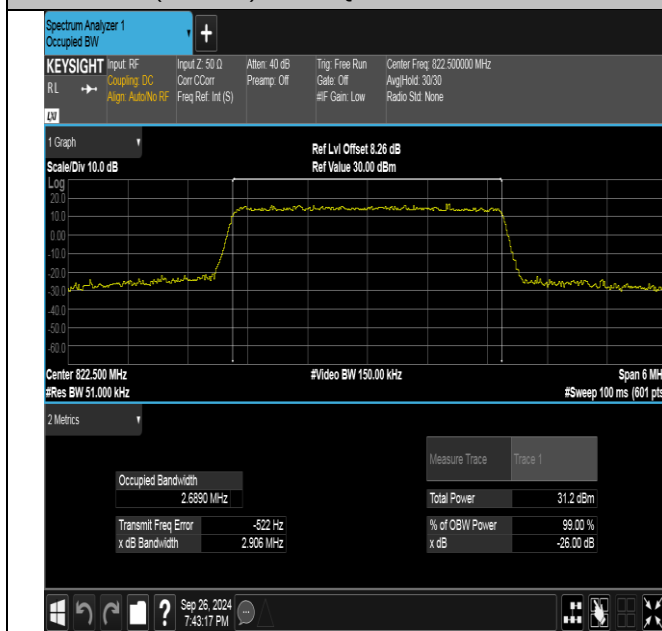
Band26(814-824)-3MHz-QPSK-26775-15RB#0-PASS
