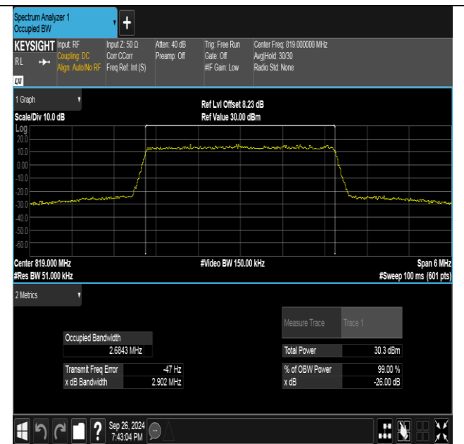
Band26(814-824)-3MHz-16QAM-26740-15RB#0-PASS
