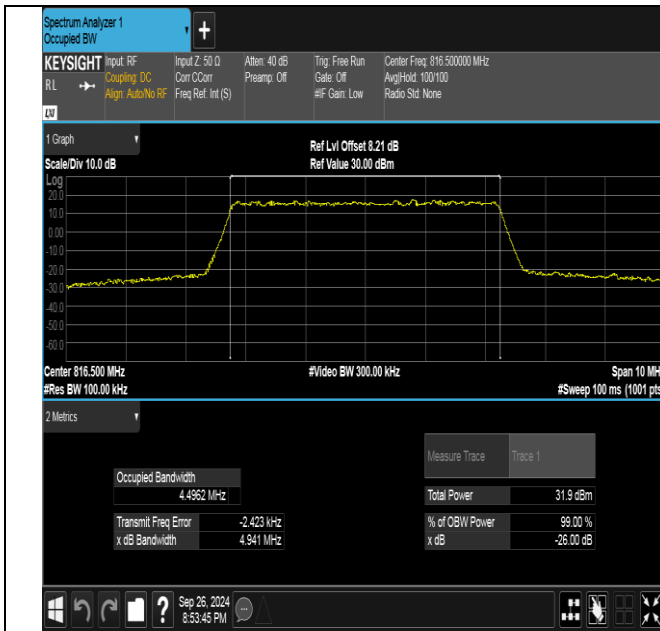
Band26(814-824)-5MHz-QPSK-26715-25RB#0-PASS
