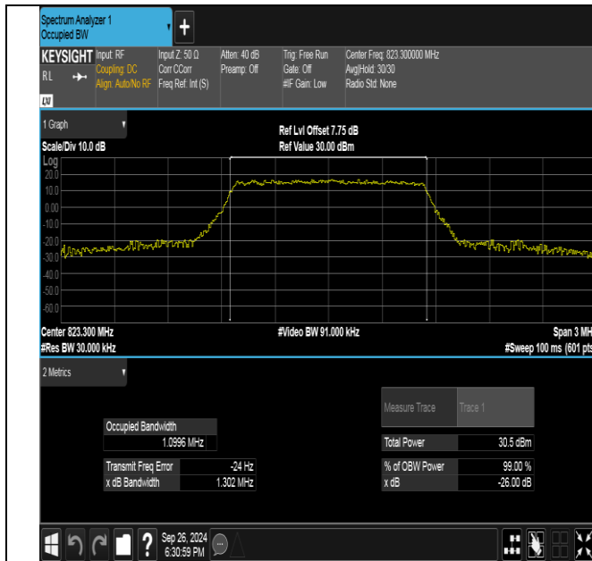
Band26(814-824)-1.4MHz-QPSK-26783-6RB#0-PASS
