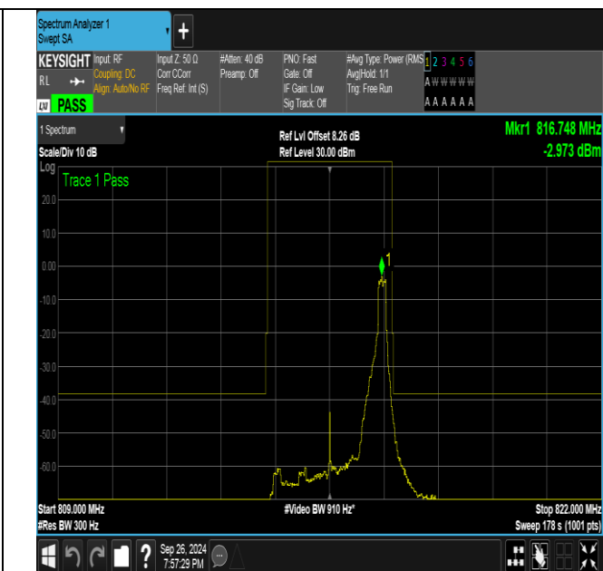
Band26_3MHz_16QAM_26705_1RB#14
