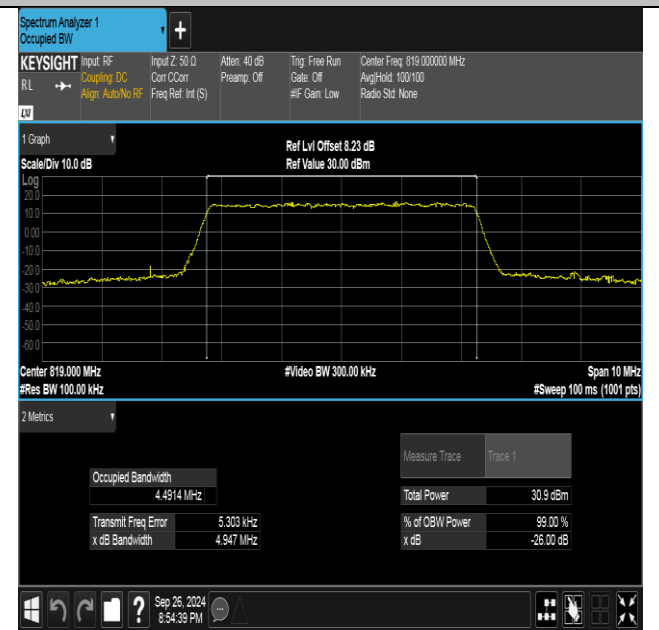
Band26(814-824)-5MHz-16QAM-26740-25RB#0-PASS
