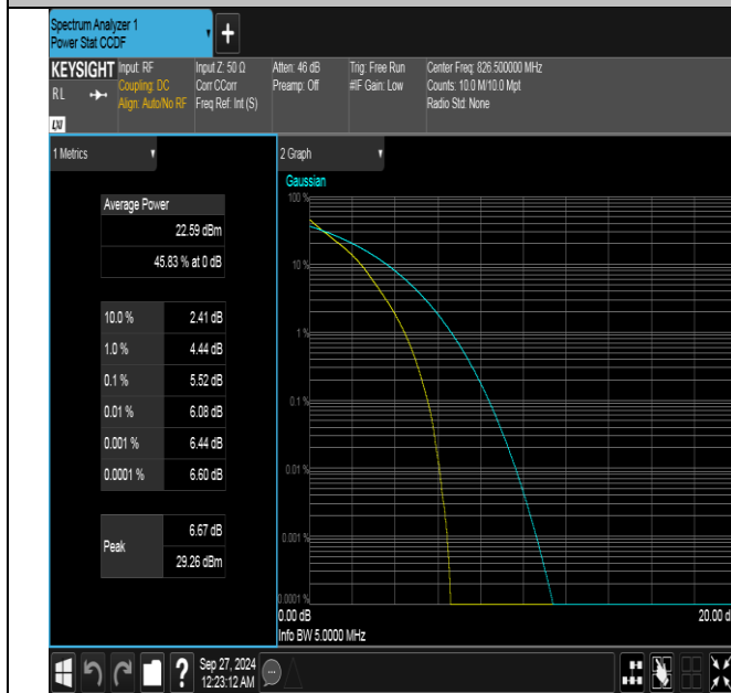
Band26(824-849)-5MHz-QPSK-26815-25RB#0-PASS
