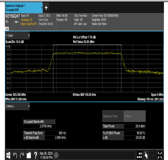
Band26(824-849)-3MHz-16QAM-26805-15RB#0-PASS
