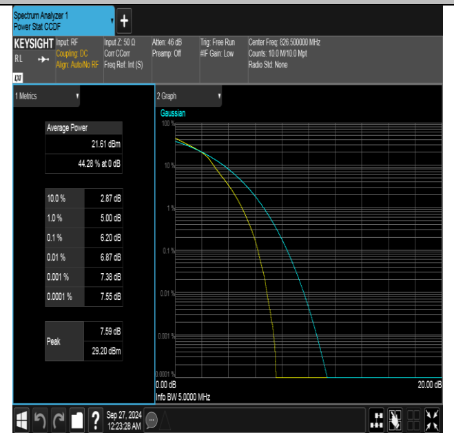
Band26(824-849)-5MHz-16QAM-26815-25RB#0-PASS
