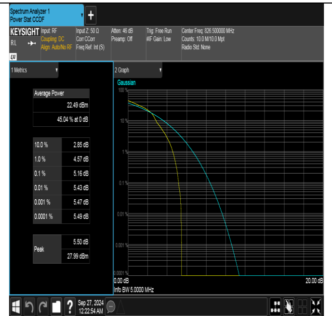
Band26(824-849)-5MHz-16QAM-26815-1RB#0-PASS
