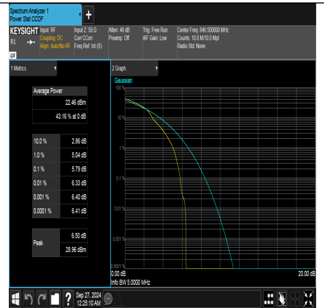
Band26(824-849)-5MHz-16QAM-27015-1RB#0-PASS
