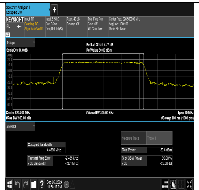
Band26(824-849)-5MHz-16QAM-26815-25RB#0-PASS
