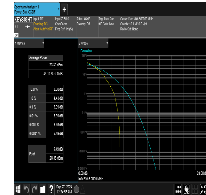
Band26(824-849)-5MHz-QPSK-27015-1RB#0-PASS
