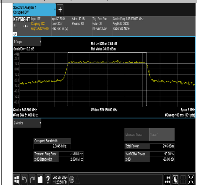
Band26(824-849)-3MHz-16QAM-27025-15RB#0-PASS
