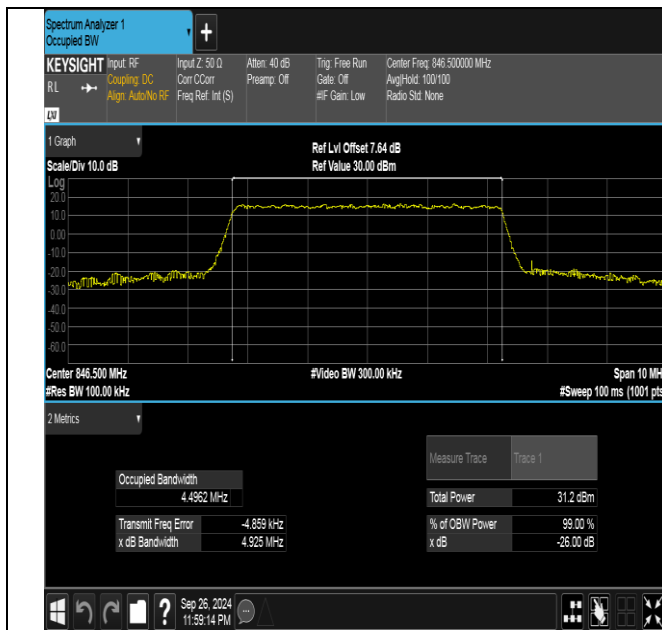
Band26(824-849)-5MHz-QPSK-27015-25RB#0-PASS
