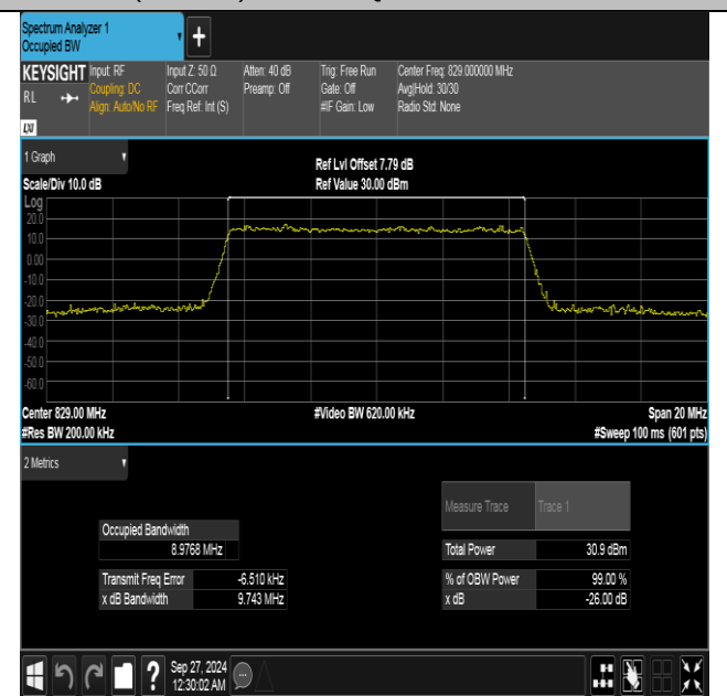
Band26(824-849)-10MHz-16QAM-26840-50RB#0-PASS
