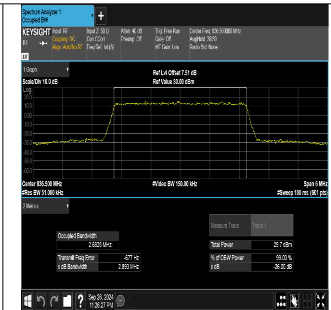
Band26(824-849)-3MHz-16QAM-26915-15RB#0-PASS
