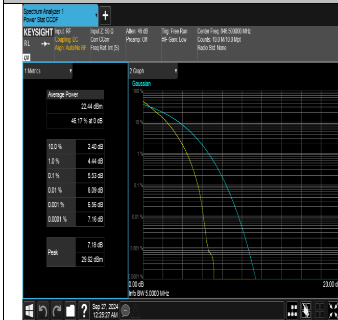
Band26(824-849)-5MHz-QPSK-27015-25RB#0-PASS
