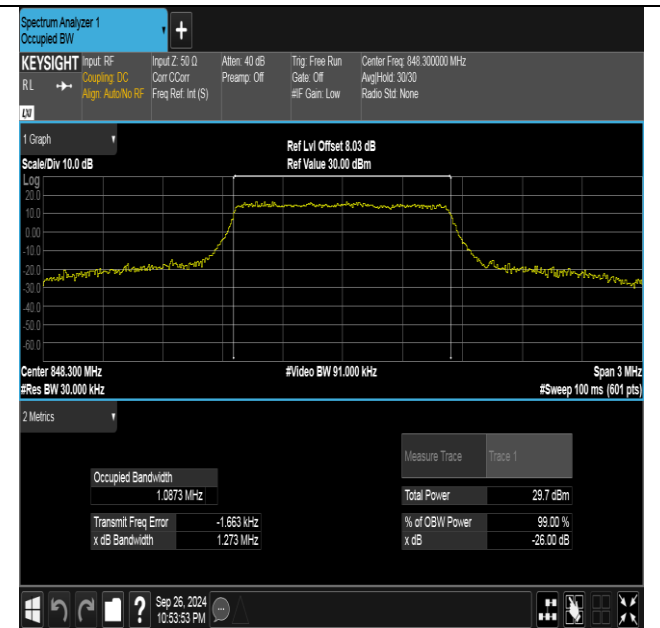
Band26(824-849)-1.4MHz-16QAM-27033-6RB#0-PASS
