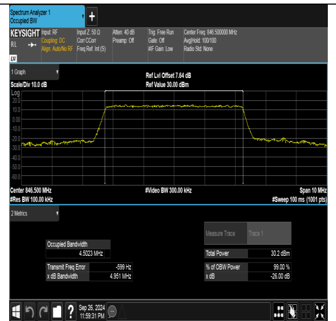
Band26(824-849)-5MHz-16QAM-27015-25RB#0-PASS
