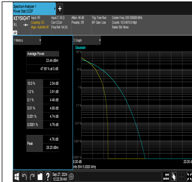
Band26(824-849)-5MHz-QPSK-26815-1RB#0-PASS
