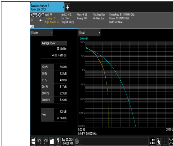
Band4-1.4MHz-QPSK-19957-1RB#0-PASS
