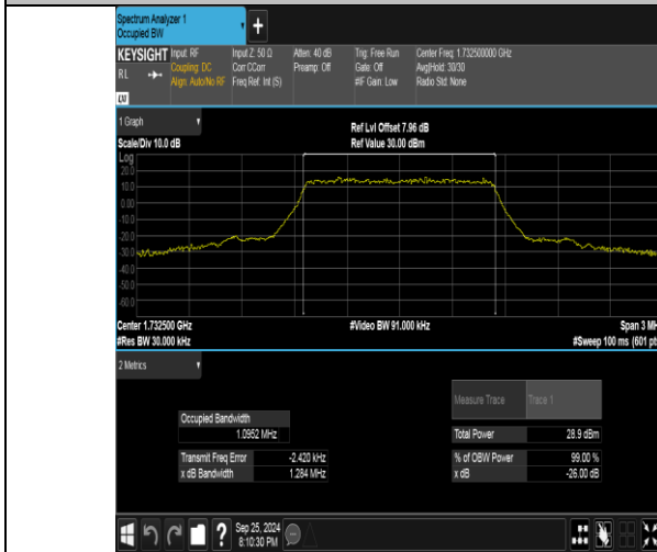
Band4-1.4MHz-QPSK-20175-6RB#0-PASS
