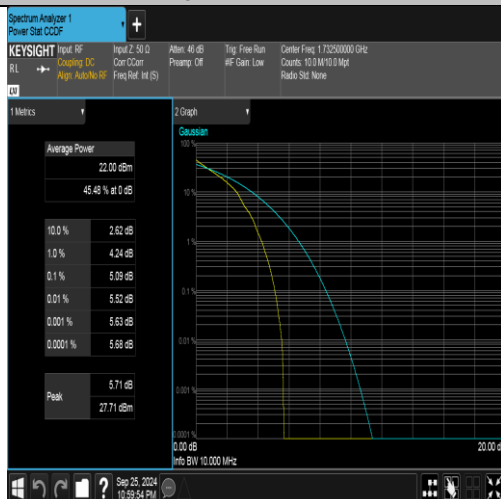
Band4-10MHz-QPSK-20175-1RB#0-PASS
