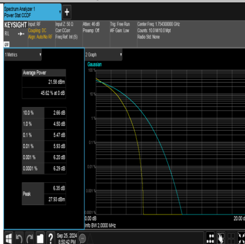
Band4-1.4MHz-QPSK-20393-6RB#0-PASS
