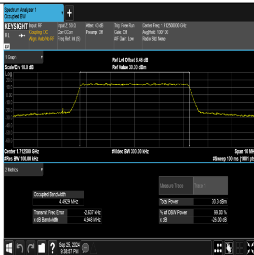
Band4-5MHz-QPSK-19975-25RB#0-PASS
