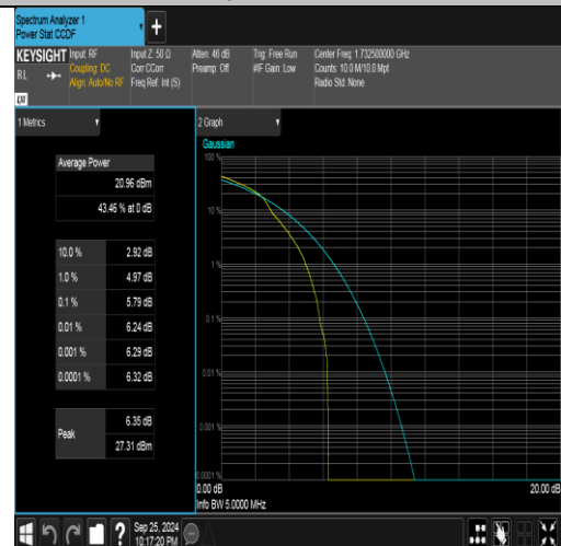
Band4-5MHz-16QAM-20175-1RB#0-PASS
