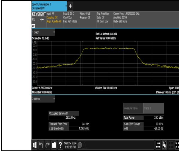
Band4-1.4MHz-QPSK-19957-6RB#0-PASS
