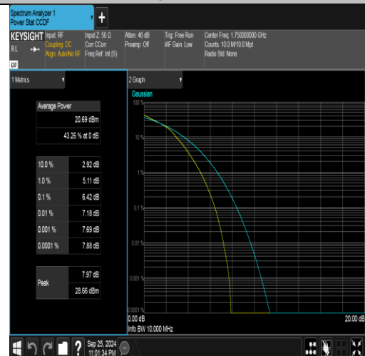
Band4-10MHz-16QAM-20350-50RB#0-PASS
