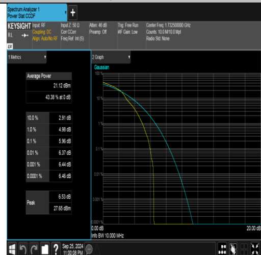
Band4-10MHz-16QAM-20175-1RB#0-PASS
