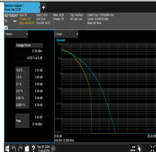
Band4-15MHz-16QAM-20175-1RB#0-PASS
