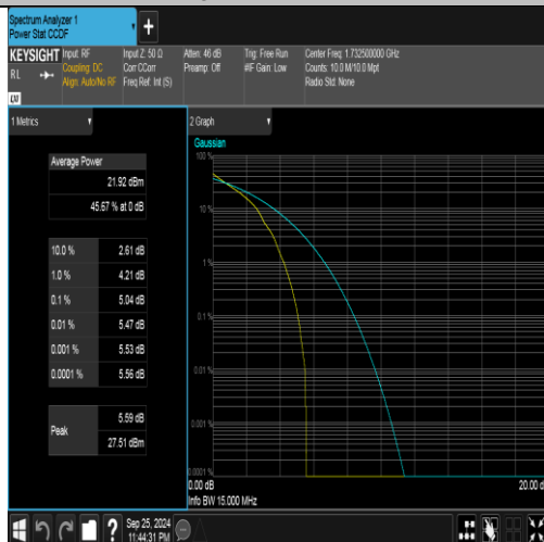
Band4-15MHz-QPSK-20175-1RB#0-PASS
