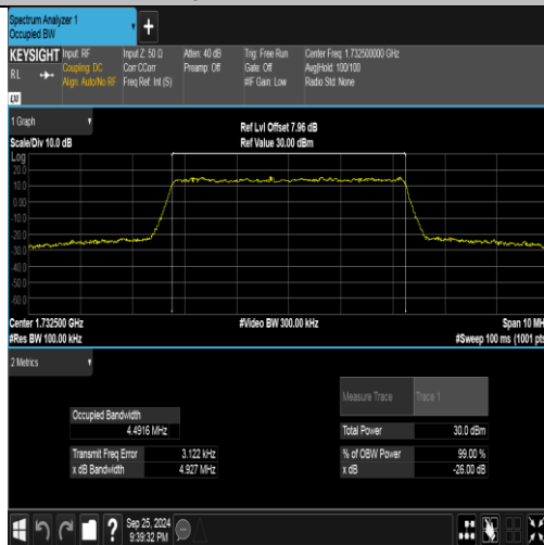
Band4-5MHz-QPSK-20175-25RB#0-PASS
