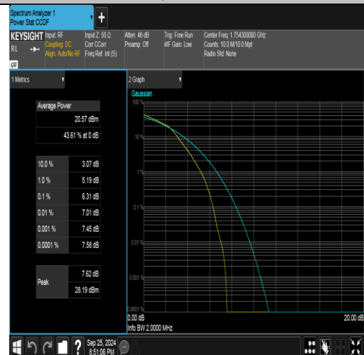
Band4-1.4MHz-16QAM-20393-6RB#0-PASS
