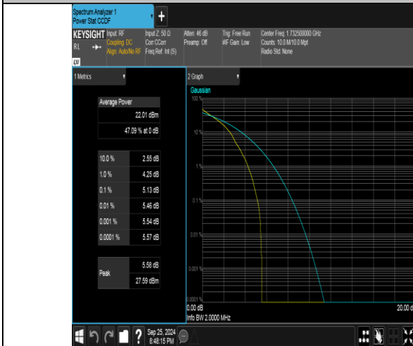
Band4-1.4MHz-QPSK-20175-1RB#0-PASS
