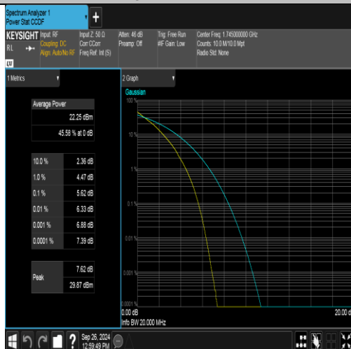
Band4-20MHz-QPSK-20300-100RB#0-PASS
