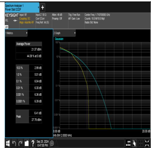
Band4-1.4MHz-16QAM-19957-1RB#0-PASS
