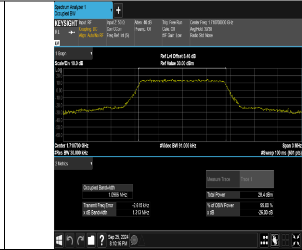
Band4-1.4MHz-16QAM-19957-6RB#0-PASS
