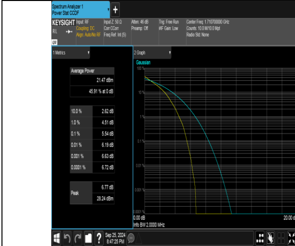
Band4-1.4MHz-QPSK-19957-6RB#0-PASS
