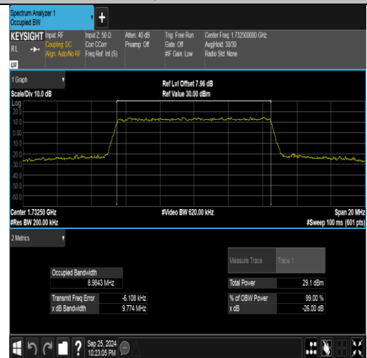
Band4-10MHz-16QAM-20175-50RB#0-PASS
