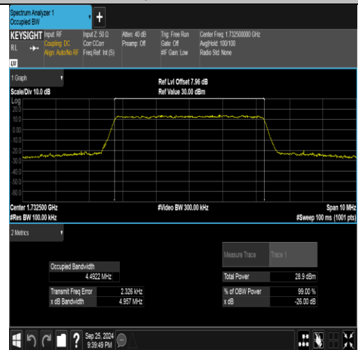
Band4-5MHz-16QAM-20175-25RB#0-PASS
