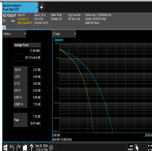
Band4-10MHz-QPSK-20350-50RB#0-PASS
