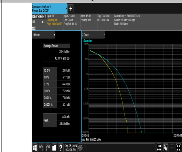
Band4-3MHz-16QAM-19965-15RB#0-PASS
