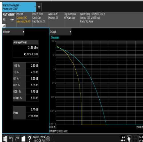
Band4-5MHz-QPSK-20175-1RB#0-PASS
