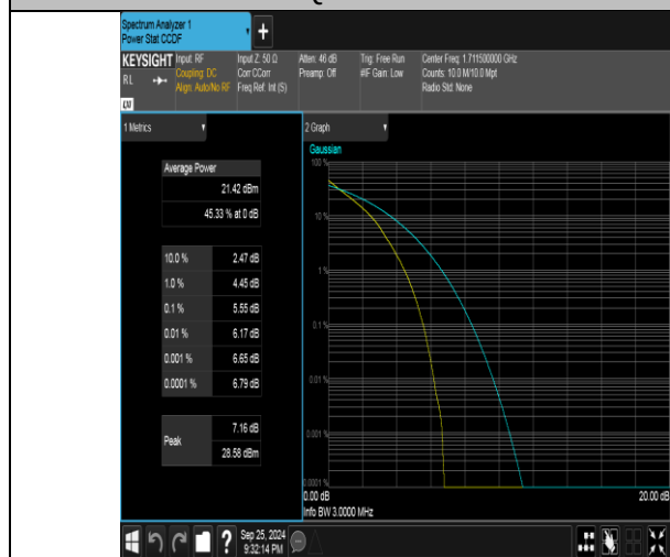
Band4-3MHz-QPSK-19965-15RB#0-PASS
