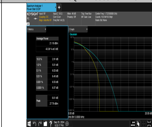
Band4-3MHz-16QAM-20175-1RB#0-PASS
