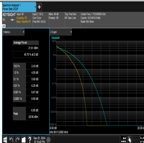
Band4-5MHz-QPSK-20375-25RB#0-PASS
