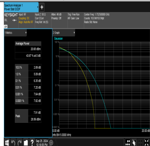
Band4-5MHz-16QAM-20375-25RB#0-PASS
