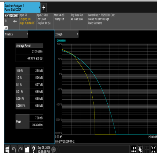
Band4-20MHz-16QAM-20175-1RB#0-PASS
