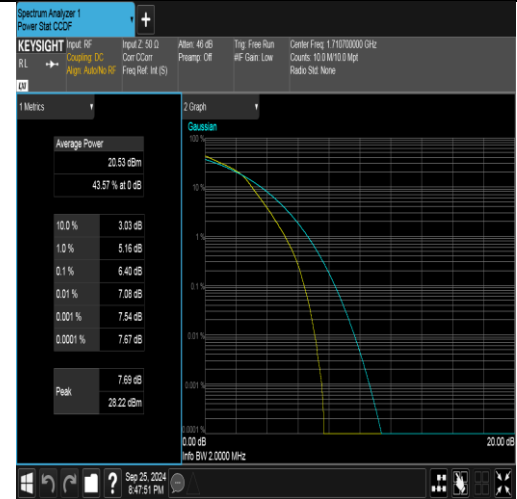
Band4-1.4MHz-16QAM-19957-6RB#0-PASS
