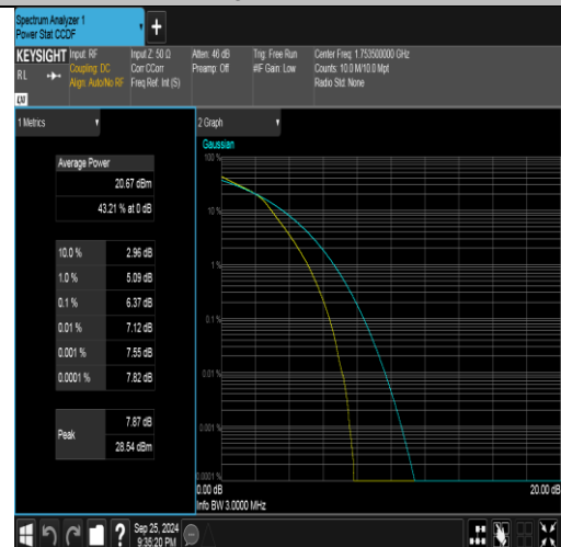
Band4-3MHz-16QAM-20385-15RB#0-PASS
