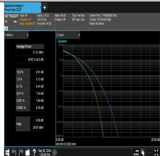
Band4-20MHz-16QAM-20300-100RB#0-PASS
