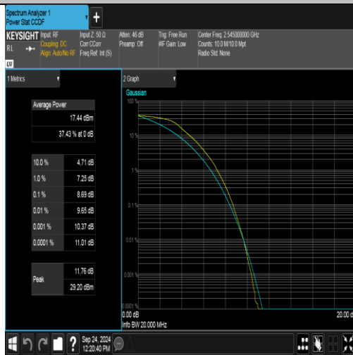
Band41(2535-2655)-20MHz-QPSK-40140-100RB#0-PASS
