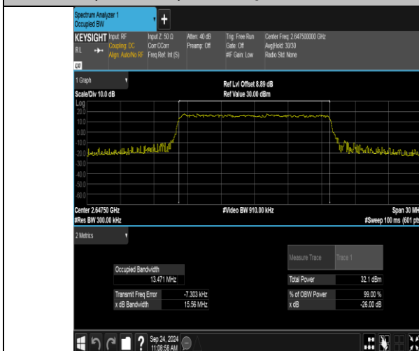
Band41(2535-2655)-15MHz-QPSK-41165-75RB#0-PASS
