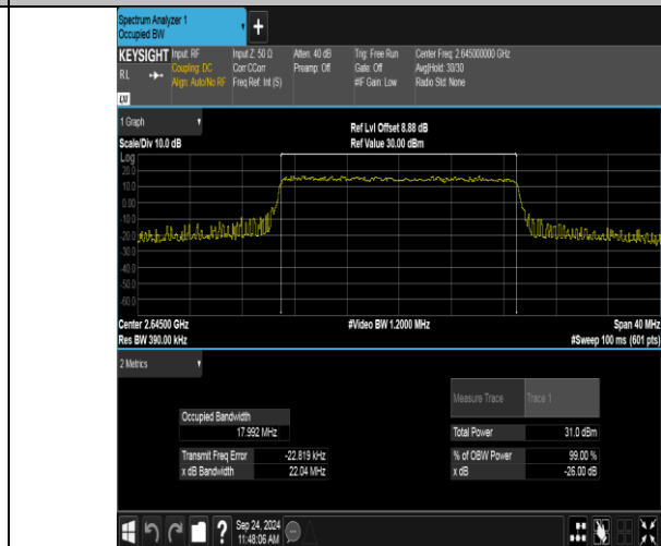
Band41(2535-2655)-20MHz-16QAM-41140-100RB#0-PASS
