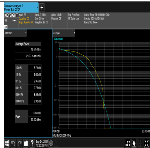
Band41(2535-2655)-20MHz-16QAM-40140-1RB#0-PASS
