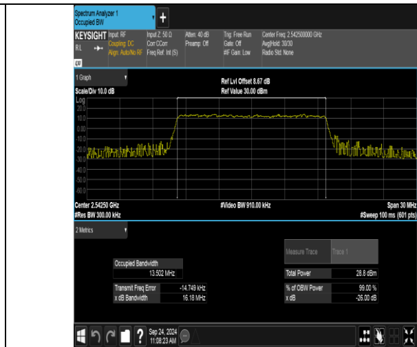
Band41(2535-2655)-15MHz-16QAM-40115-75RB#0-PASS
