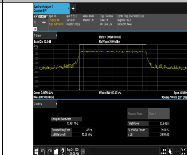
Band41(2535-2655)-15MHz-16QAM-41165-75RB#0-PASS
