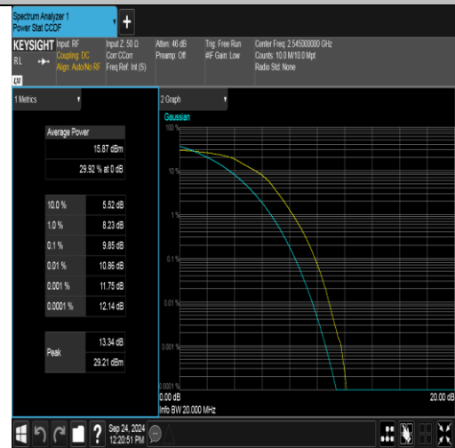
Band41(2535-2655)-20MHz-16QAM-40140-100RB#0-PASS
