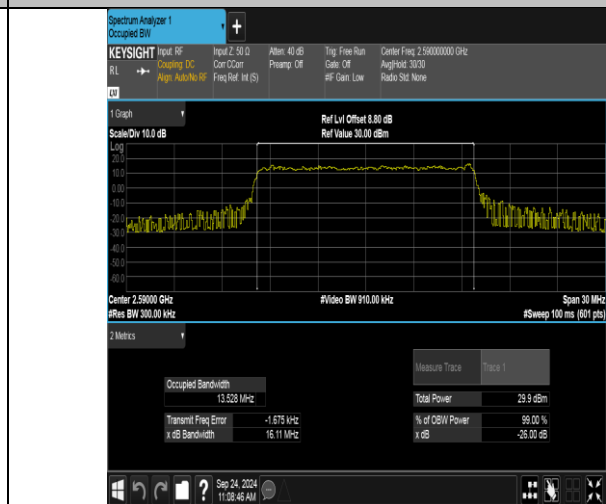
Band41(2535-2655)-15MHz-16QAM-40590-75RB#0-PASS
