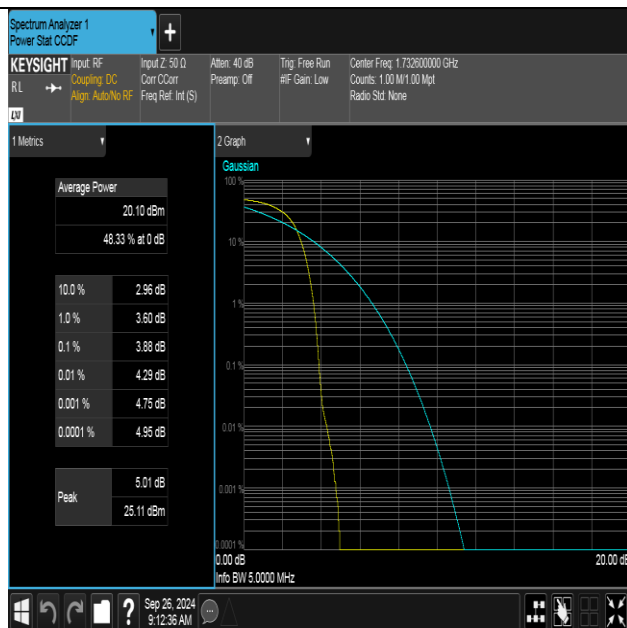
Band4-1413-4-PASS
