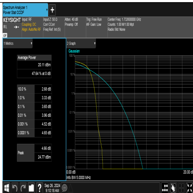
Band4-1413-2-PASS
