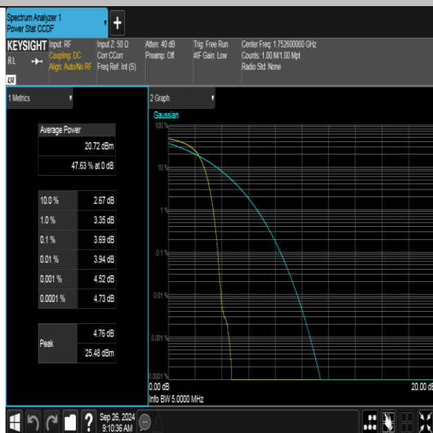
Band4-1513-2-PASS
