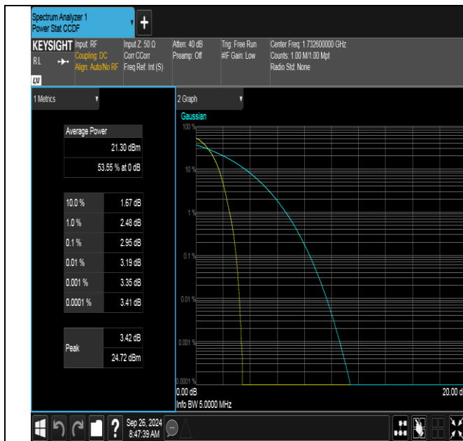
Band4-1413-PASS
