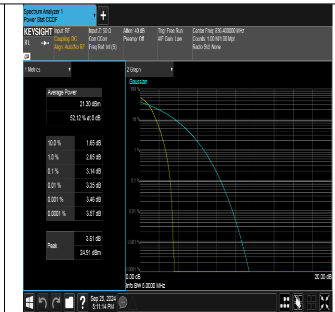
Band5-4182-PASS
