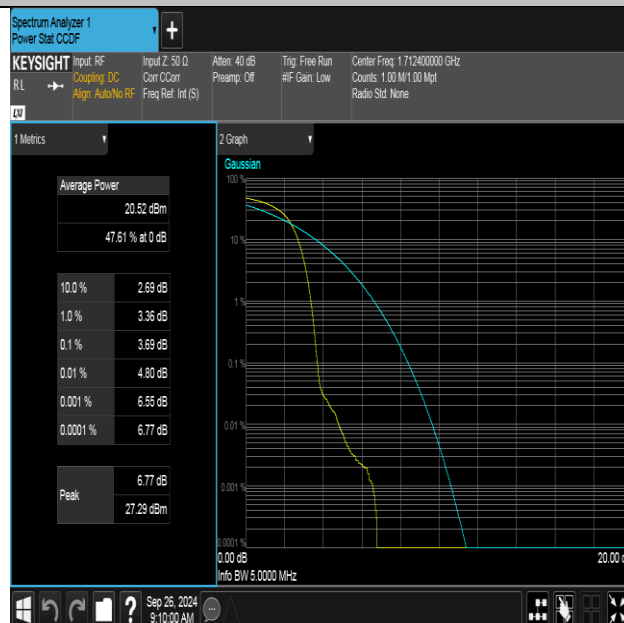
Band4-1312-2-PASS
