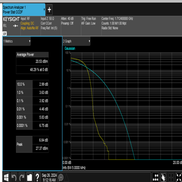
Band4-1312-4-PASS
