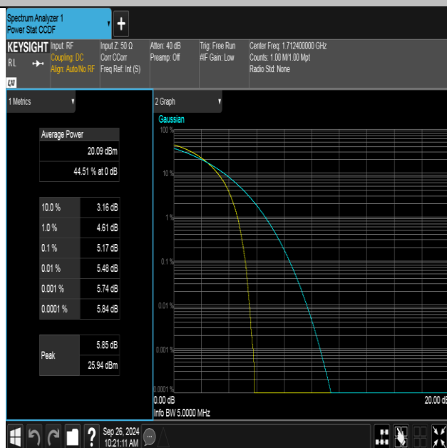
Band4-1312-3-PASS
