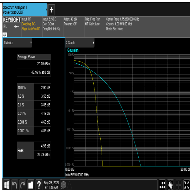
Band4-1513-3-PASS
