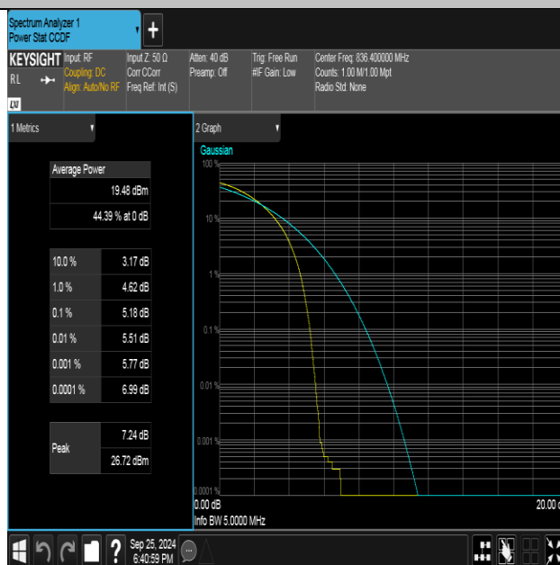
Band5-4182-3-PASS
