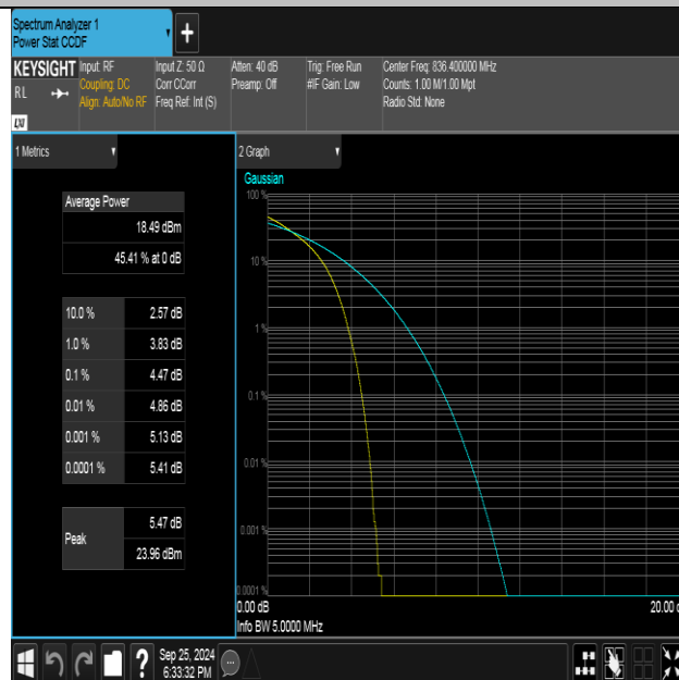
Band5-4182-1-PASS
