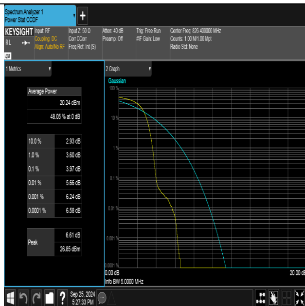
Band5-4132-3-PASS
