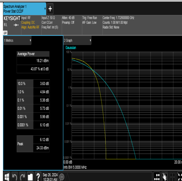
Band4-1413-4-PASS
