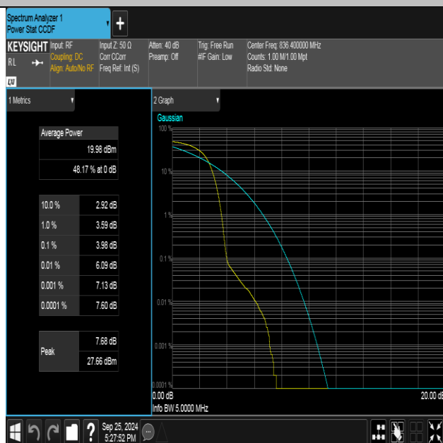
Band5-4182-3-PASS
