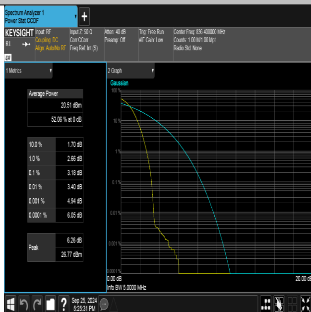
Band5-4182-1-PASS
