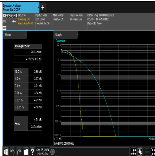
Band2-9400-2-PASS
