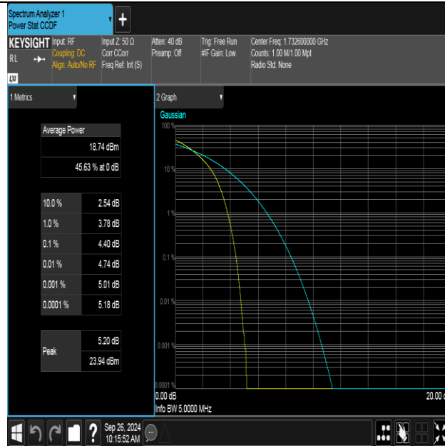
Band4-1413-1-PASS
