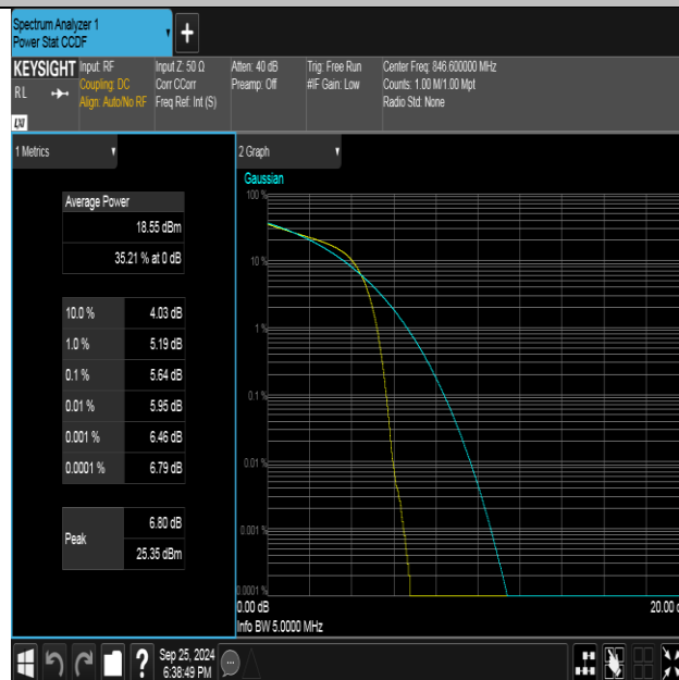
Band5-4233-2-PASS
