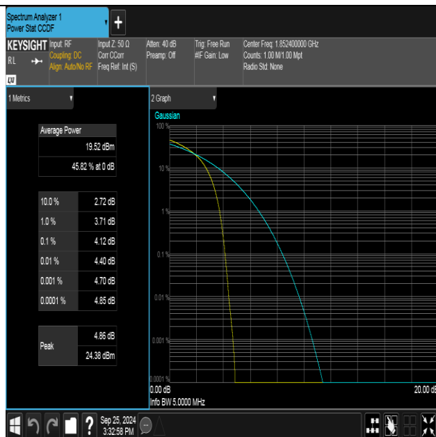
Band2-9262-5-PASS
