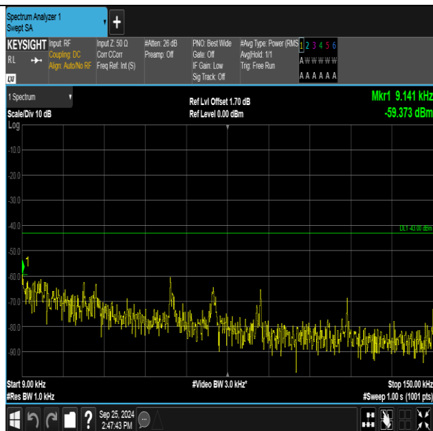
Band2-9400-3-0.009~0.15MHz-PASS
