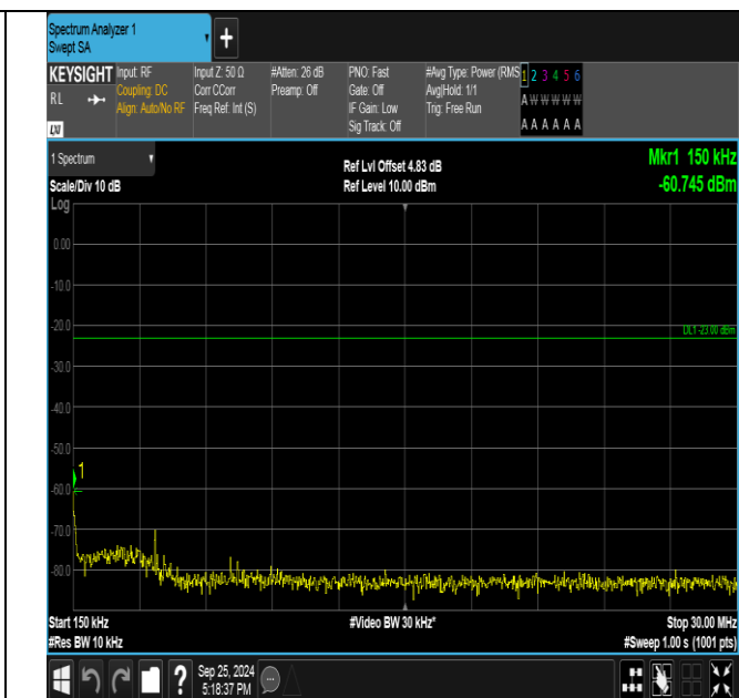
Band5-4182-0.15~30MHz-PASS
