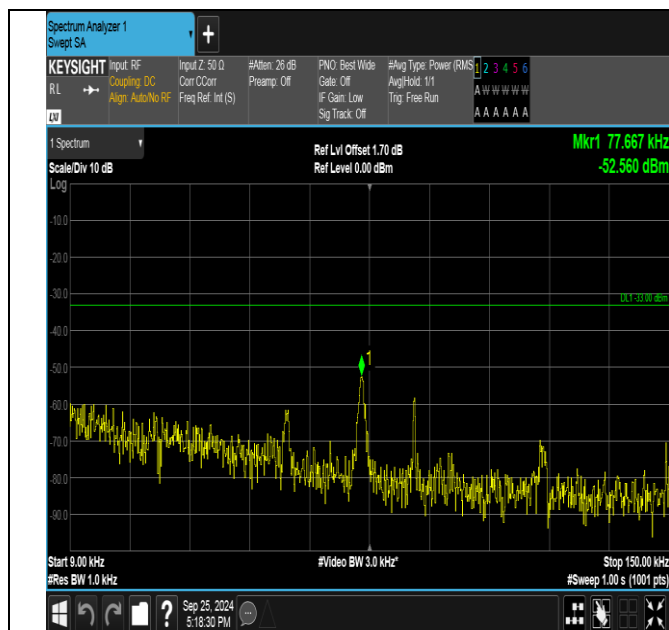
Band5-4182-0.009~0.15MHz-PASS
