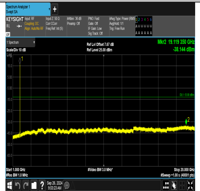
Band4-1513-1000~20000MHz-PASS
