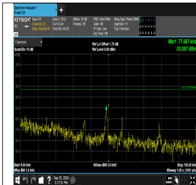
Band5-4132-0.009~0.15MHz-PASS
