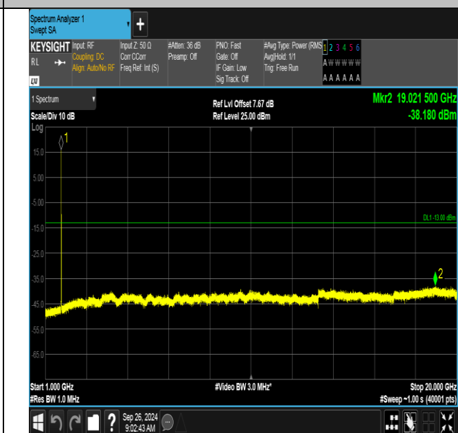
Band4-1413-1000~20000MHz-PASS
