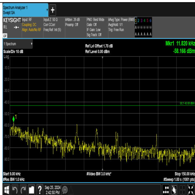
Band2-9262-1-0.009~0.15MHz-PASS
