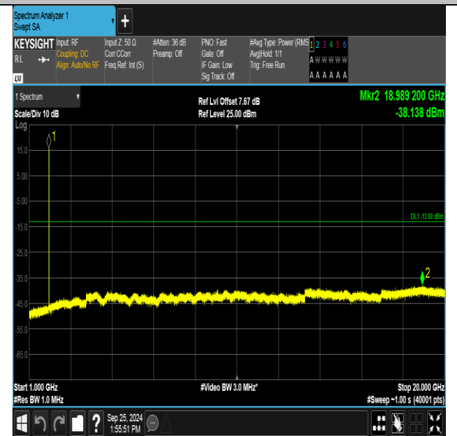
Band2-9538-1000~20000MHz-PASS
