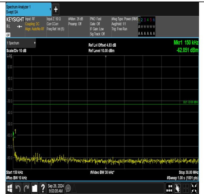
Band4-1513-0.15~30MHz-PASS
