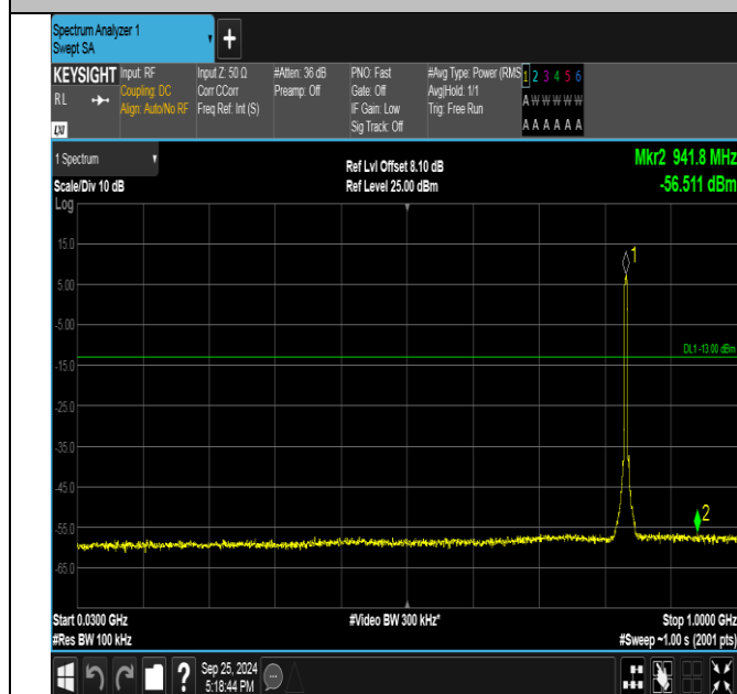
Band5-4182-30~1000MHz-PASS
