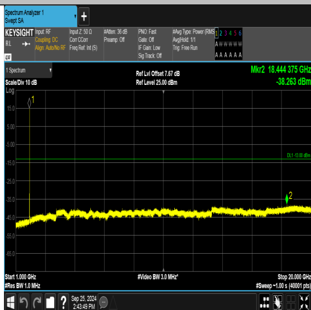
Band2-9400-1-1000~20000MHz-PASS
