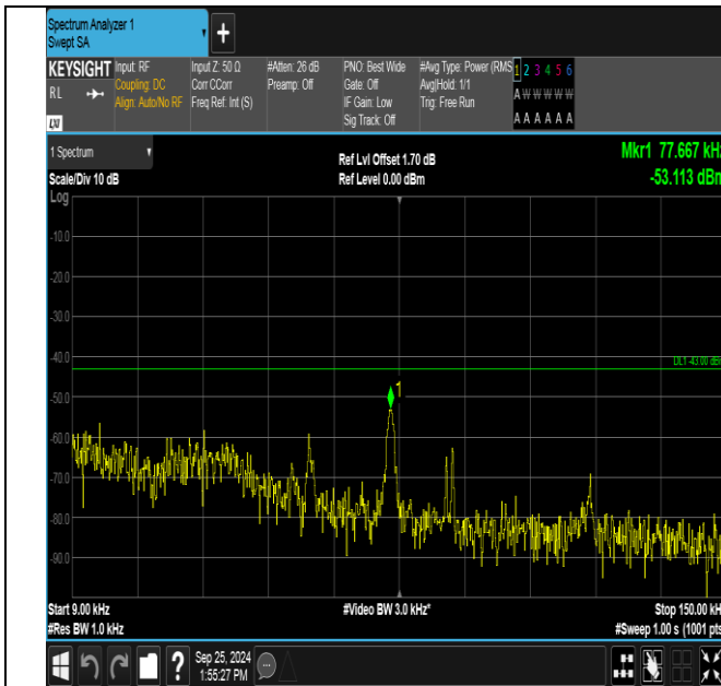
Band2-9538-0.009~0.15MHz-PASS
