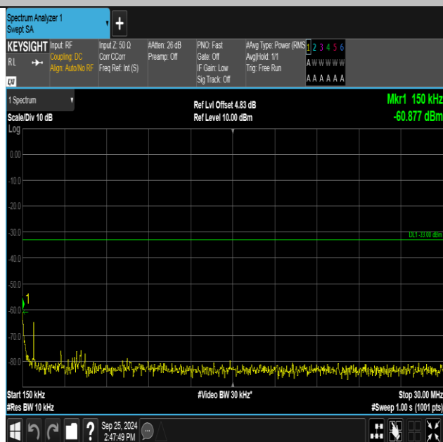
Band2-9400-3-0.15~30MHz-PASS
