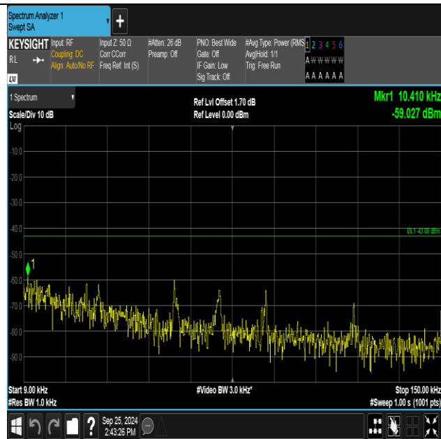
Band2-9400-1-0.009~0.15MHz-PASS
