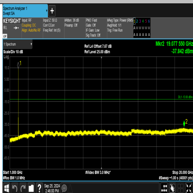
Band2-9400-2-1000~20000MHz-PASS
