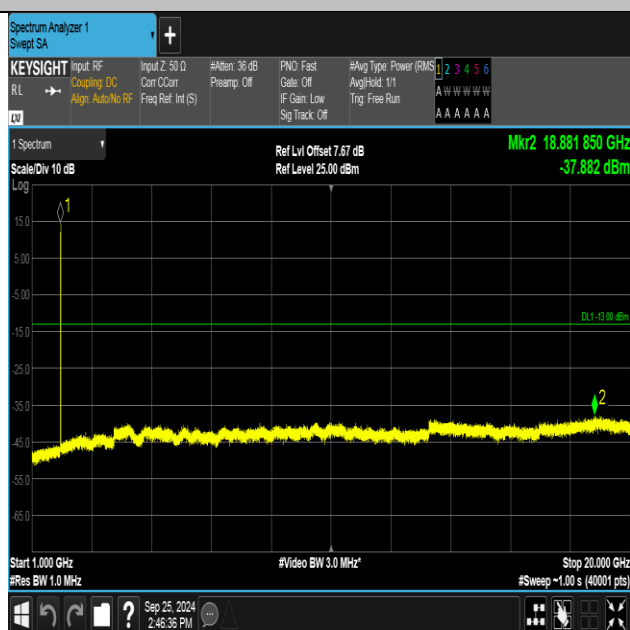
Band2-9538-2-1000~20000MHz-PASS
