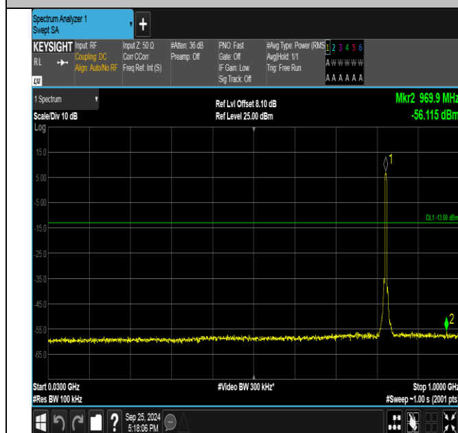
Band5-4132-30~1000MHz-PASS
