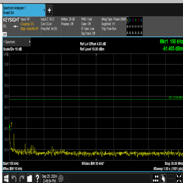
Band2-9400-4-0.15~30MHz-PASS
