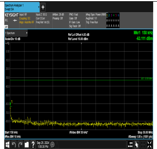
Band2-9538-0.15~30MHz-PASS
