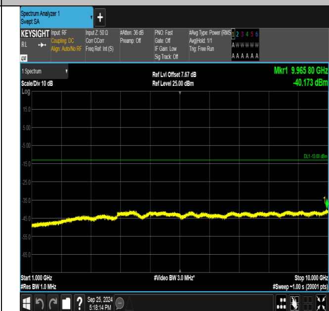
Band5-4132-1000~10000MHz-PASS
