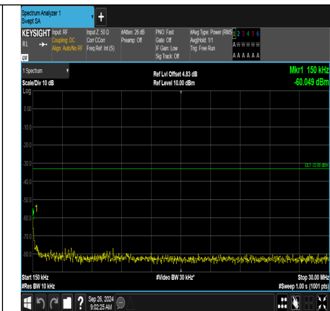
Band4-1413-0.15~30MHz-PASS
