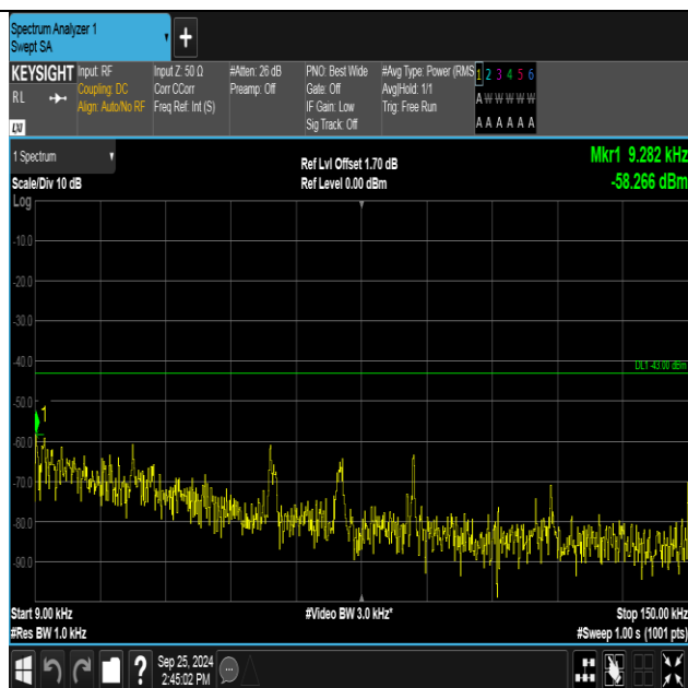
Band2-9262-2-0.009~0.15MHz-PASS
