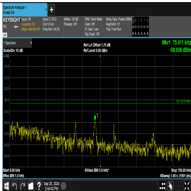
Band2-9538-1-0.009~0.15MHz-PASS
