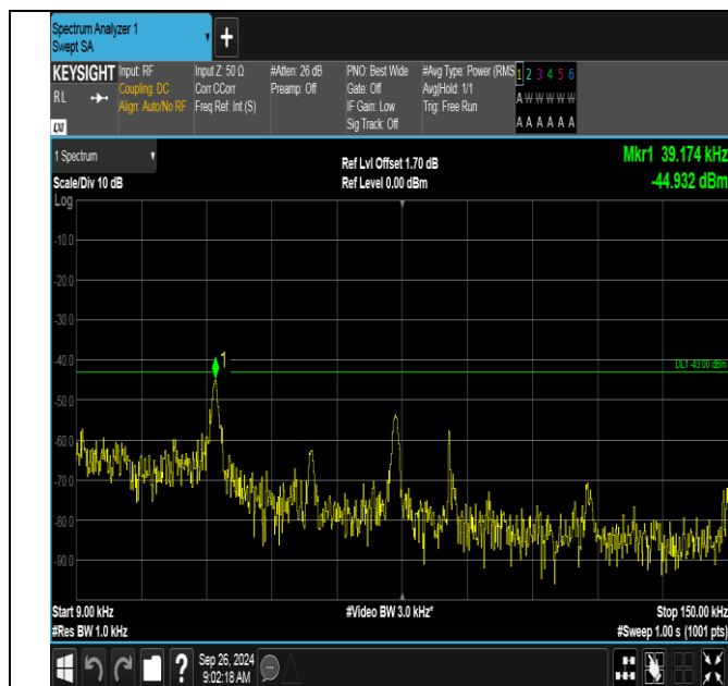
Band4-1413-0.009~0.15MHz-PASS
