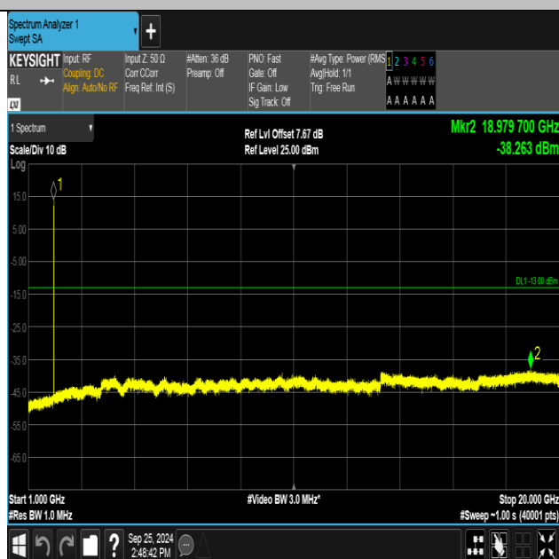
Band2-9538-3-1000~20000MHz-PASS
