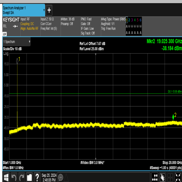
Band2-9400-3-1000~20000MHz-PASS
