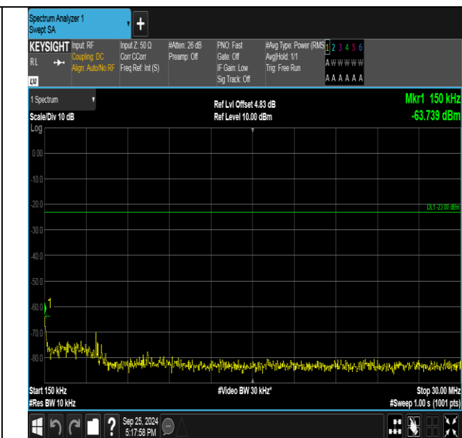
Band5-4132-0.15~30MHz-PASS
