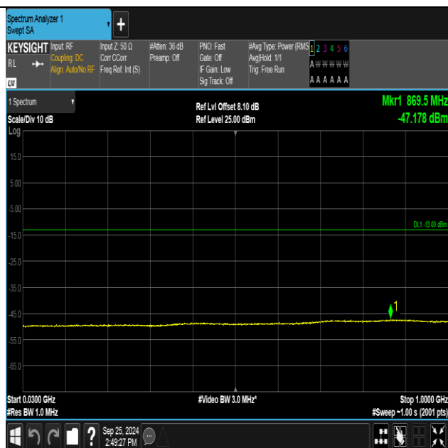
Band2-9262-4-30~1000MHz-PASS
