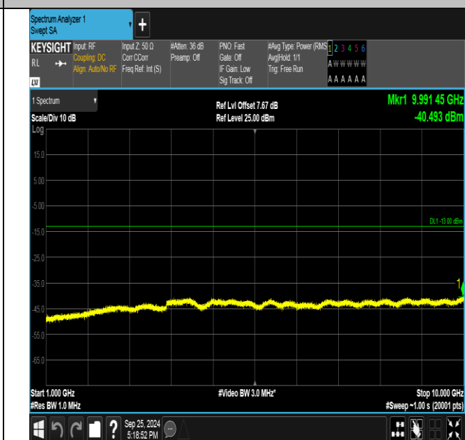
Band5-4182-1000~10000MHz-PASS
