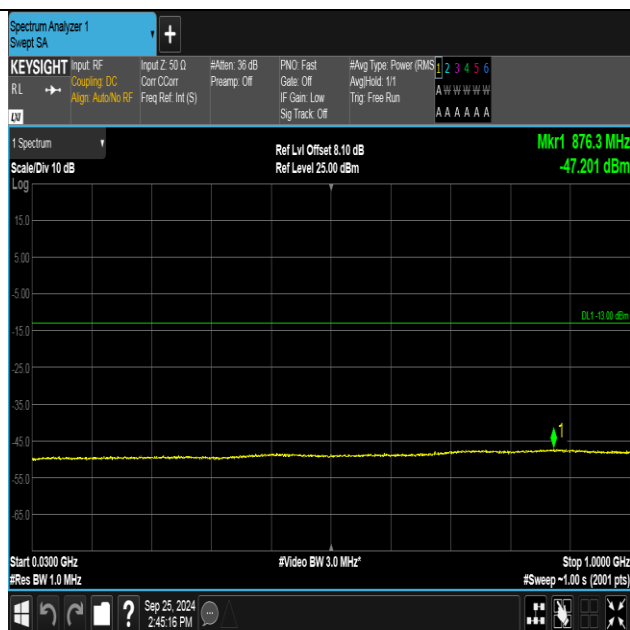
Band2-9262-2-30~1000MHz-PASS
