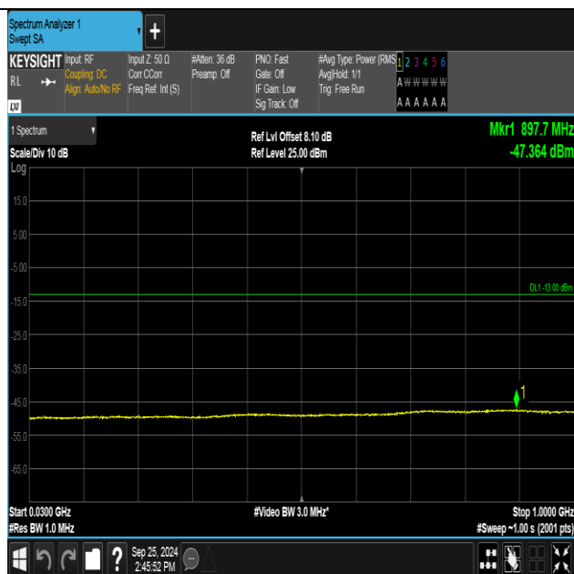
Band2-9400-2-30~1000MHz-PASS
