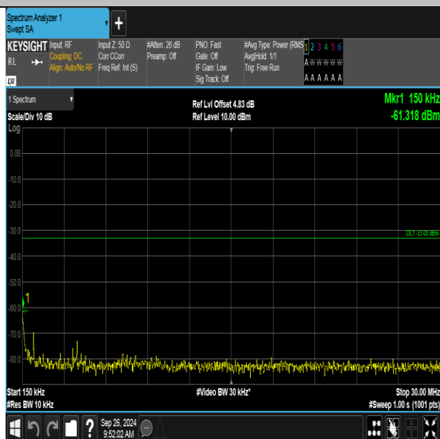
Band4-1413-4-0.15~30MHz-PASS
