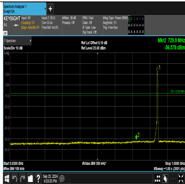
Band5-4233-1-30~1000MHz-PASS
