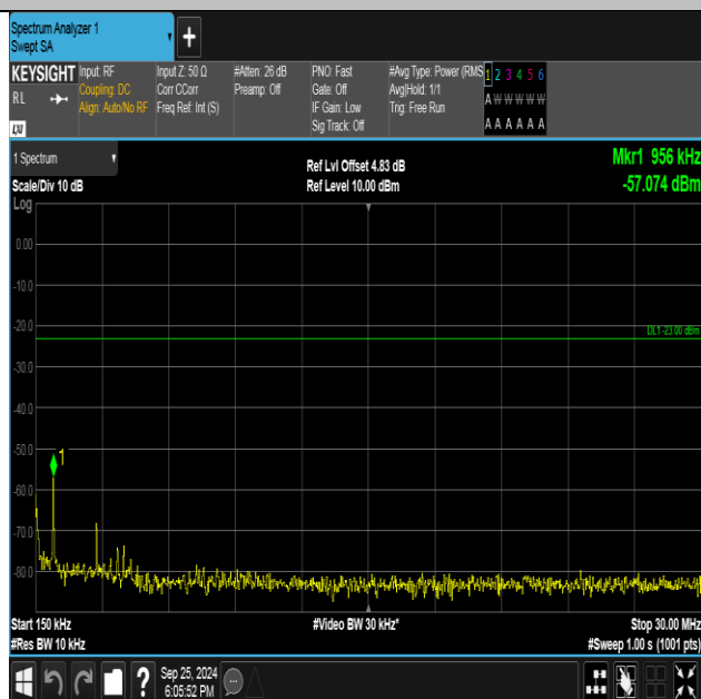
Band5-4132-3-0.15~30MHz-PASS
