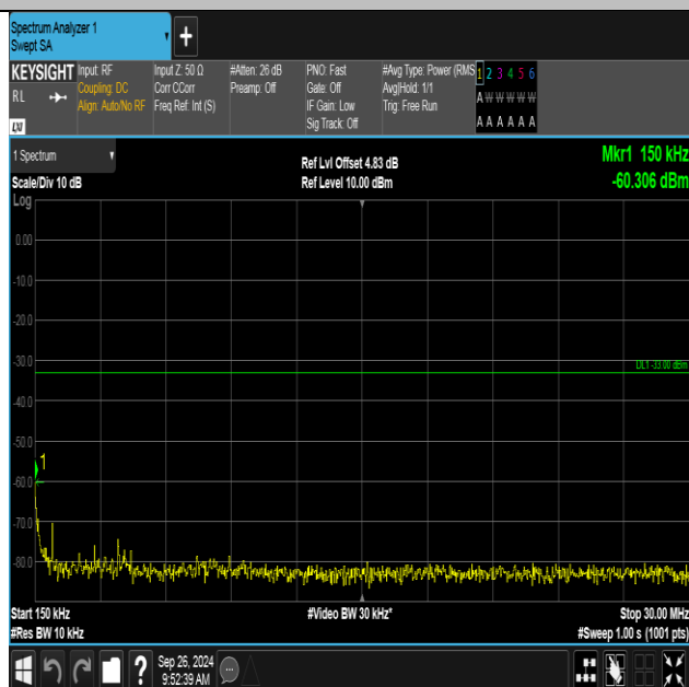
Band4-1513-4-0.15~30MHz-PASS
