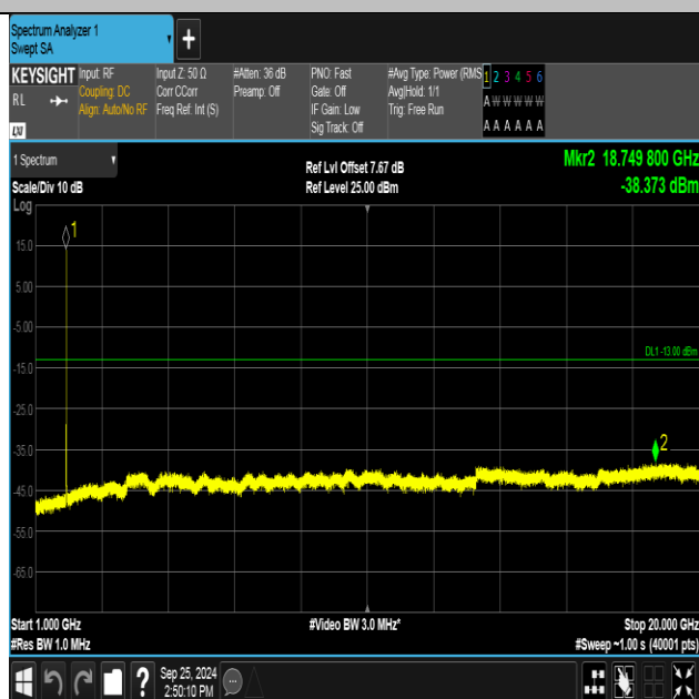
Band2-9400-4-1000~20000MHz-PASS
