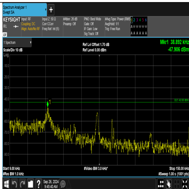
Band4-1413-1-0.009~0.15MHz-PASS
