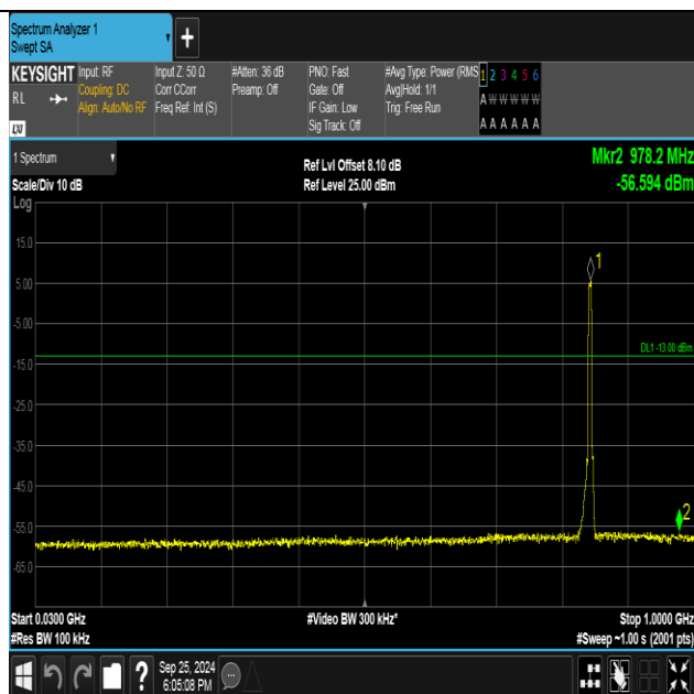
Band5-4233-2-30~1000MHz-PASS
