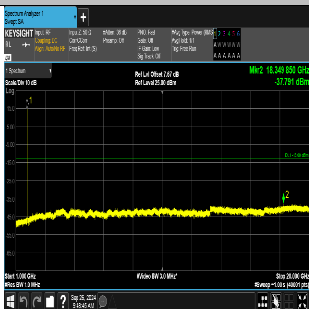
Band4-1513-2-1000~20000MHz-PASS
