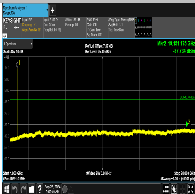
Band4-1513-3-1000~20000MHz-PASS
