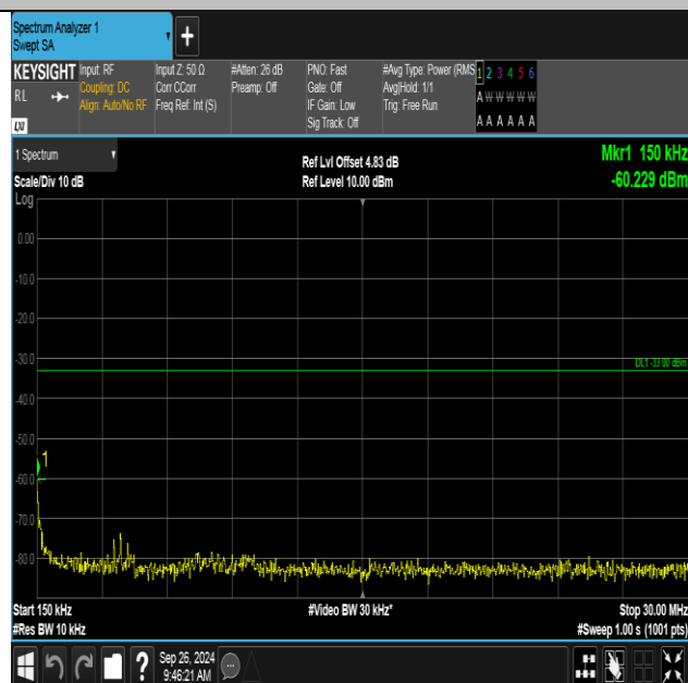
Band4-1513-1-0.15~30MHz-PASS
