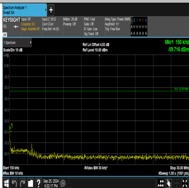
Band5-4182-1-0.15~30MHz-PASS
