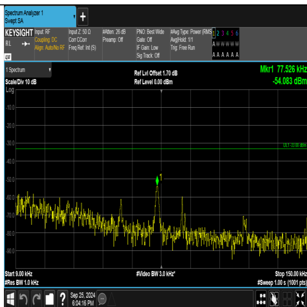
Band5-4182-2-0.009~0.15MHz-PASS
