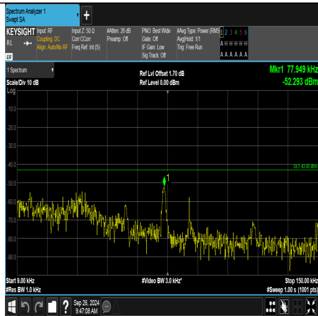
Band4-1312-2-0.009~0.15MHz-PASS
