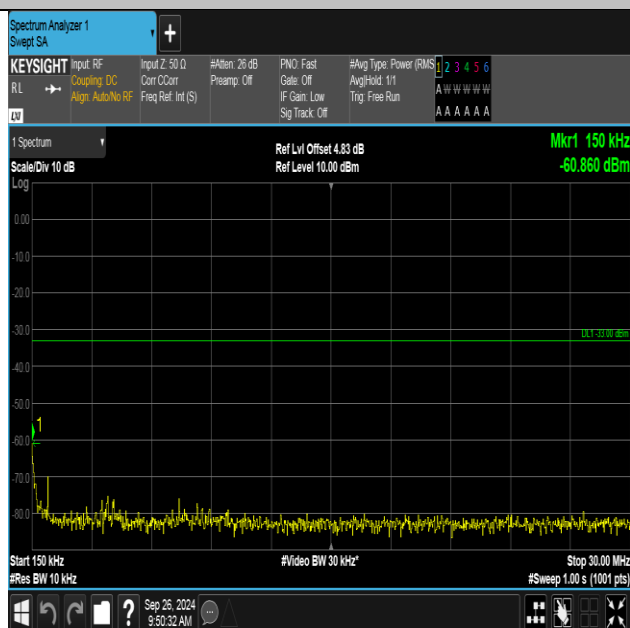
Band4-1513-3-0.15~30MHz-PASS
