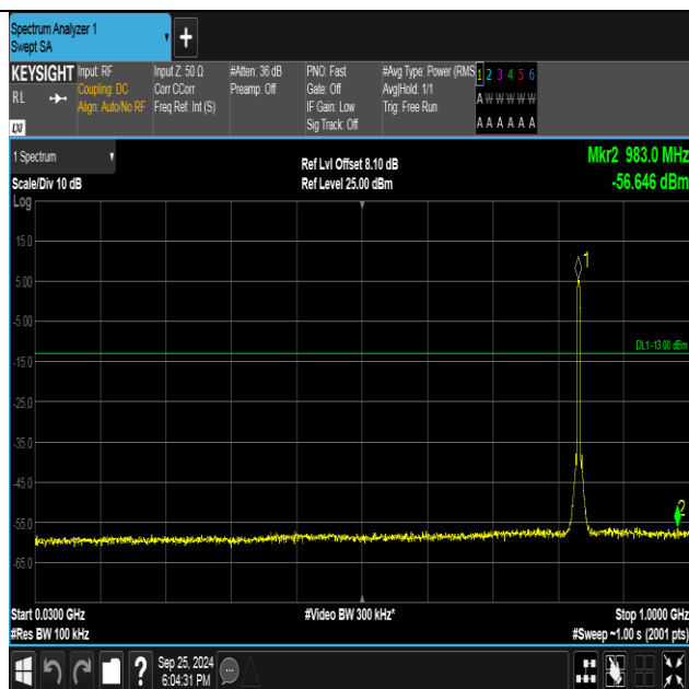
Band5-4182-2-30~1000MHz-PASS
