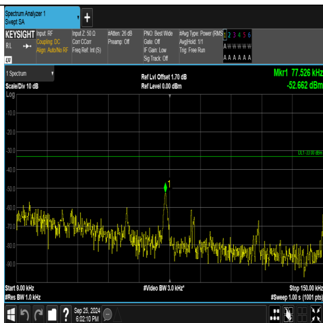
Band5-4182-1-0.009~0.15MHz-PASS
