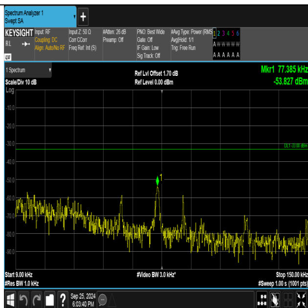
Band5-4132-2-0.009~0.15MHz-PASS
