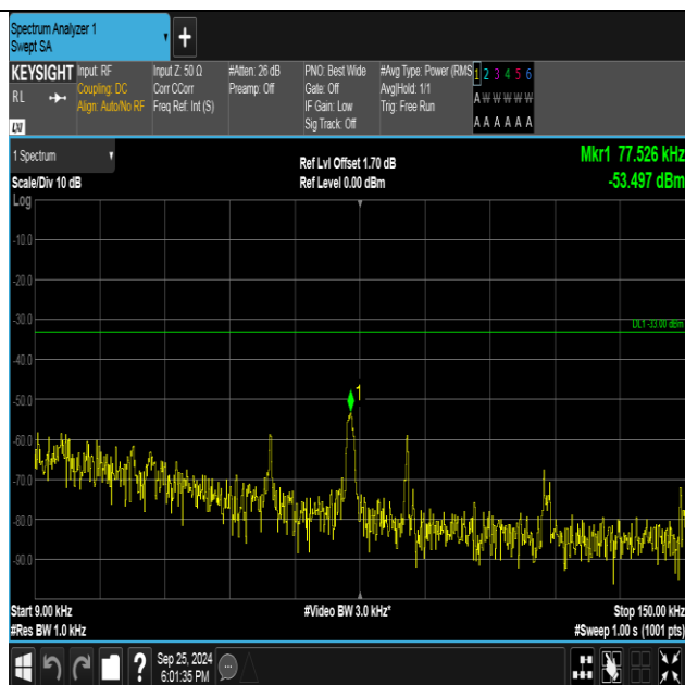
Band5-4132-1-0.009~0.15MHz-PASS
