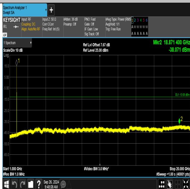
Band4-1413-2-1000~20000MHz-PASS
