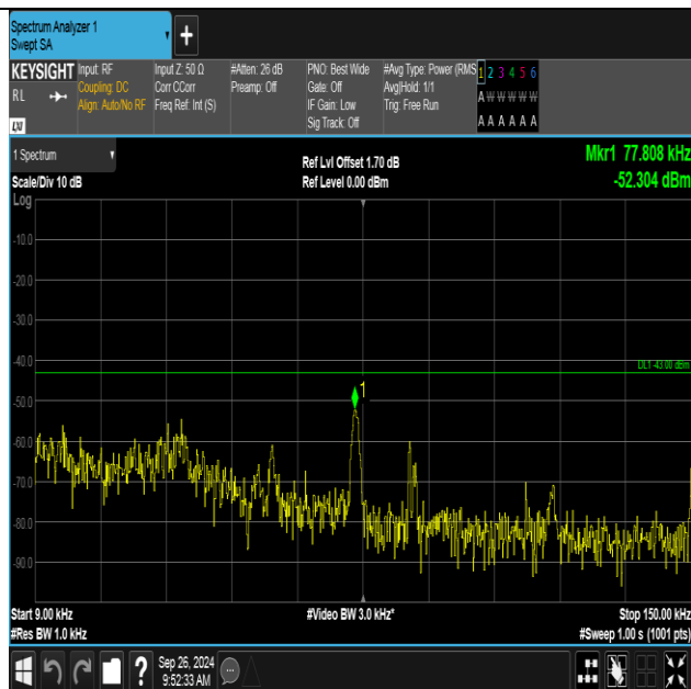
Band4-1513-4-0.009~0.15MHz-PASS
