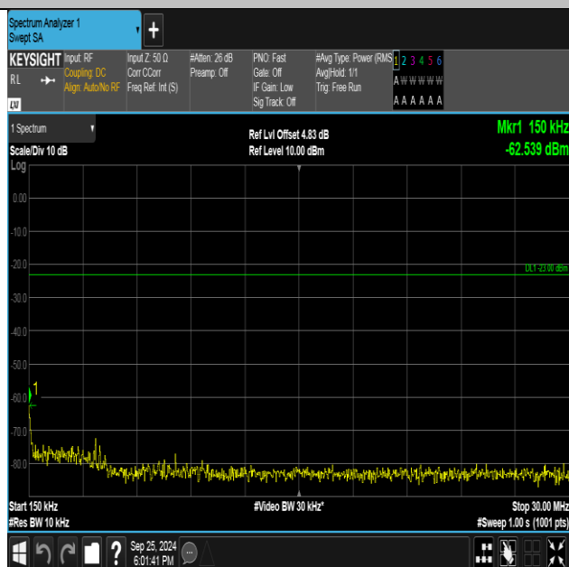
Band5-4132-1-0.15~30MHz-PASS
