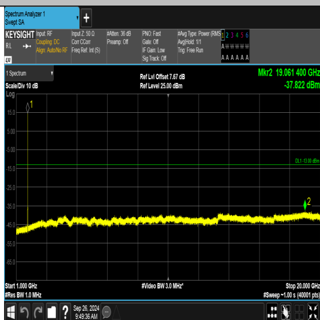
Band4-1312-3-1000~20000MHz-PASS
