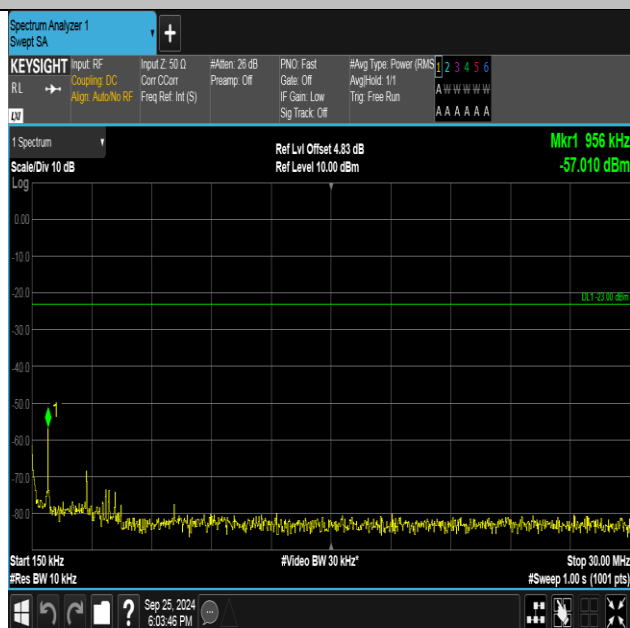
Band5-4132-2-0.15~30MHz-PASS
