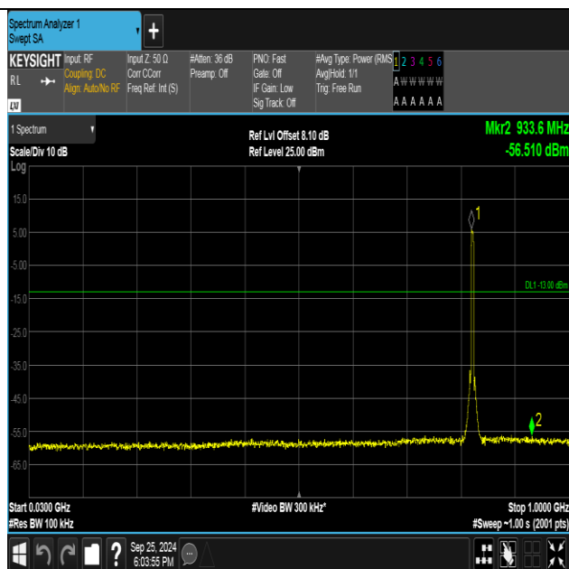
Band5-4132-2-30~1000MHz-PASS
