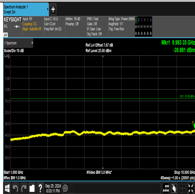
Band5-4233-1-1000~10000MHz-PASS
