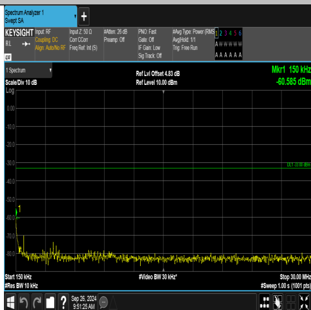
Band4-1312-4-0.15~30MHz-PASS
