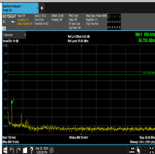
Band5-4233-2-0.15~30MHz-PASS
