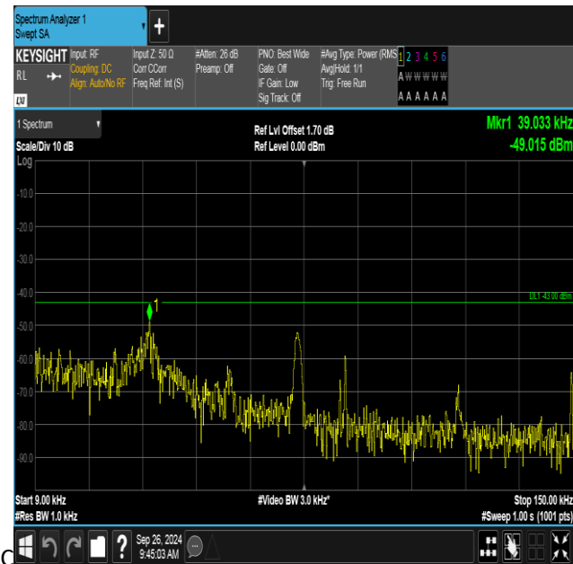
Band4-1312-1-0.009~0.15MHz-PASS
