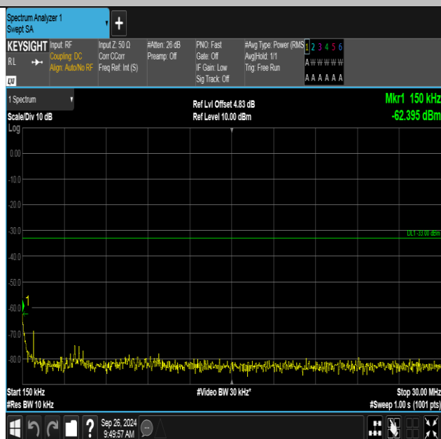
Band4-1413-3-0.15~30MHz-PASS
