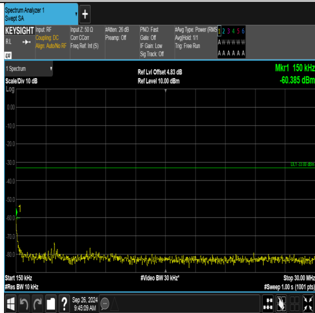
Band4-1312-1-0.15~30MHz-PASS
