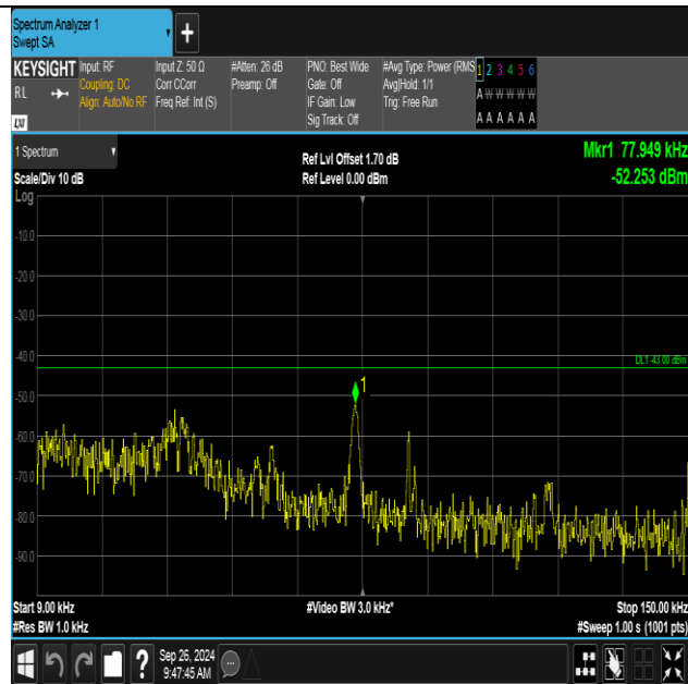
Band4-1413-2-0.009~0.15MHz-PASS
