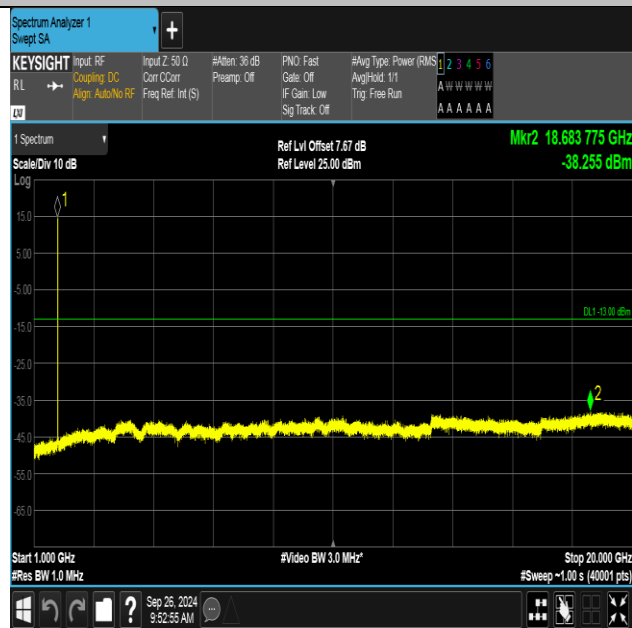
Band4-1513-4-1000~20000MHz-PASS
