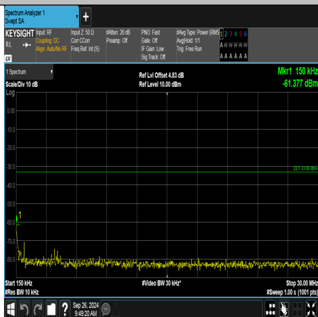
Band4-1312-3-0.15~30MHz-PASS
