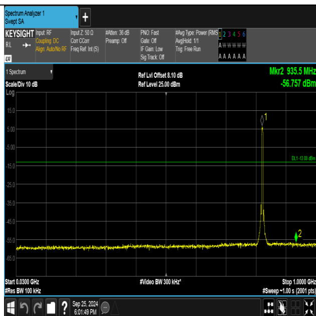
Band5-4132-1-30~1000MHz-PASS
