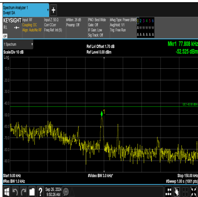
Band4-1513-3-0.009~0.15MHz-PASS
