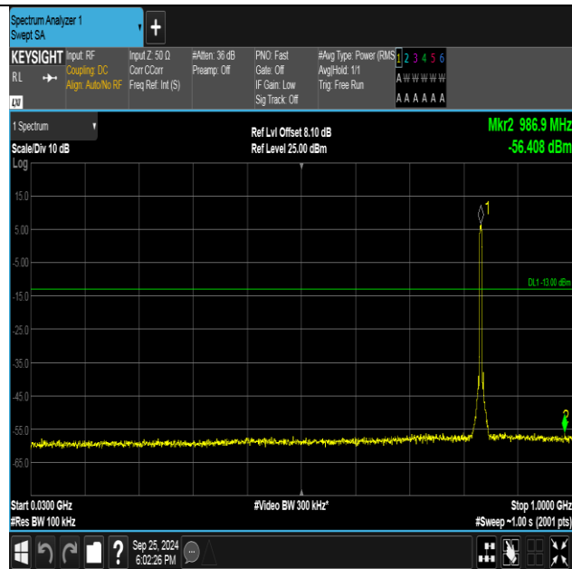
Band5-4182-1-30~1000MHz-PASS
