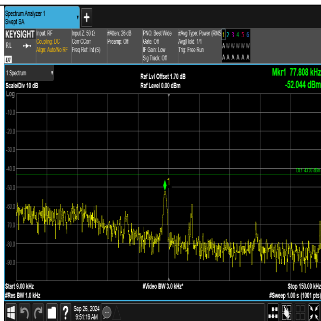
Band4-1312-4-0.009~0.15MHz-PASS
