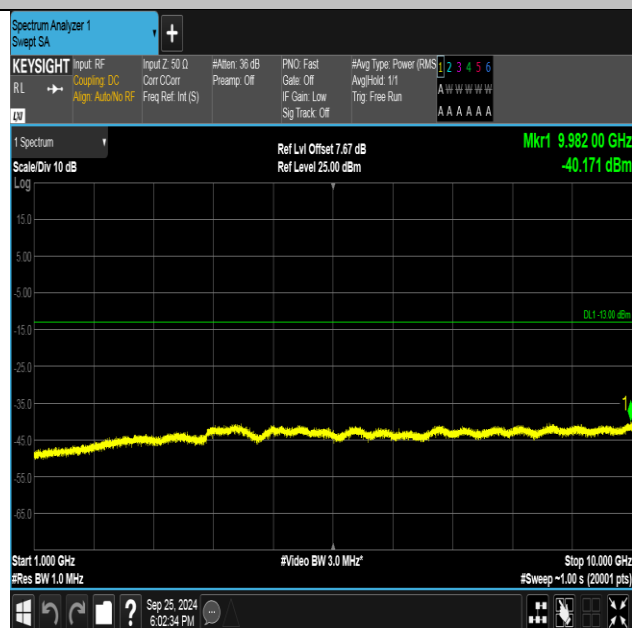
Band5-4182-1-1000~10000MHz-PASS
