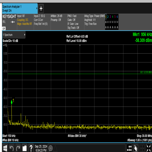
Band5-4182-2-0.15~30MHz-PASS
