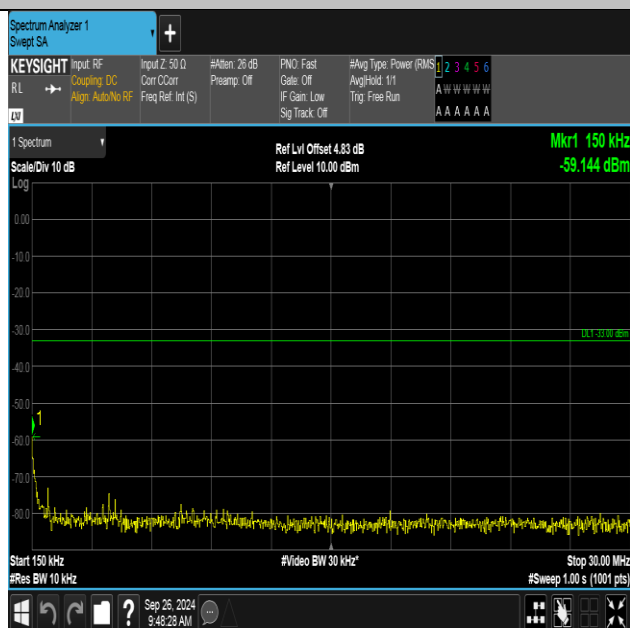
Band4-1513-2-0.15~30MHz-PASS
