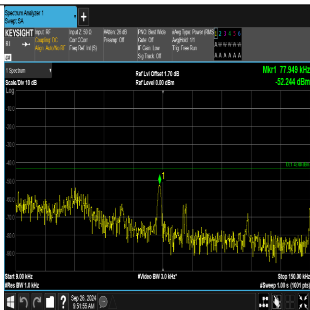
Band4-1413-4-0.009~0.15MHz-PASS
