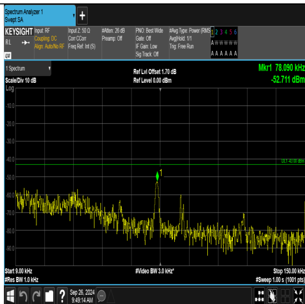
Band4-1312-3-0.009~0.15MHz-PASS
