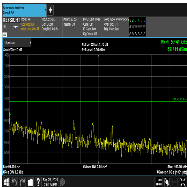
Band2-9538-4-0.009-0.15MHz-PASS
