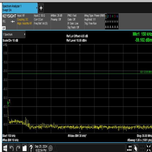
Band5-4233-1-0.15~30MHz-PASS
