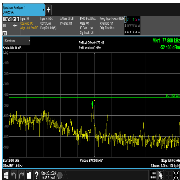
Band4-1413-3-0.009~0.15MHz-PASS
