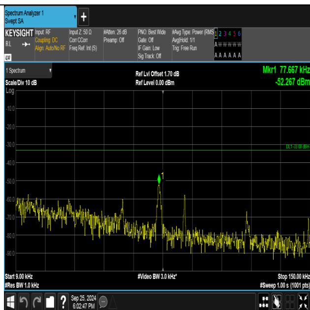
Band5-4233-1-0.009~0.15MHz-PASS
