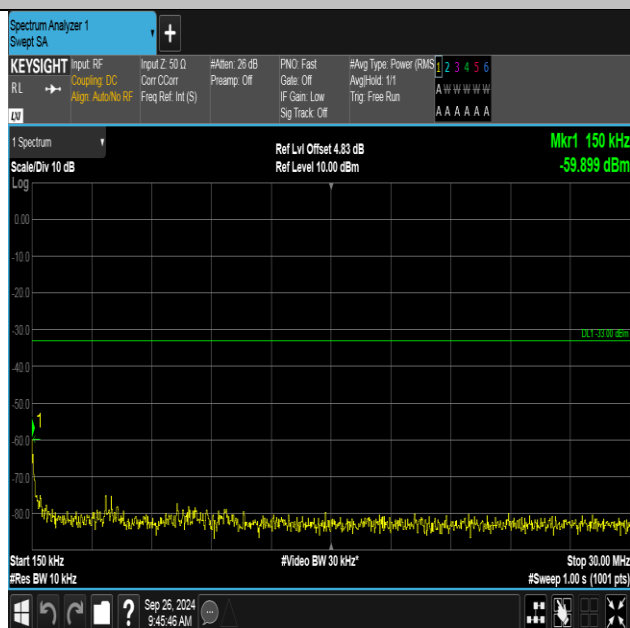
Band4-1413-1-0.15~30MHz-PASS
