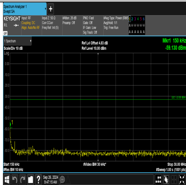
Band4-1312-2-0.15~30MHz-PASS
