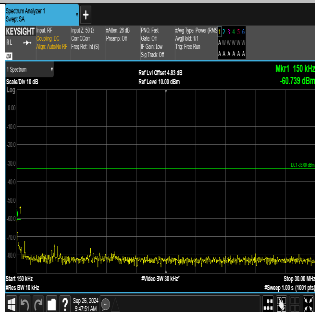
Band4-1413-2-0.15~30MHz-PASS
