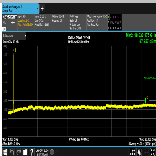
Band4-1312-2-1000~20000MHz-PASS
