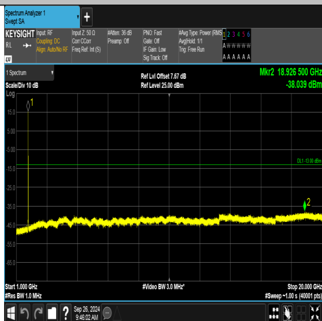
Band4-1413-1-1000~20000MHz-PASS
