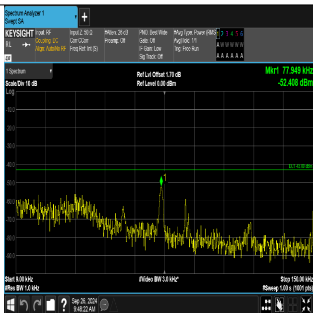
Band4-1513-2-0.009~0.15MHz-PASS
