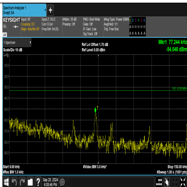
Band5-4132-3-0.009~0.15MHz-PASS
