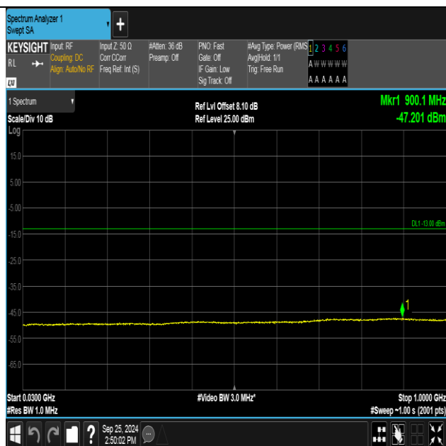
Band2-9400-4-30~1000MHz-PASS
