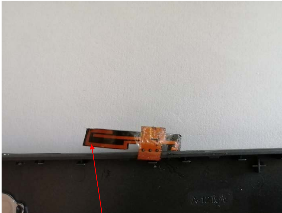
WIFI Antenna / BT antenna
