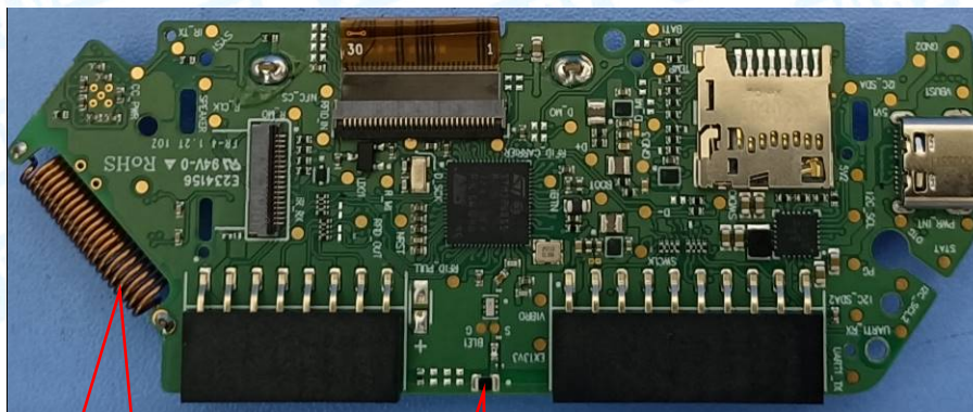
Photo 13 Appearance of PCB
