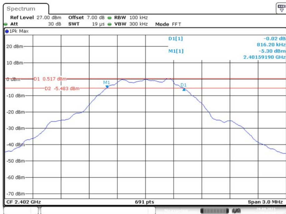
6dB Bandwidth, BLE Low Channel
