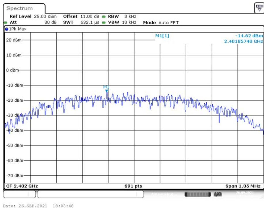
Power Spectral Density, BLE Low Channel
