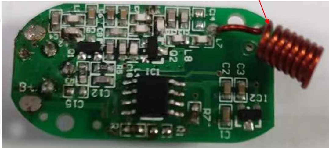
Name: Enameled antenna, model: RW01 433MHZ (CKHL3.2*7.5TS*0.8-P)
