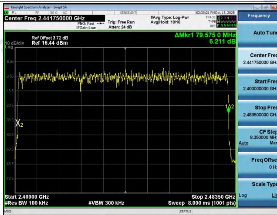
Number_of_Hopping_Channel_(Hopping)_NVNT_ANT1_2-DH5_Hopping
