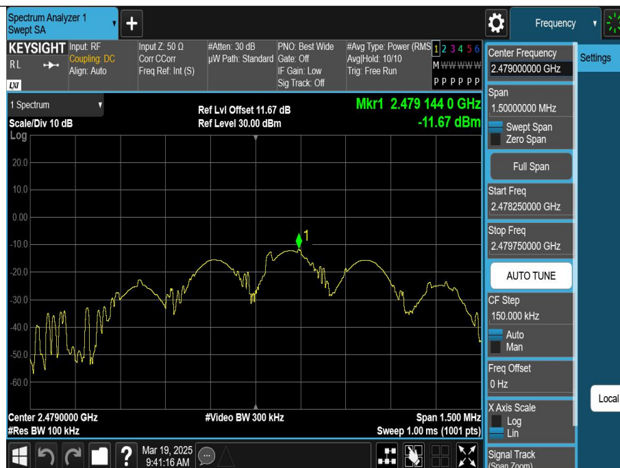
DH5-Ant1-2479-0~Reference-PASS
