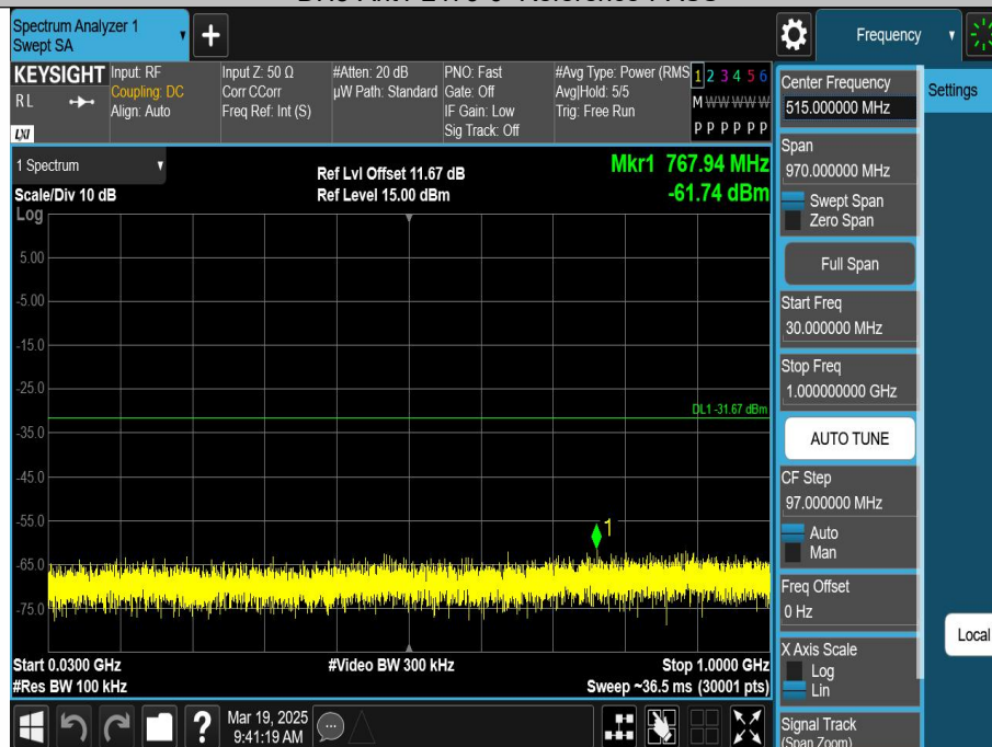
DH5-Ant1-2479-30~1000-PASS
