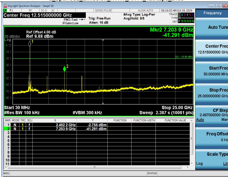
2_Spurious_Emission_NVNT_ANT1_125kbps_2402
