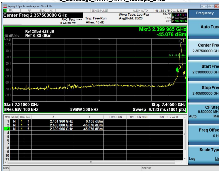
2_Bandedge_NVNT_ANT1_125kbps_2402
