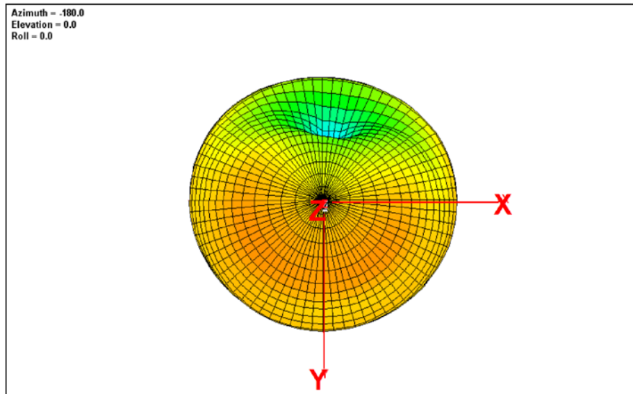
3D Radiation Pattern @ 2440 MHz
