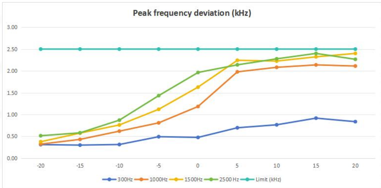
Peak frequency deviation chart
