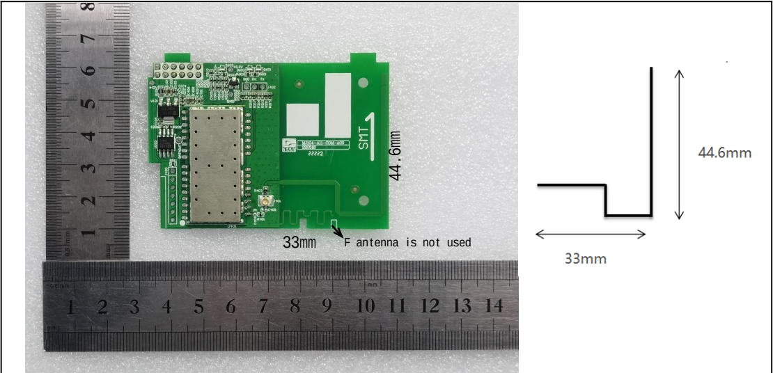
Antenna Top View [With Ruler]
