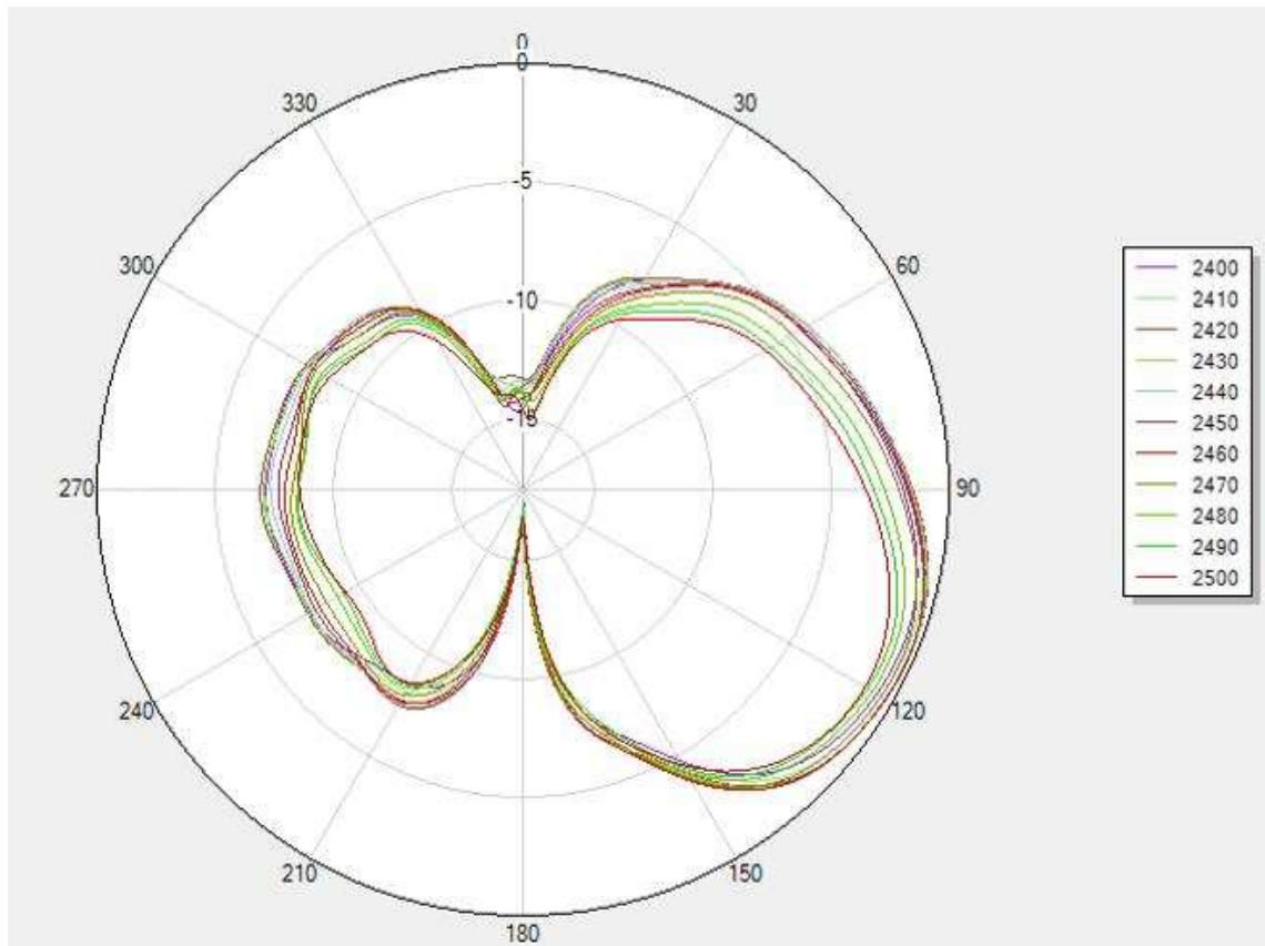
Phi 90 2D
