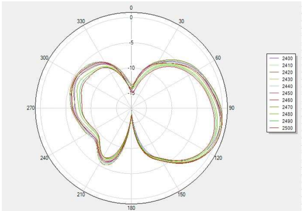
Theta 90 2D
